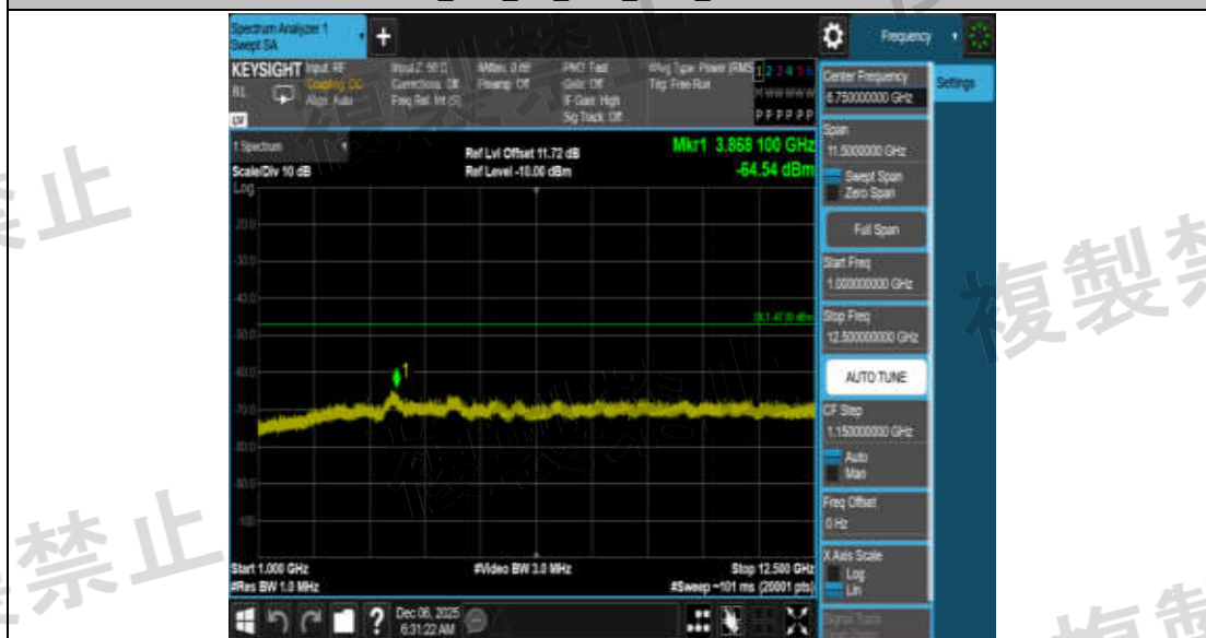
NTNV_BLE_2M_Ant1_2440_1000~12500
