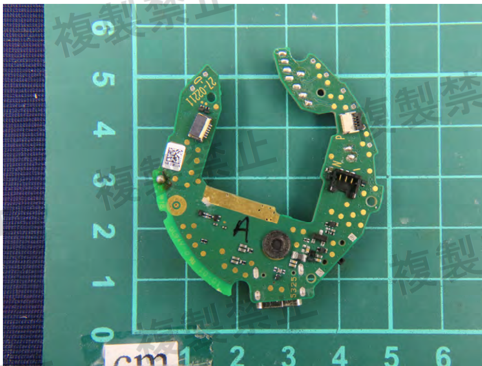
(35) EUT Photo
