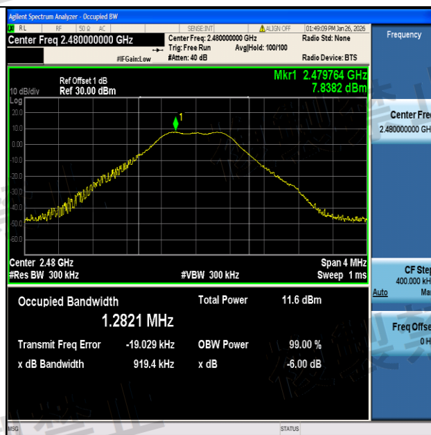
NTNV-BLE_1M-Ant1-2480-PASS
