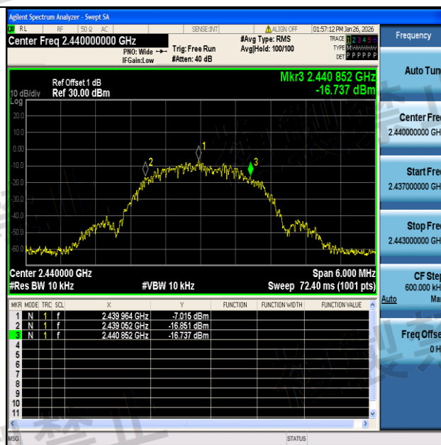
NTNV-BLE_2M-Ant1-2440-PASS
