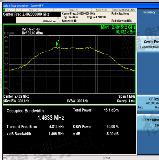
NTNV-BLE_2M-Ant1-2402-PASS
