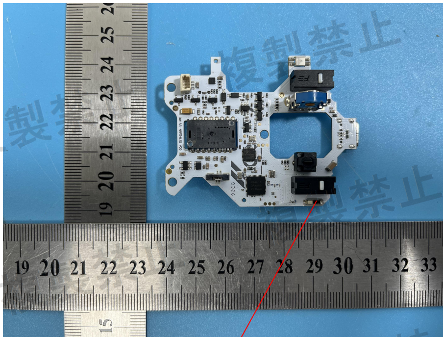
Antenna location
