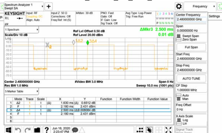
載波頻率週期_8DPSK_3M_DH3_2480MHz
