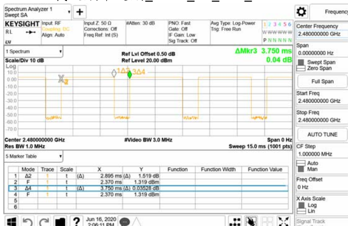
載波頻率週期_GFSK_1M_DH5_2480MHz
