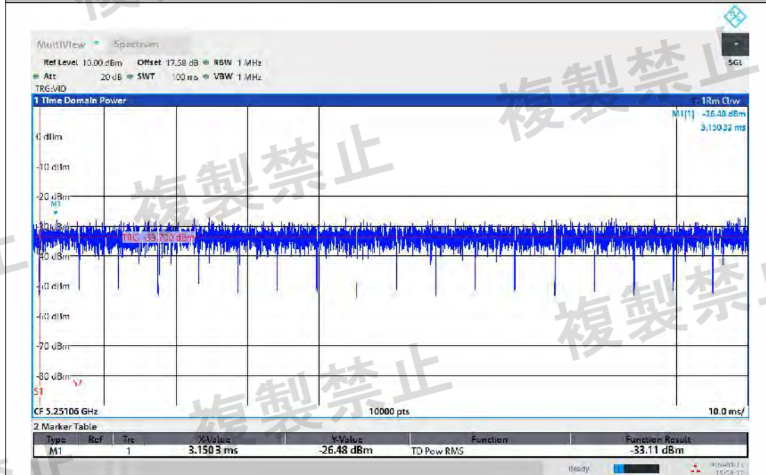
NTNV-11AC20MIMO-Ant1-5240-5251~5260-PASS
