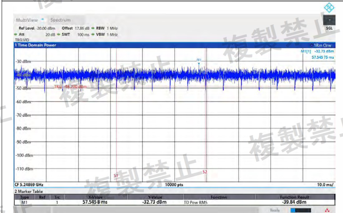
NTNV-11AX80MIMO-Ant2-5290-5210~5249-PASS
