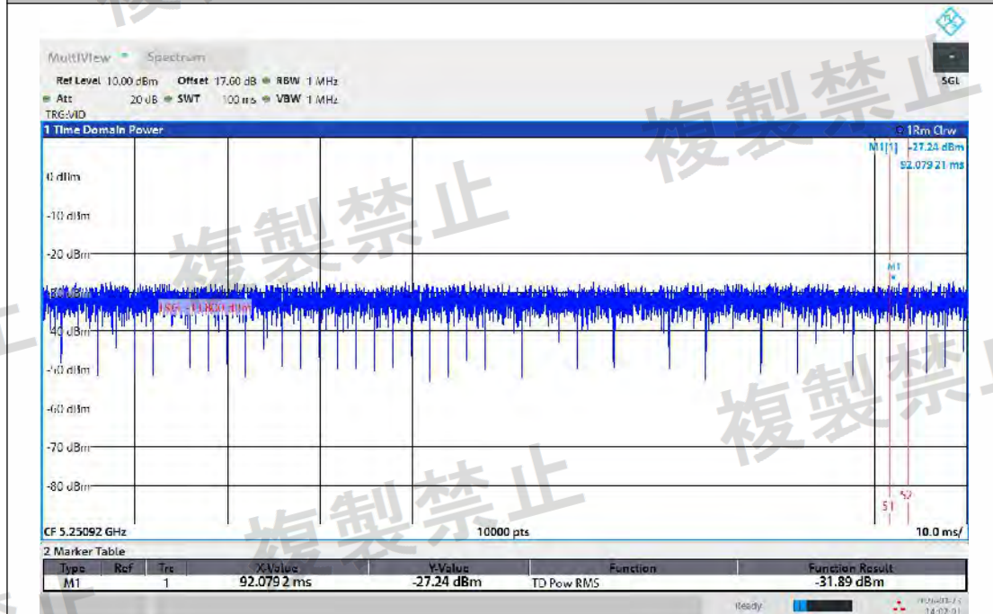
NTNV-11A-Ant2-5240-5250~5251-PASS
