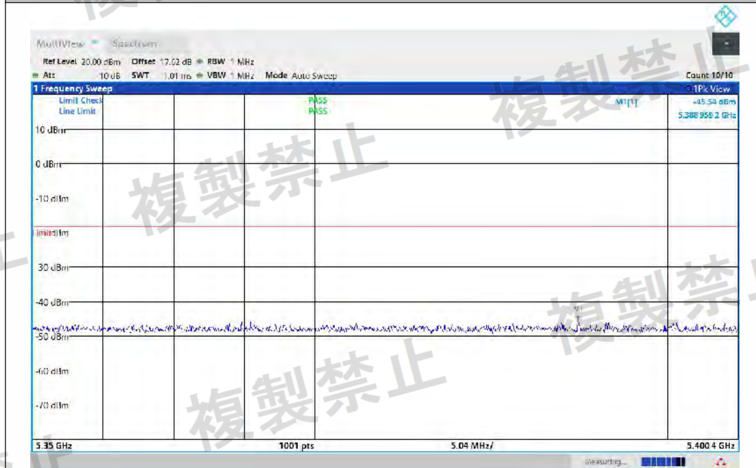
NTNV-11BE160MIMO-Ant1-5250-5350~5400.4-PASS
