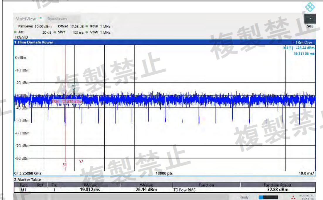
NTNV-11AC20MIMO-Ant1-5240-5250.2~5251-PASS
