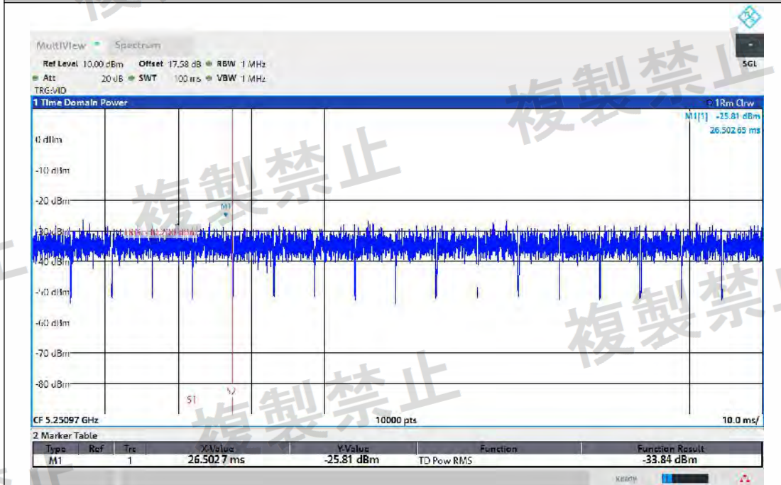
NTNV-11AX20MIMO-Ant1-5240-5250.2~5251-PASS
