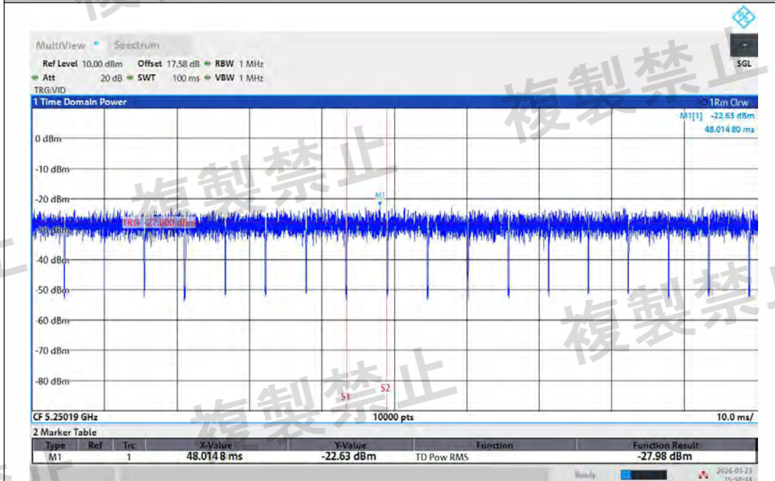
NTNV-11AC20MIMO-Ant2-5240-5250~5250.2-PASS
