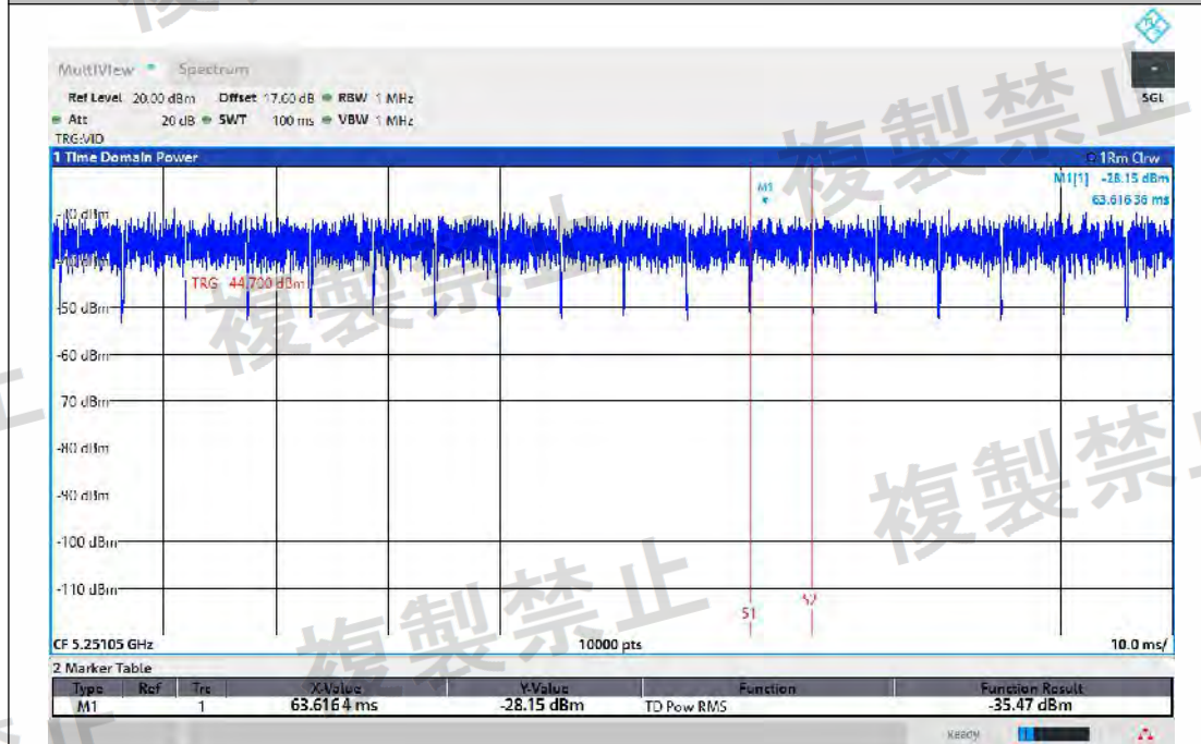
NTNV-11AX20MIMO-Ant1-5240-5251~5260-PASS
