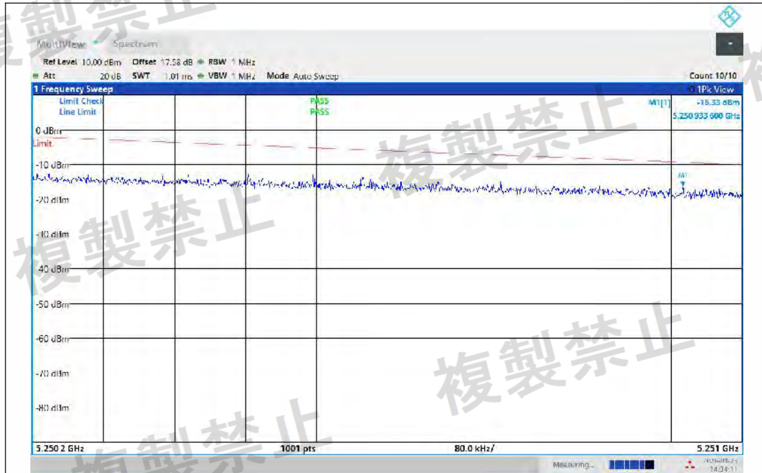
NTNV-11N20MIMO-Ant1-5240-5250.2~5251-PASS
