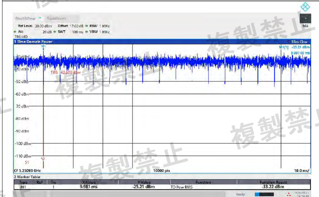
NTNV-11N20MIMO-Ant1-5240-5250.2~5251-PASS
