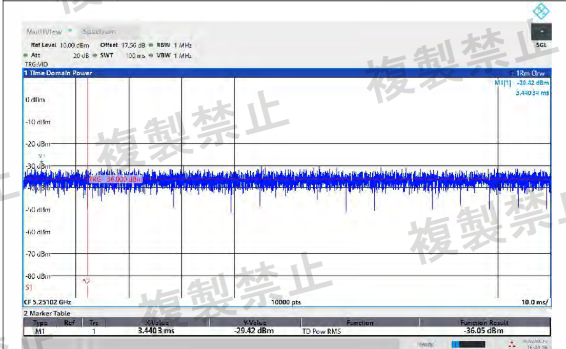
NTNV-11AC40MIMO-Ant2-5230-5251~5270-PASS
