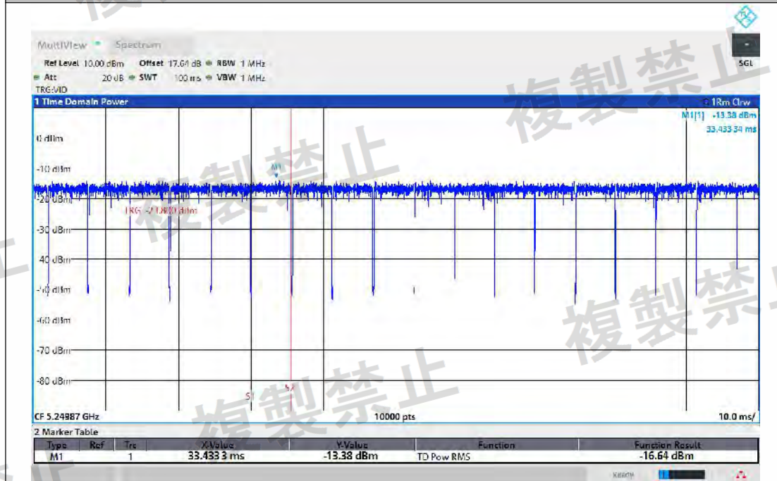
NTNV-11BE20MIMO-Ant2-5260-5249.8~5250-PASS
