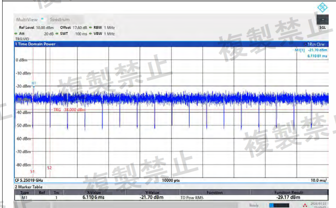
NTNV-11AC20MIMO-Ant2-5240-5250~5250.2-PASS
