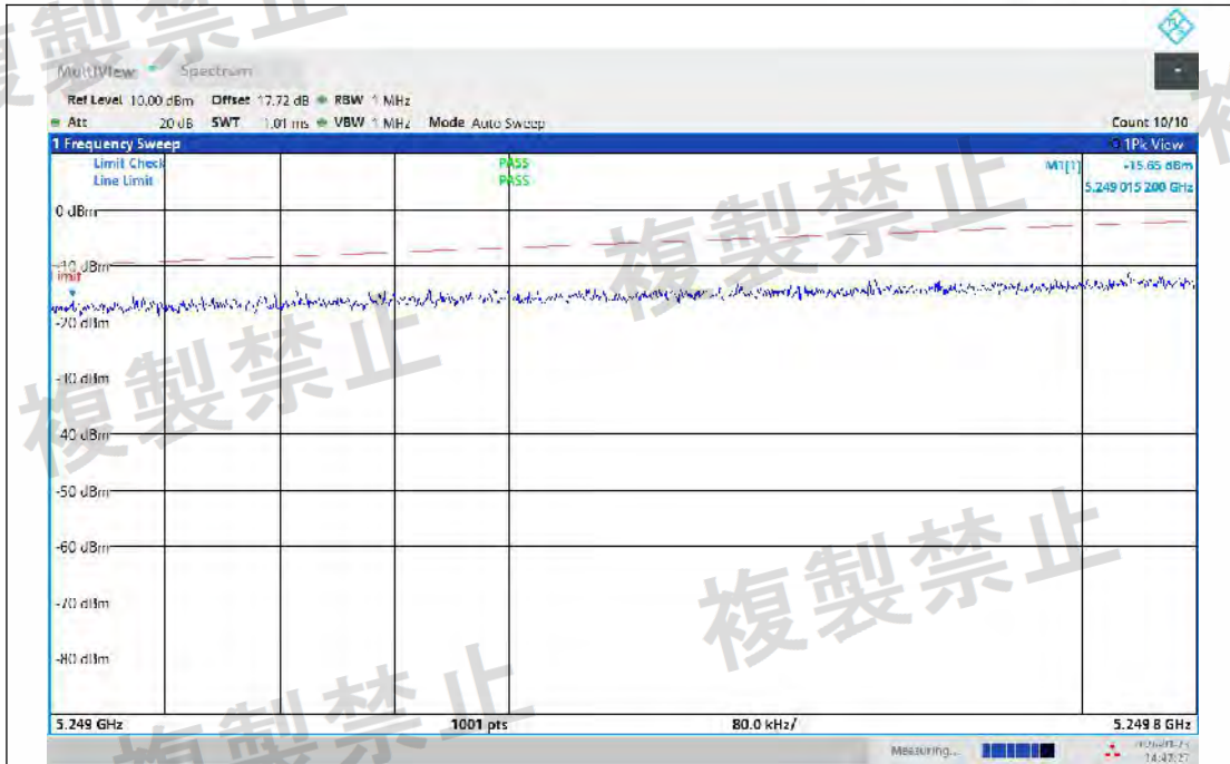
NTNV-11N20MIMO-Ant2-5260-5249~5249.8-PASS
