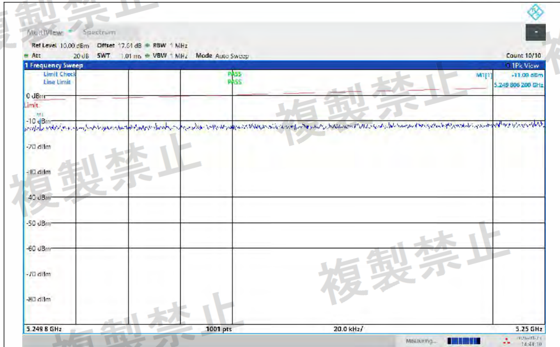
NTNV-11N20MIMO-Ant1-5260-5249.8~5250-PASS
