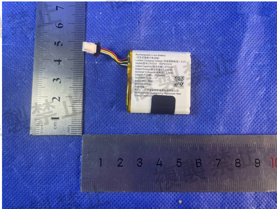
Figure 19: Battery view
