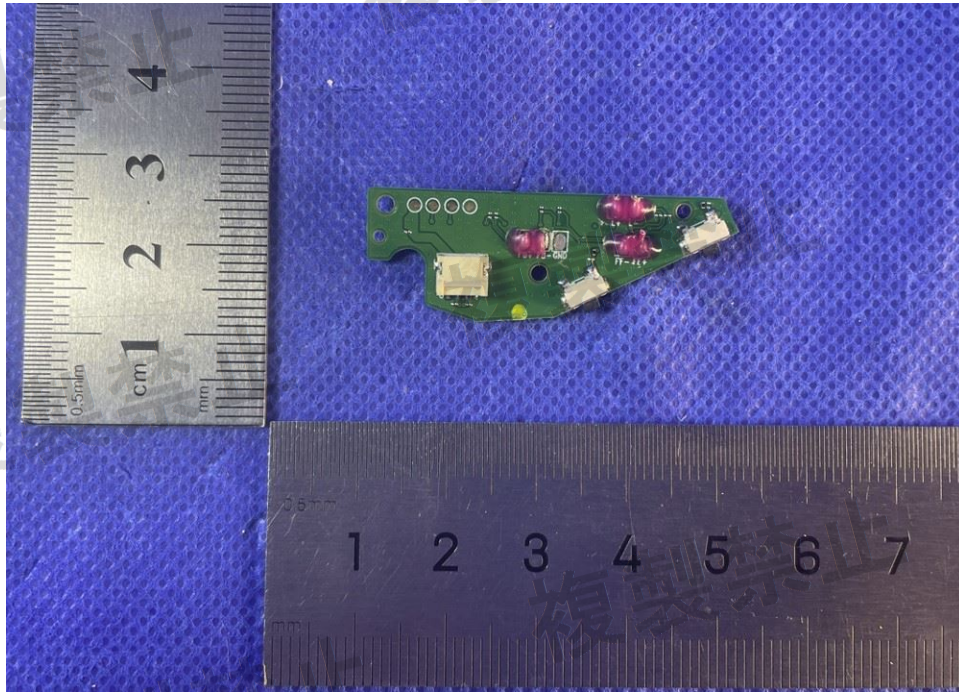
Figure 17: Top view of main board 2
