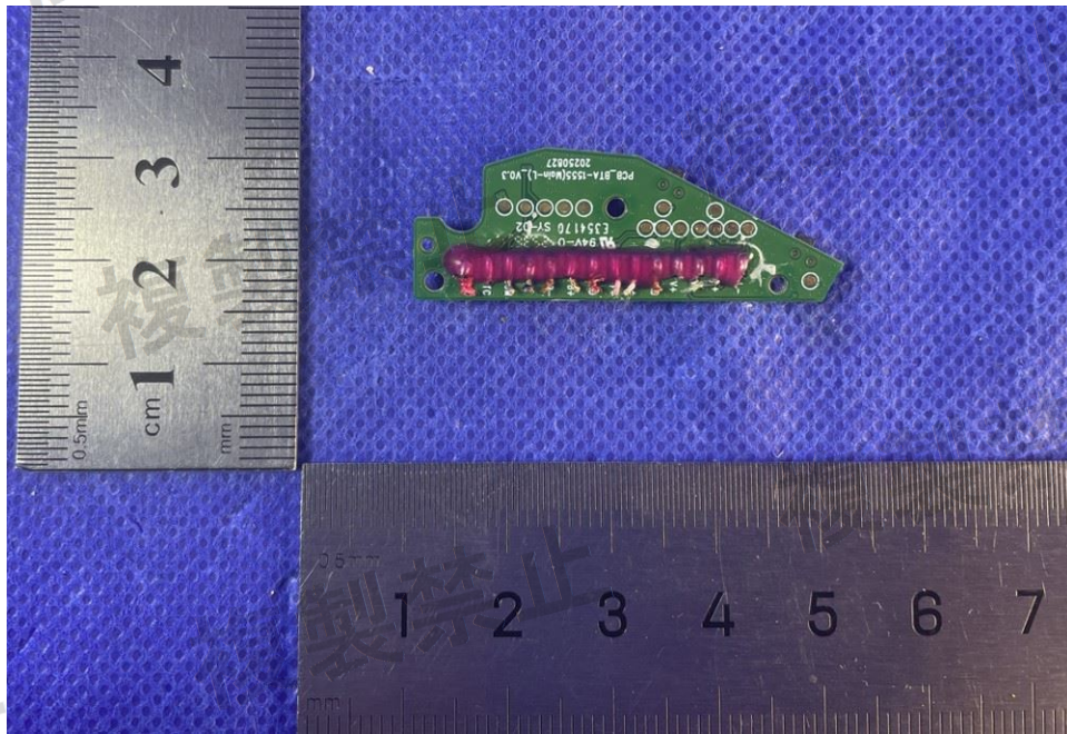
Figure 18: Bottom view of main board 2
