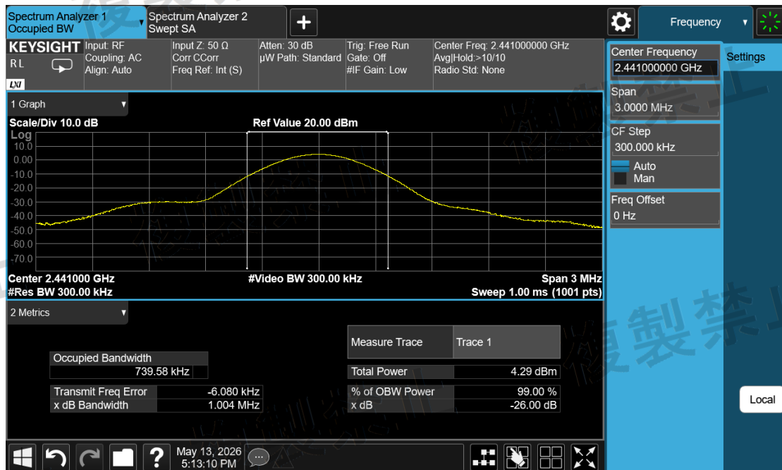
Channel Sounding_Mode 2\Occupied Bandwidth\2441-ANT2-N
