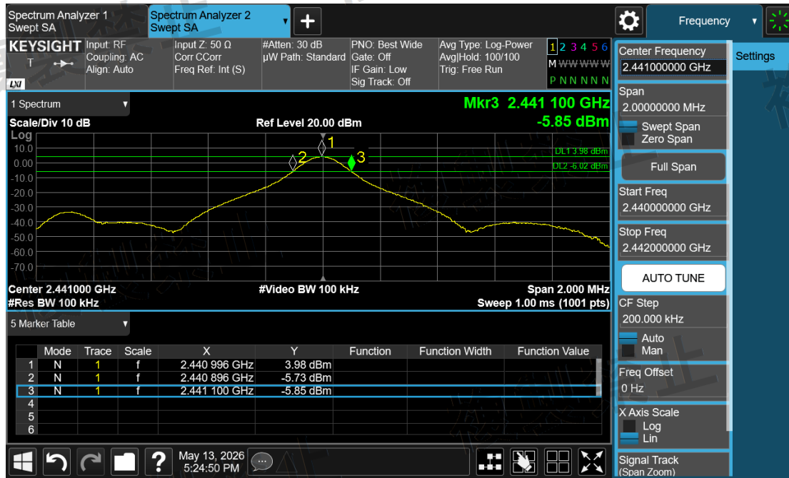
Channel Sounding_Mode 2\Frequency Error\2441-ANT2-N
