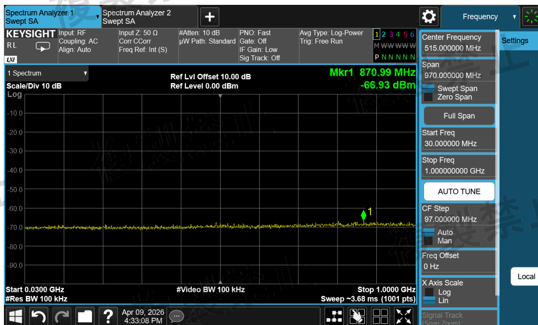
Channel Sounding_Mode 0\Secondarily Emitted Radio Wave Strength\30M~1000M-2404-ANT1-N
