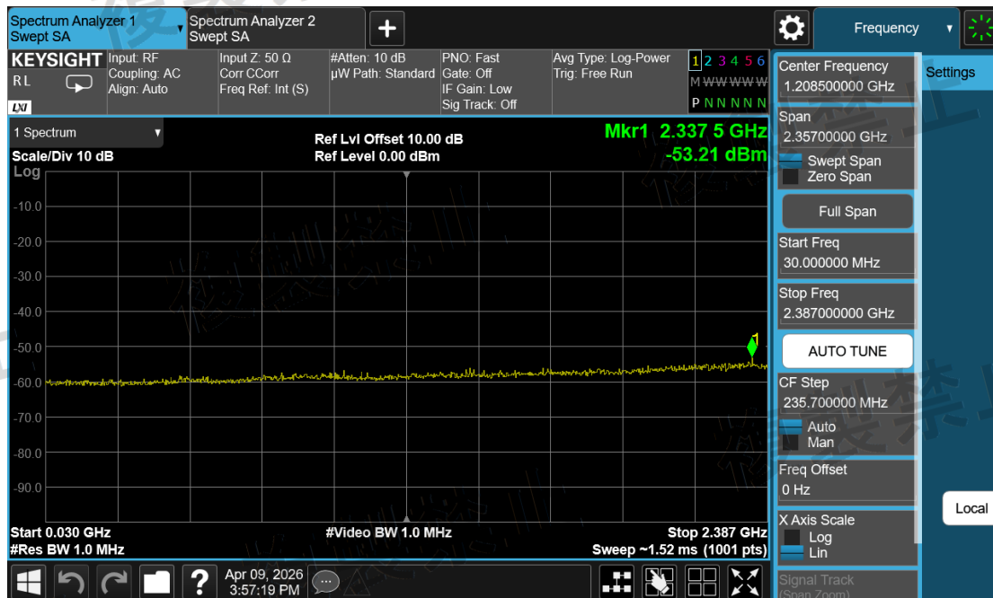
Channel Sounding_Mode 0\Unwanted Emission Strength\30M~2387M-2404-ANT1-N
