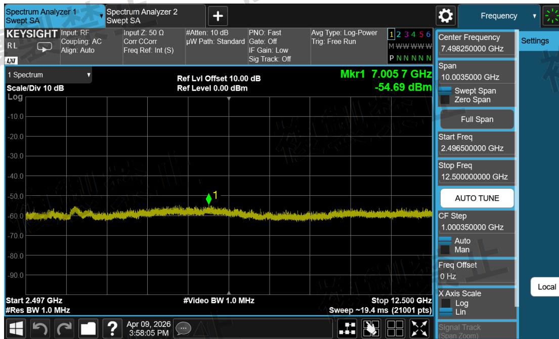
Channel Sounding_Mode 0\Unwanted Emission Strength\2496.5M~12500M-2404-ANT1-N
