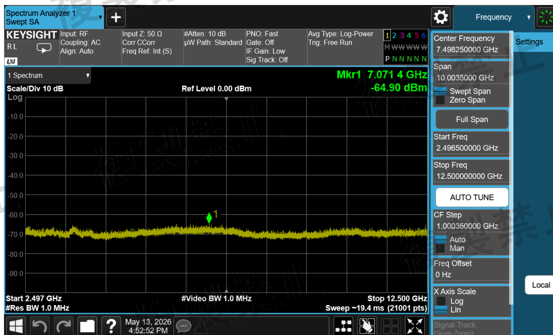
Channel Sounding_Mode 2\Unwanted Emission Strength\2496.50~12500.00-2404-ANT2-N
