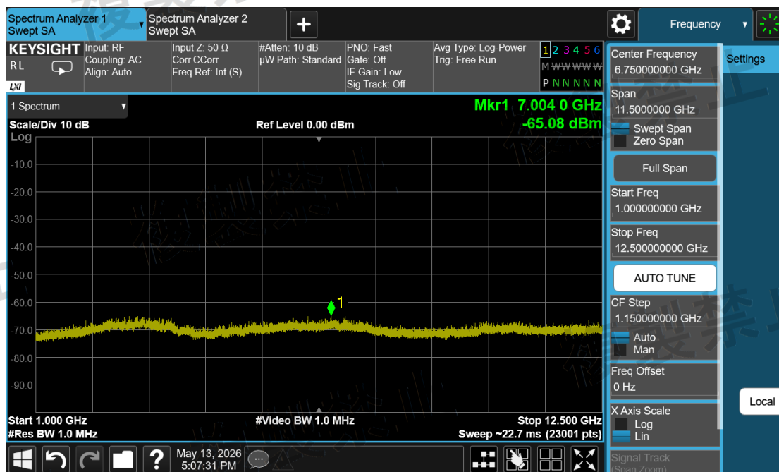
Channel Sounding_Mode 2\Secondarily Emitted Radio Wave Strength\1000.00~12500.00-2404-ANT2-N
