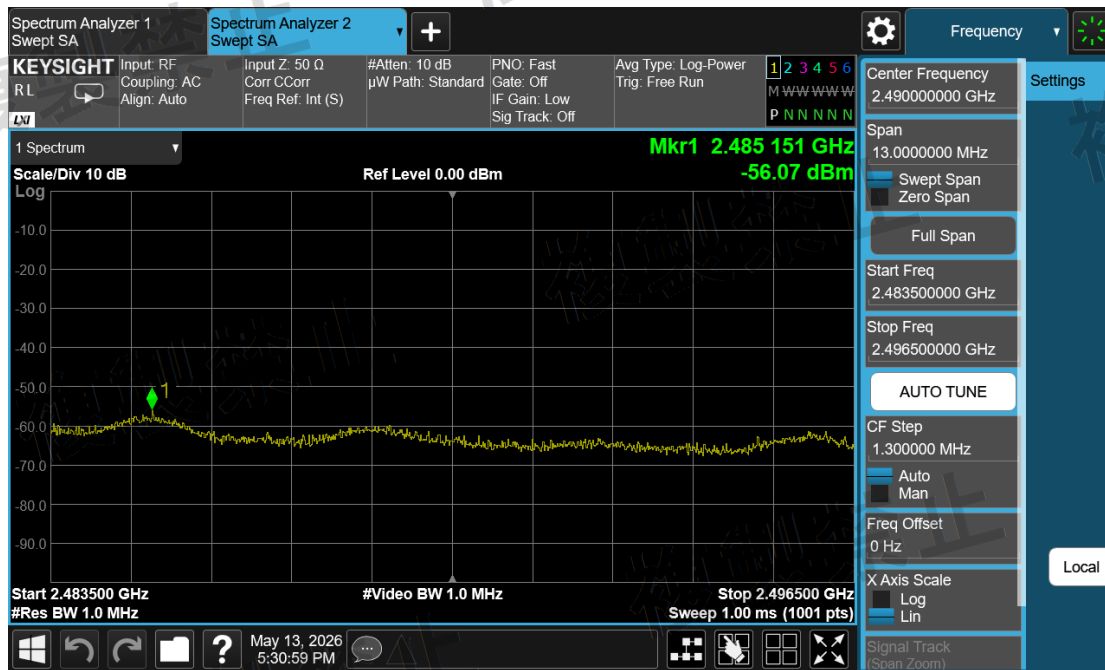
Channel Sounding_Mode 2\Unwanted Emission Strength\2483.50~2496.50-2478-ANT2-N
