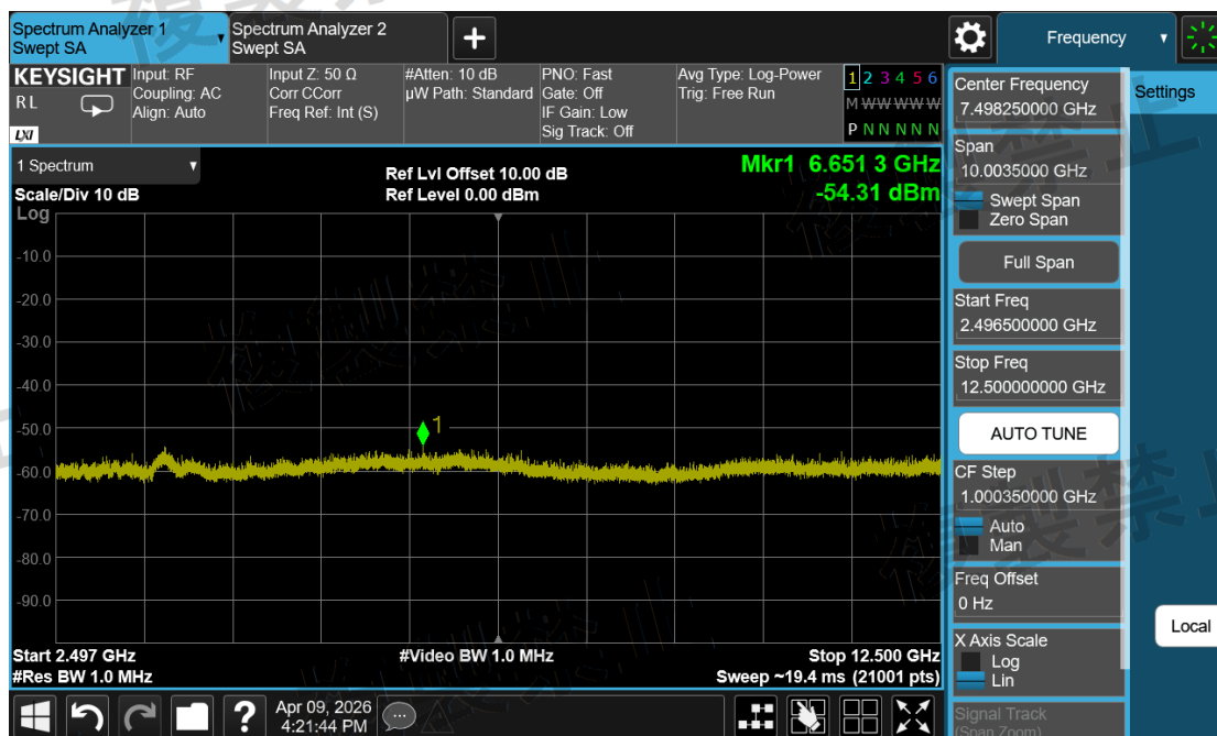
Channel Sounding_Mode 0\Unwanted Emission Strength\2496.5M~12500M-2441-ANT1-N
