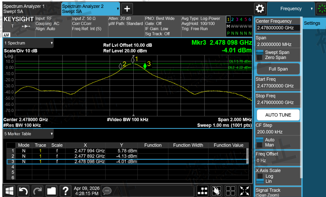
Channel Sounding_Mode 0\Frequency Error\2478-ANT1-N
