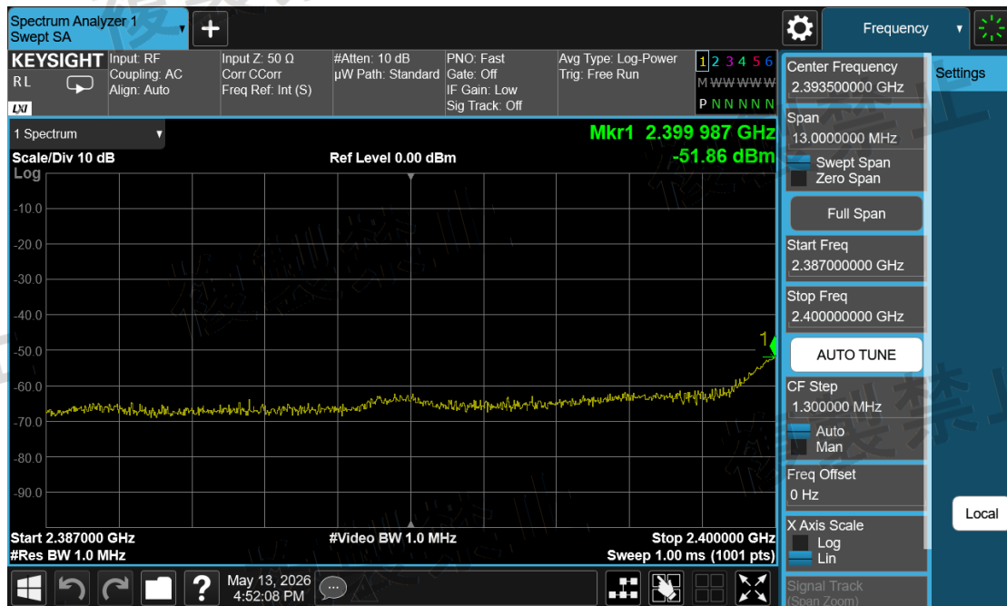
Channel Sounding_Mode 2\Unwanted Emission Strength\2387.00~2400.00-2404-ANT2-N
