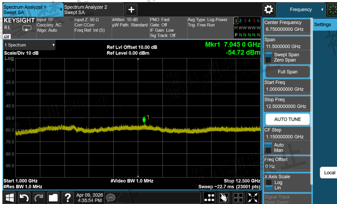
Channel Sounding_Mode 0\Secondarily Emitted Radio Wave Strength\1000M~12500M-2478-ANT1-N
