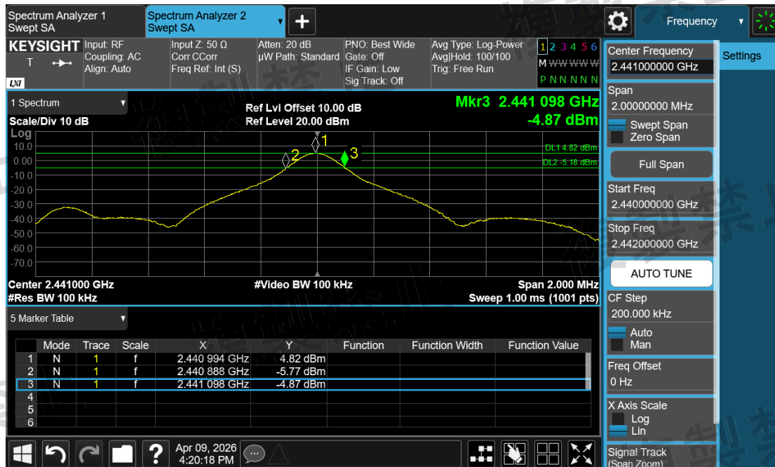
Channel Sounding_Mode 0\Frequency Error\2441-ANT1-N
