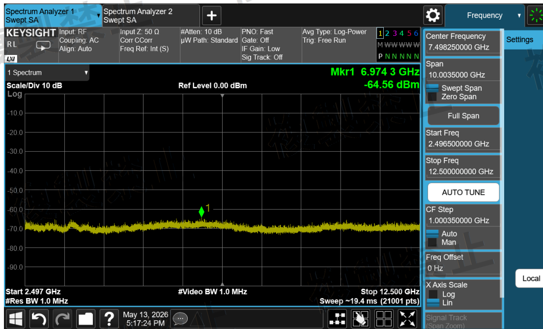
Channel Sounding_Mode 2\Unwanted Emission Strength\2496.50~12500.00-2441-ANT2-N
