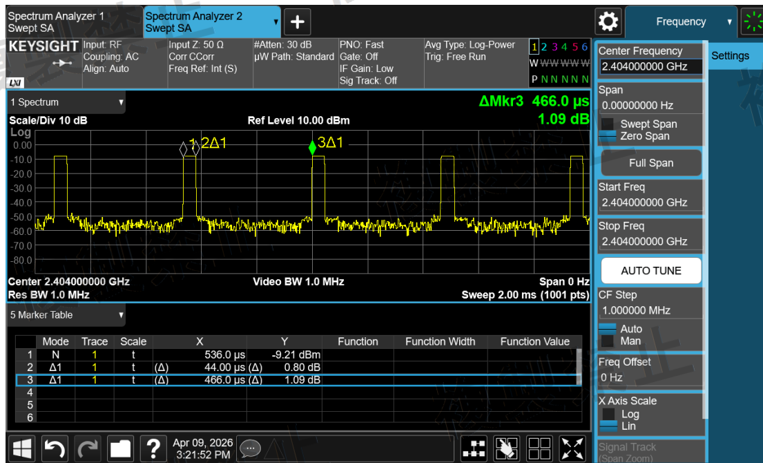
Channel Sounding_Mode 0\Dwell Time\2404
