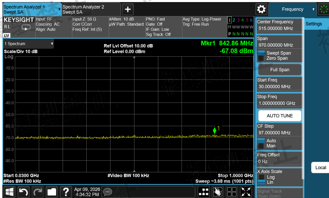
Channel Sounding_Mode 0\Secondarily Emitted Radio Wave Strength\30M~1000M-2441-ANT1-N
