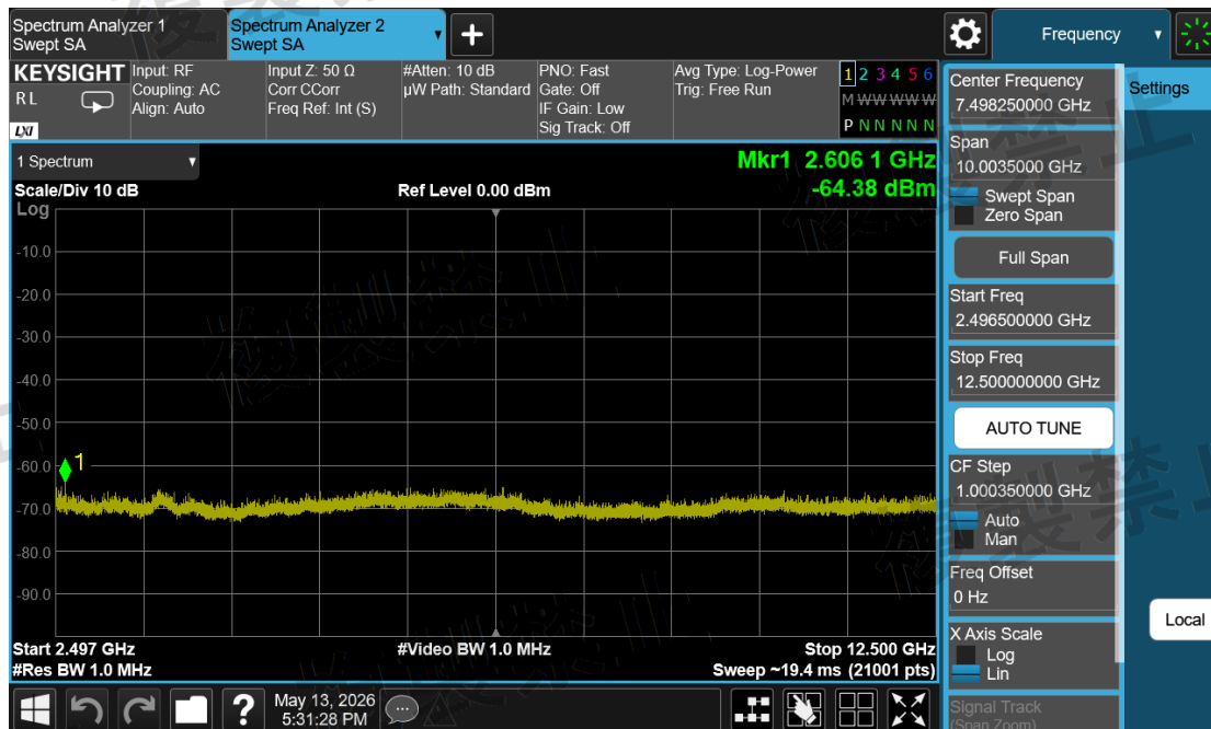
Channel Sounding_Mode 2\Unwanted Emission Strength\2496.50~12500.00-2478-ANT2-N
