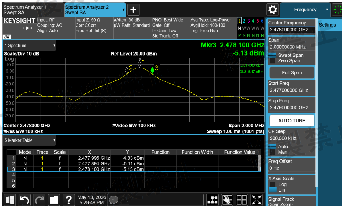
Channel Sounding_Mode 2\Frequency Error\2478-ANT2-N
