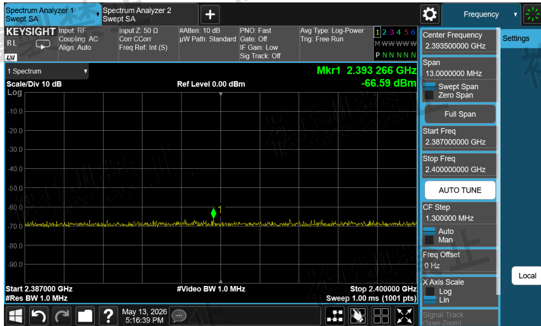
Channel Sounding_Mode 2\Unwanted Emission Strength\2387.00~2400.00-2441-ANT2-N
