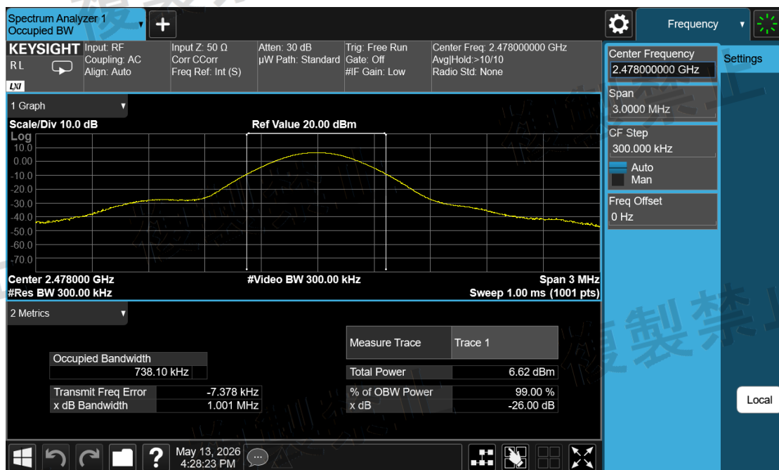
Channel Sounding_Mode 0\Occupied Bandwidth\2478-ANT1-N
