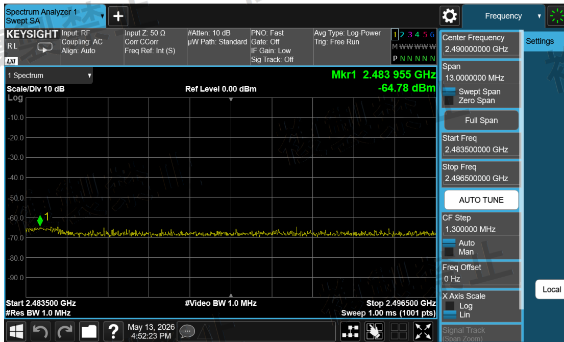
Channel Sounding_Mode 2\Unwanted Emission Strength\2483.50~2496.50-2404-ANT2-N
