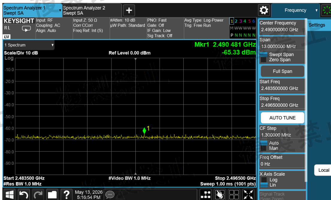
Channel Sounding_Mode 2\Unwanted Emission Strength\2483.50~2496.50-2441-ANT2-N
