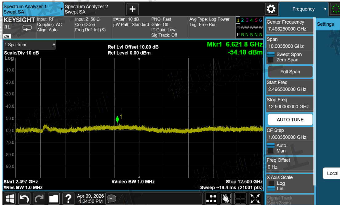
Channel Sounding_Mode 0\Unwanted Emission Strength\2496.5M~12500M-2478-ANT1-N
