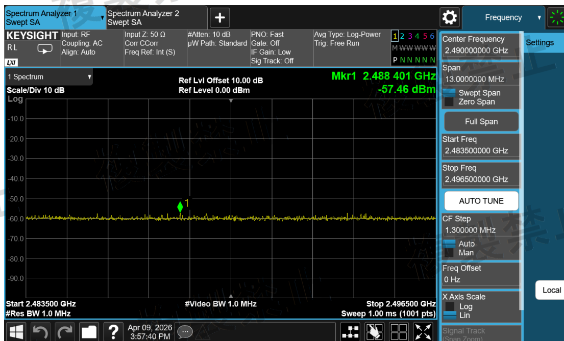
Channel Sounding_Mode 0\Unwanted Emission Strength\2483.5M~2496.5M-2404-ANT1-N
