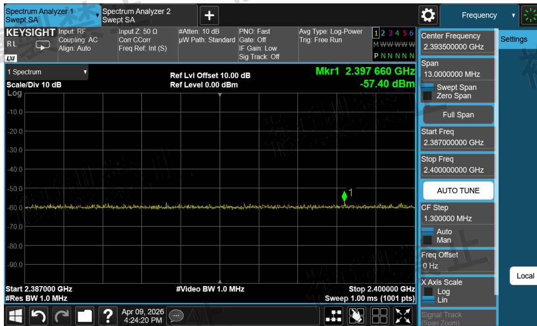
Channel Sounding_Mode 0\Unwanted Emission Strength\2387M~2400M-2478-ANT1-N
