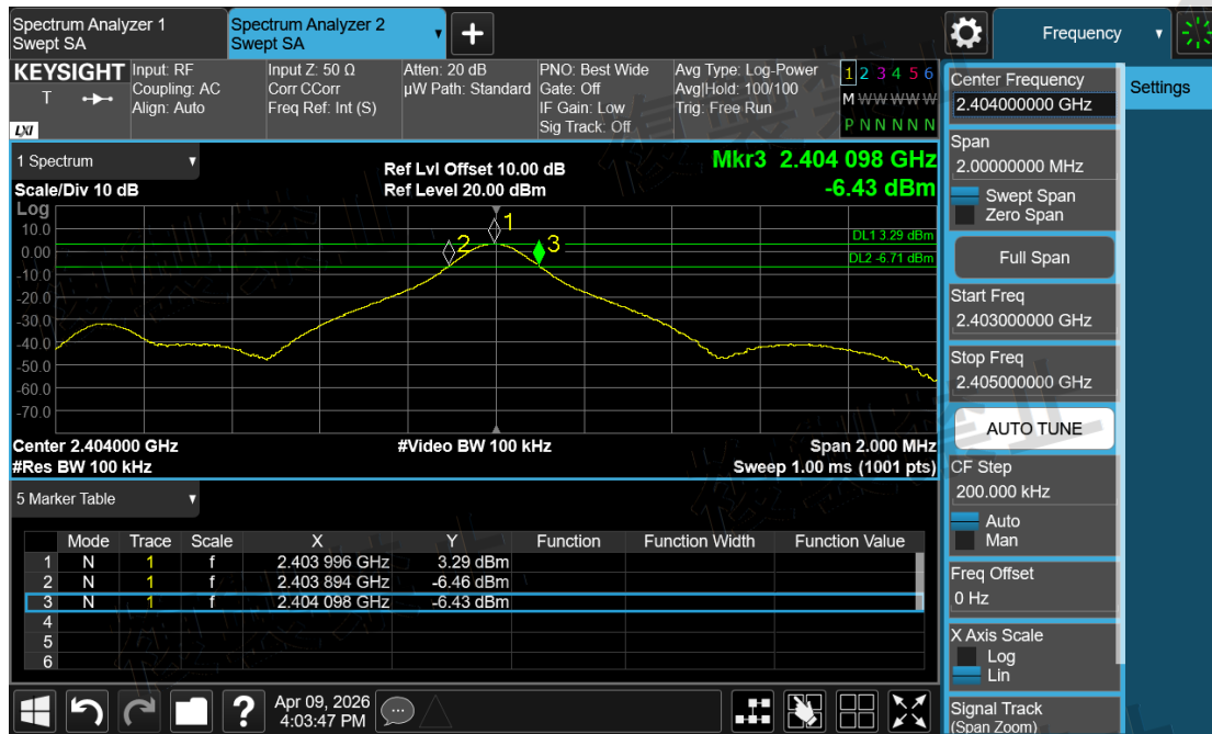
Channel Sounding_Mode 0\Frequency Error\2404-ANT1-N
