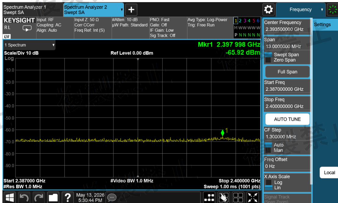
Channel Sounding_Mode 2\Unwanted Emission Strength\2387.00~2400.00-2478-ANT2-N
