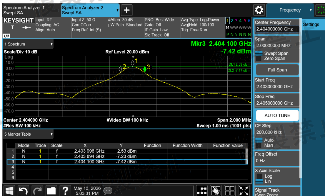
Channel Sounding_Mode 2\Frequency Error\2404-ANT2-N
