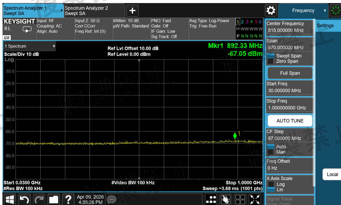
Channel Sounding_Mode 0\Secondarily Emitted Radio Wave Strength\30M~1000M-2478-ANT1-N
