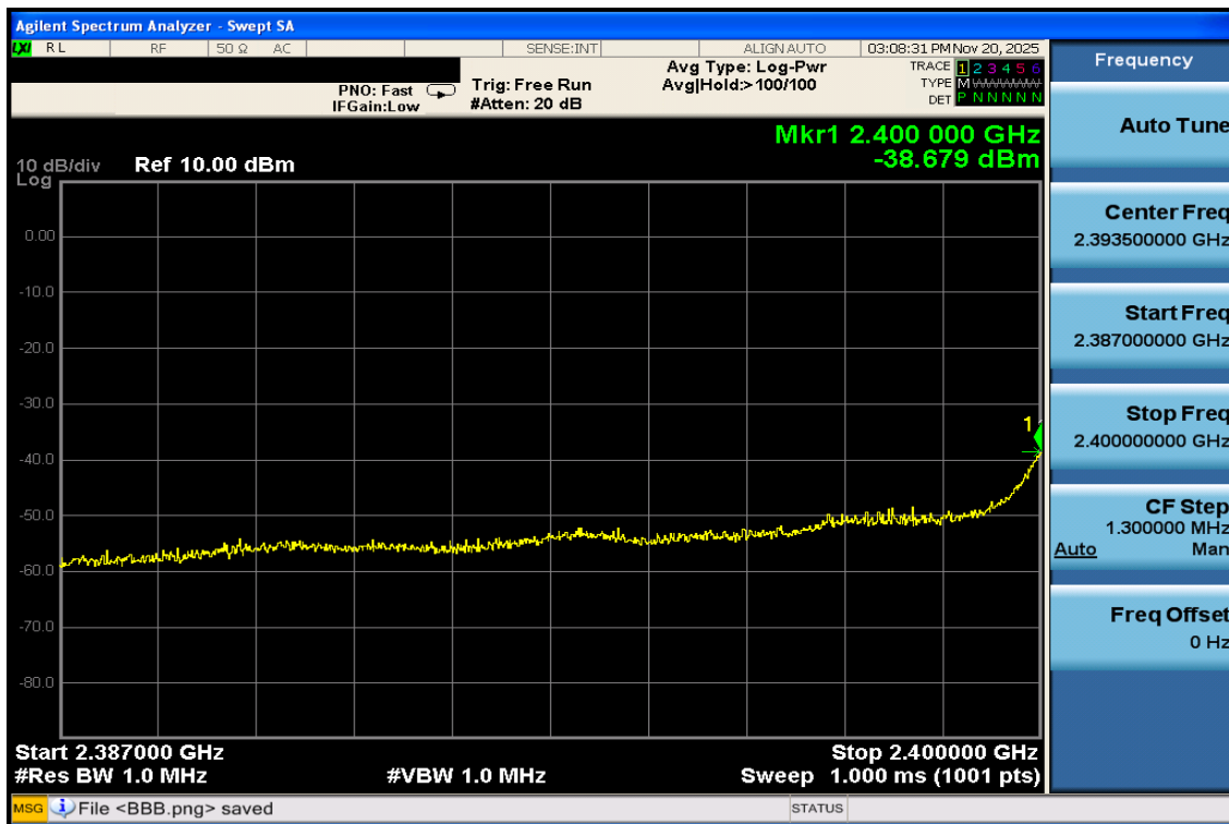
SRD\Unwanted Emission Strength\High Voltage\2387-2400M_2403-H
