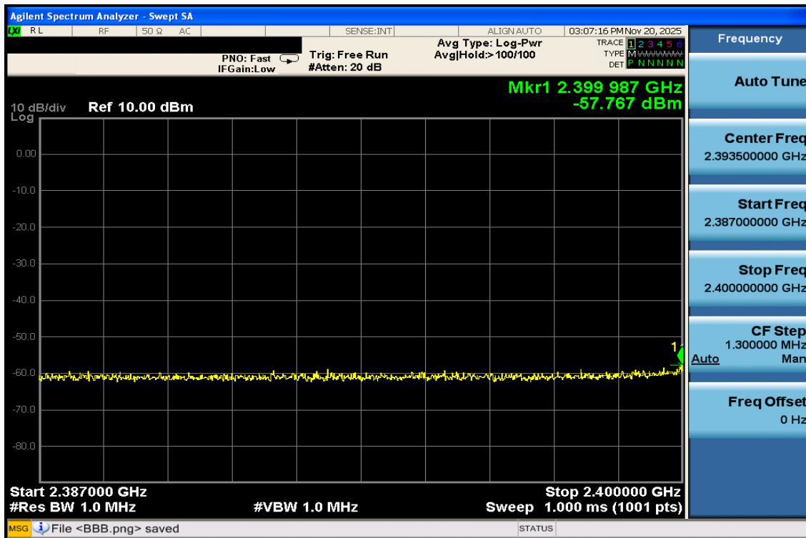
SRD\Unwanted Emission Strength\High Voltage\2387-2400M_2441-H
