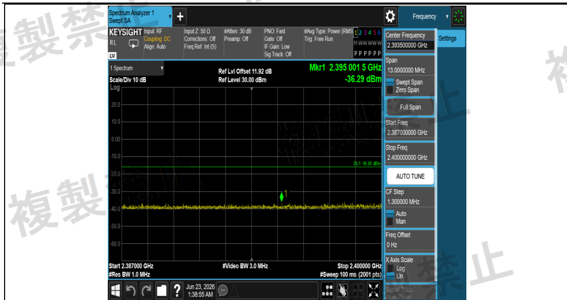
NTNV_11G_Ant1_2412_2387~2400
