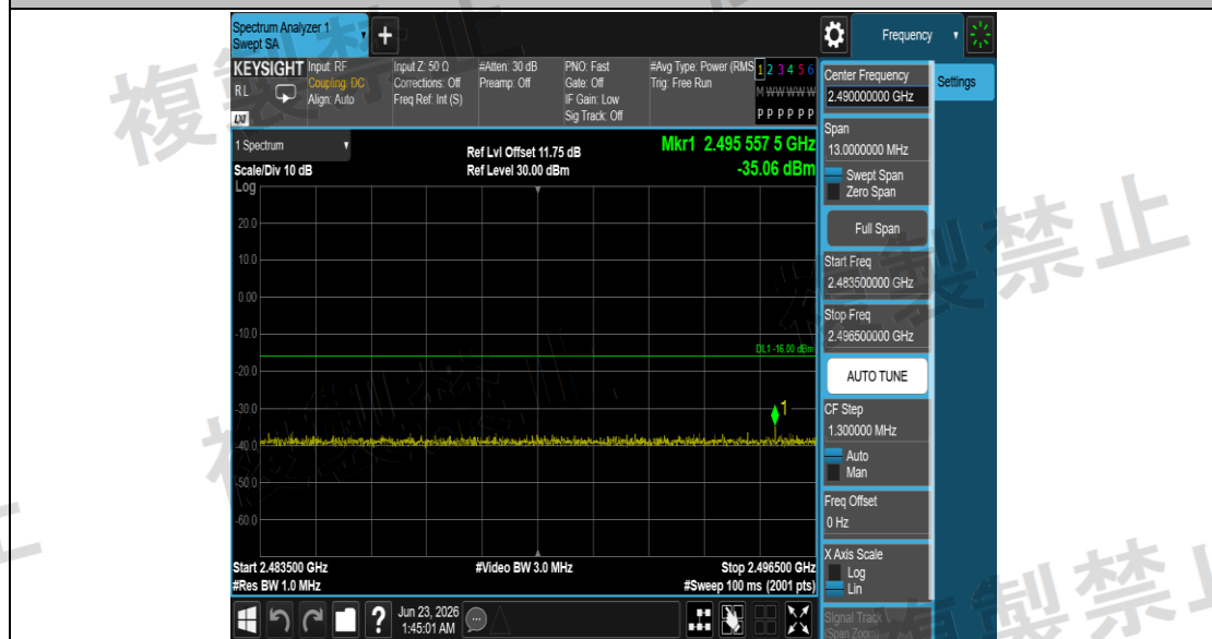
NTNV_11G_Ant1_2442_2483.5~2496.5
