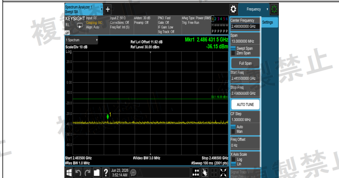
NTNV_11AX20SISO_Ant1_2412_2483.5~2496.5
