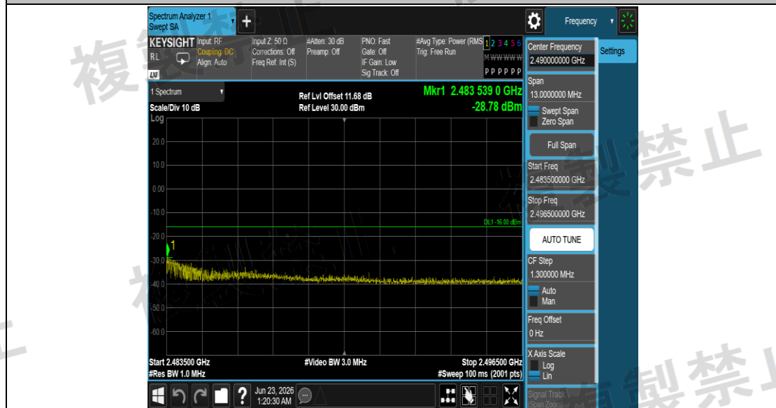
NTNV_11B_Ant1_2472_2483.5~2496.5
