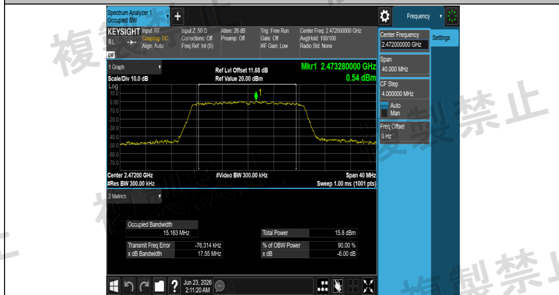
NTNV_11N20SISO_Ant1_2472
