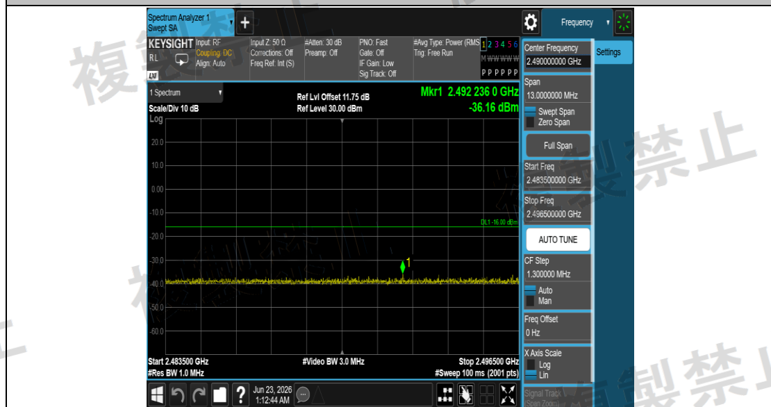
NTNV_11B_Ant1_2442_2483.5~2496.5
