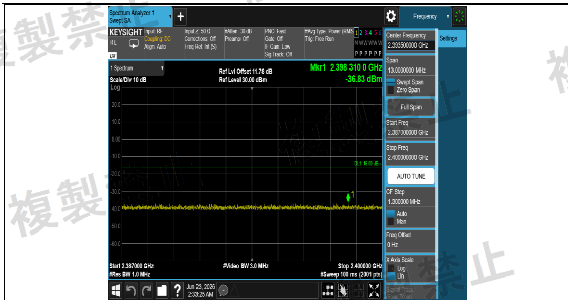
NTNV_11N40SISO_Ant1_2462_2387~2400
