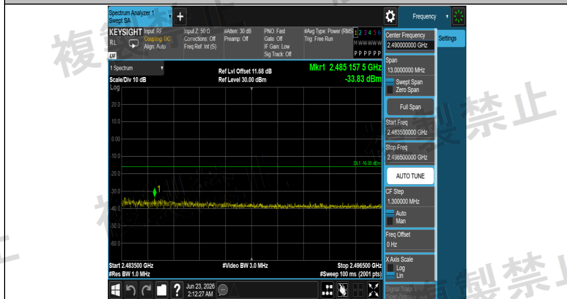
NTNV_11N20SISO_Ant1_2472_2483.5~2496.5
