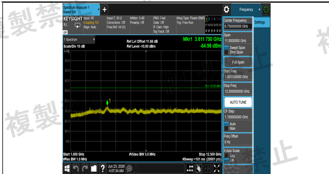
NTNV_11N20SISO_Ant1_2472_1000~12500
