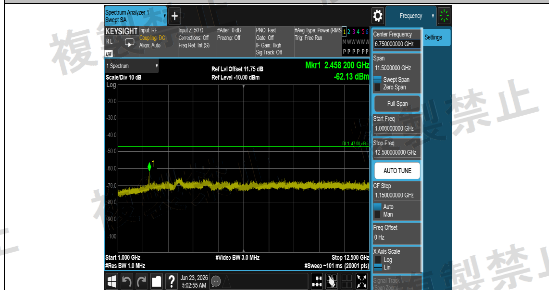
NTNV_11AX40SISO_Ant1_2442_1000~12500
