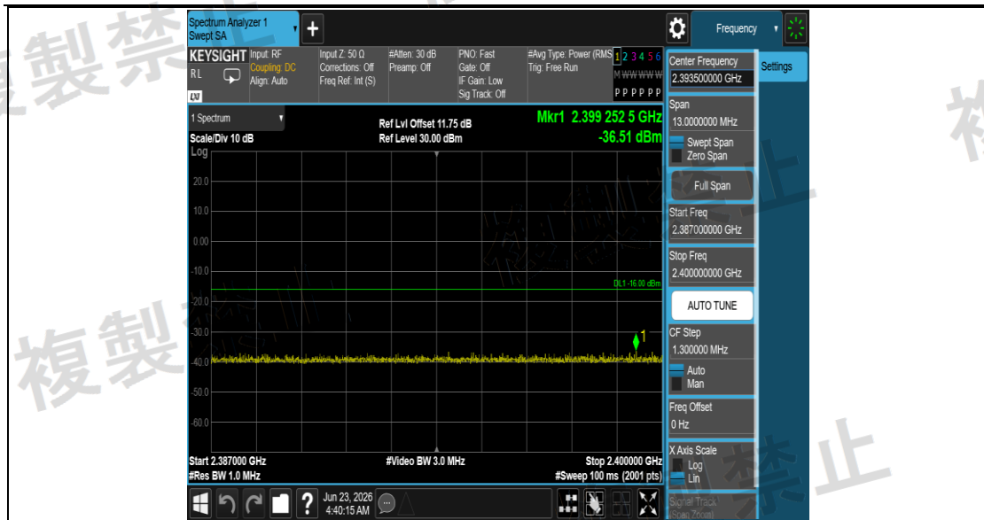
NTNV_11AX40SISO_Ant1_2442_2387~2400
