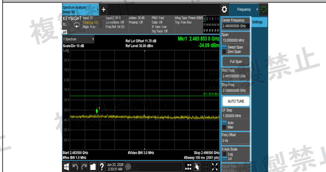
NTNV_11N40SISO_Ant1_2462_2483.5~2496.5
