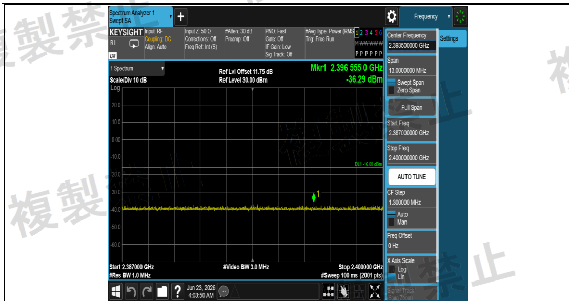
NTNV_11AX20SISO_Ant1_2442_2387~2400
