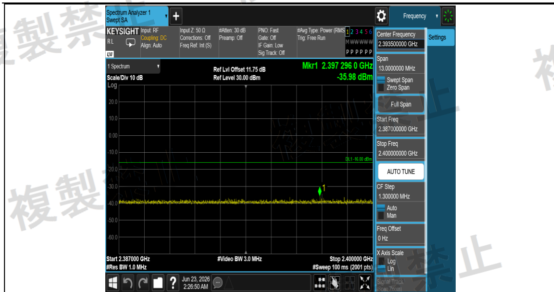
NTNV_11N40SISO_Ant1_2442_2387~2400
