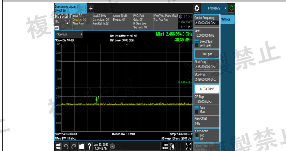
NTNV_11N20SISO_Ant1_2412_2483.5~2496.5
