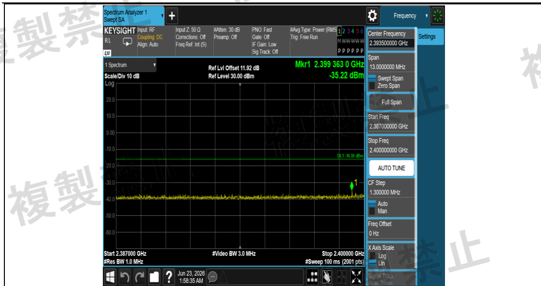
NTNV_11N20SISO_Ant1_2412_2387~2400
