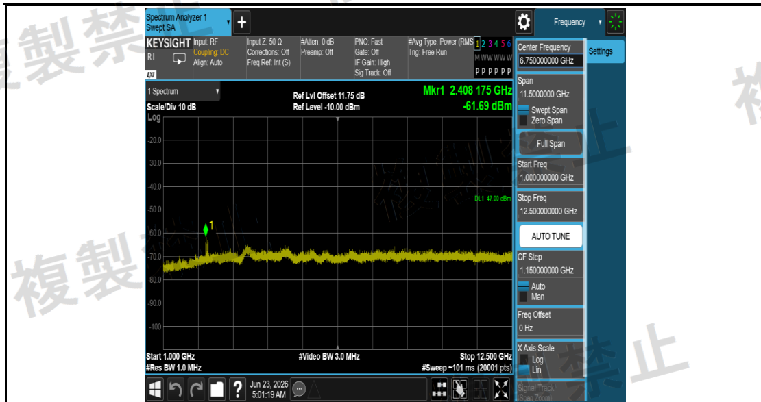
NTNV_11AX20SISO_Ant1_2442_1000~12500
