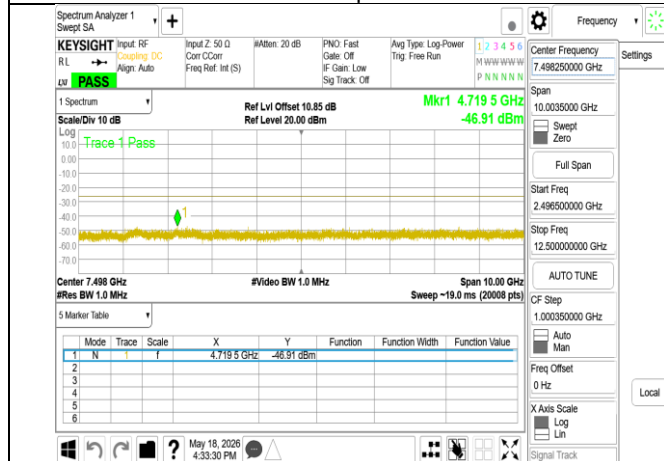
TX_2496.5MHz~12.5GHz_π/4DQPSK_2M_DH5_2441MHz
