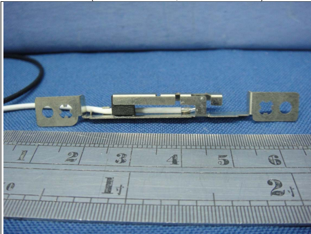
Antenna 2 (Chain 0 / Brand: WNC, Model: 81.ED415.001)
