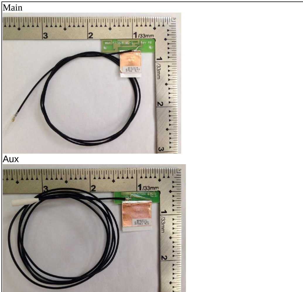
Antenna 13_ SK5DMWIPB01+A(MAIN), SK5DMWIPB03+C(AUX), WGT , 2016/8/22
