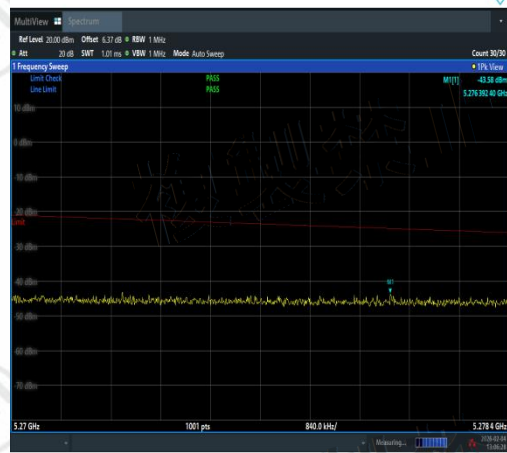
NTNV-11AX40MIMO-Ant2-5230-5270~5278.4-P
