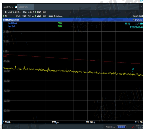
NTNV-11N40MIMO-Ant1-5230-5250~5251-PASS
