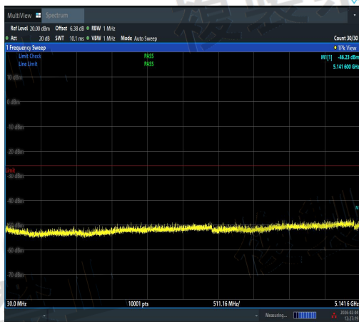
NTNV-11AX40MIMO-Ant1-5190-30~5141.6-PAS S
