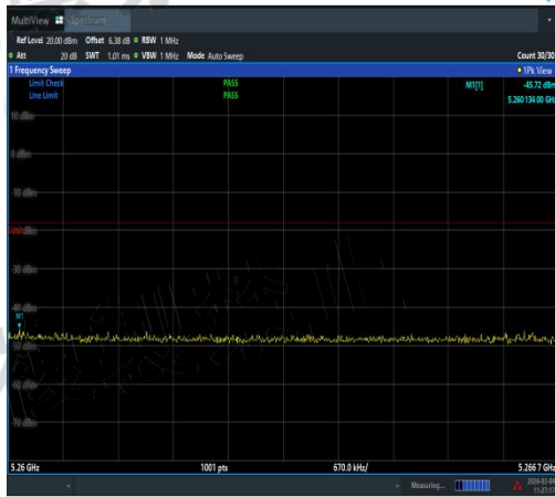
NTVN-11AX20MIMO-Ant3-5180-5260~5266.7-P ASS
