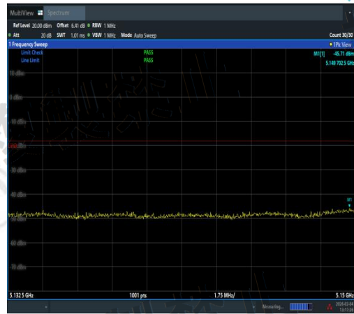
NTVN-11AX80MIMO-Ant3-5210-5132.5~5150-P ASS
