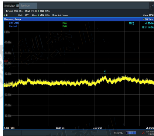
NTNV-11AX20SISO-Ant2-5240-5266.7~26000-P ASS
