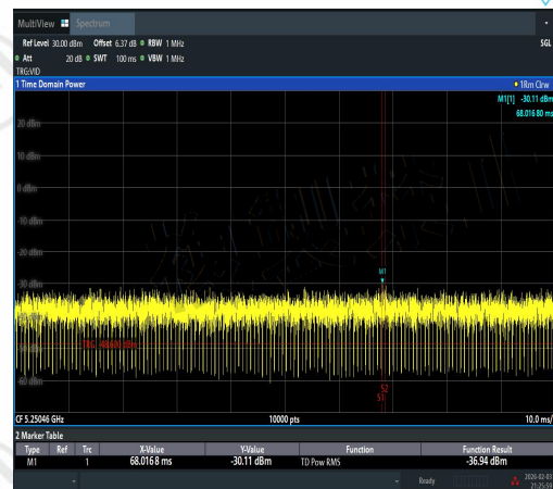
NTVN-11N20MIMO-Ant2-5240-5250~5251-PASS
