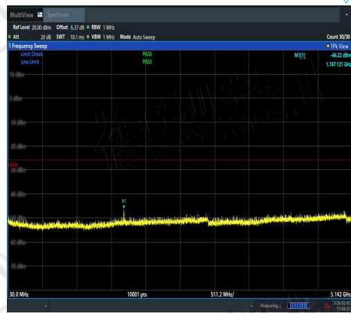
NTNV-11AX20SISO-Ant2-5240-30~5142-PASS
