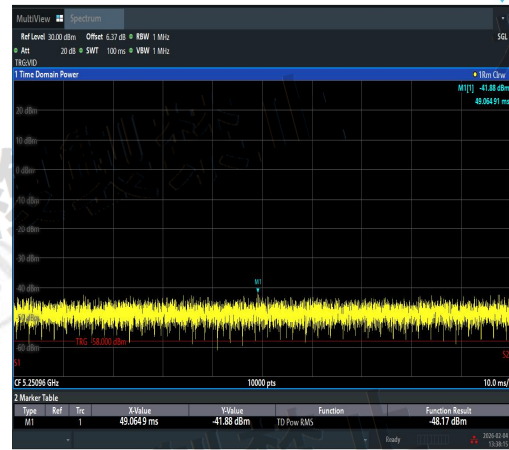
NTVN-11N40MIMO-Ant2-5230-5250~5251-PASS
