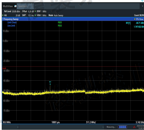
NTNV-11AX20SISO-Ant1-5240-30~5142-PASS
