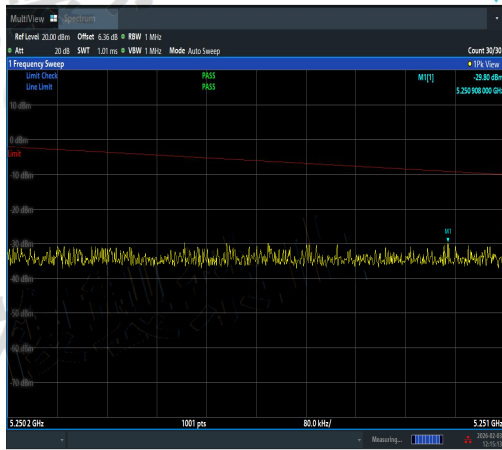
NTNV-11AX20SISO-Ant1-5220-5250.2~5251-PA
