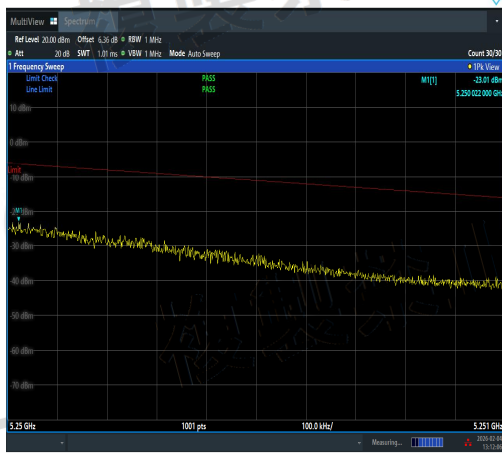
NTVN-11AX80MIMO-Ant1-5210-5250~5251-PAS S
