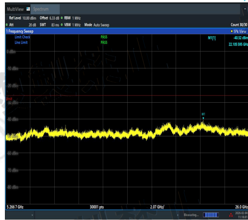
NTVN-11AX20MIMO-Ant1-5180-5266.7~26000-P ASS
