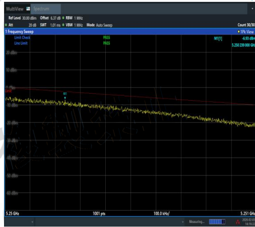
NTNV-11A-Ant2-5240-5250~5251-PASS
