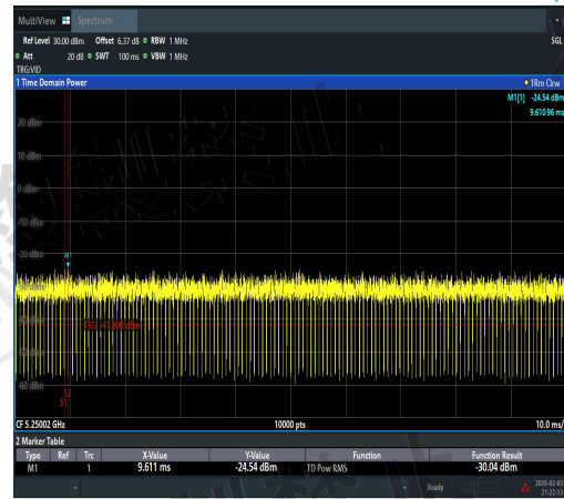
NTVN-11N20MIMO-Ant1-5240-5250~5251-PASS
