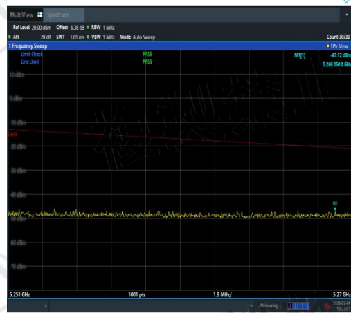
NTNV-11AX40MIMO-Ant3-5190-5251~5270-PAS
