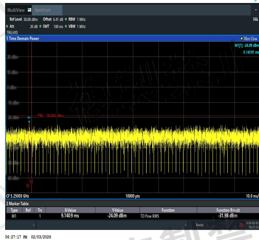
NTNV-11A-Ant3-5240-5250~5251-PASS
