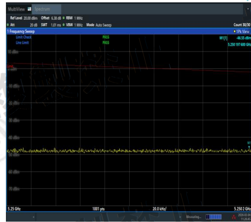
NTVN-11AX20MIMO-Ant3-5180-5250~5250.2-P ASS
