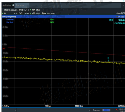
NTVN-11N40MIMO-Ant3-5230-5250~5251-PASS
