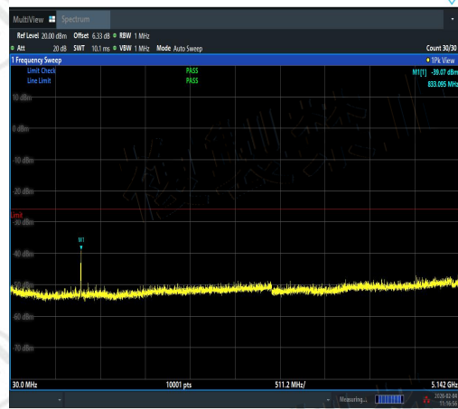
NTNV-11AX20MIMO-Ant1-5180-30~5142-PASS
