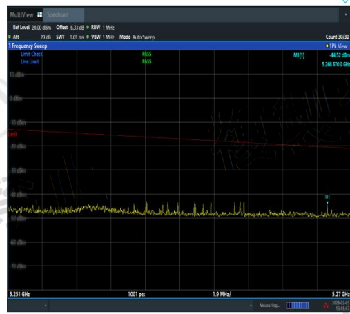
NTNV-11AX40SISO-Ant2-5190-5250~5251-PAS S
