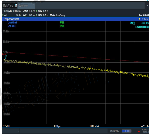
NTVN-11N20MIMO-Ant1-5240-5250~5251-PASS
