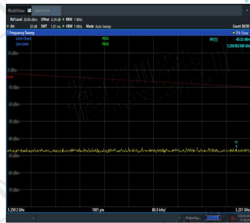
NTVN-11AX20MIMO-Ant2-5180-5250.2~5251-P ASS
