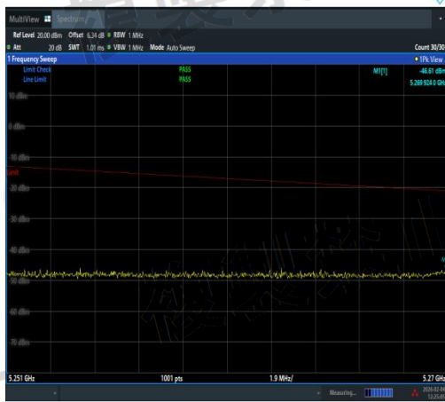
NTNV-11AX40MIMO-Ant2-5190-5251~5270-PAS
