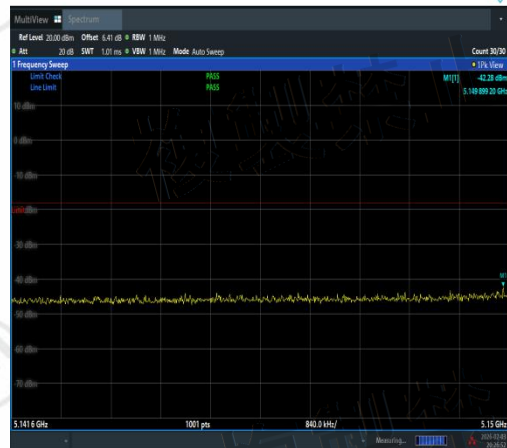
NTNV-11AX40SISO-Ant3-5230-5141.6~5150-PA SS
