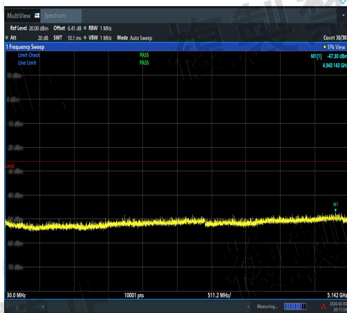
NTNV-11AX20SISO-Ant3-5240-30~5142-PASS
