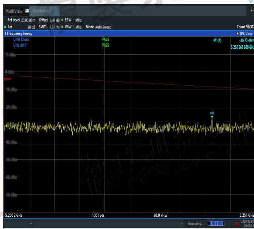
NTNV-11AX20SISO-Ant3-5220-5250.2~5251-PA
