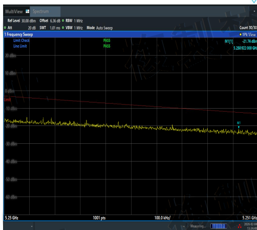
NTVN-11N40MIMO-Ant1-5230-5250~5251-PASS
