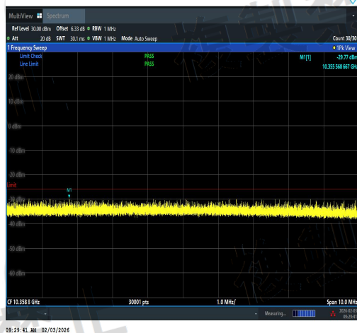
NTNV-11N20SISO-Ant1-5180-5266.7~26000-PA
