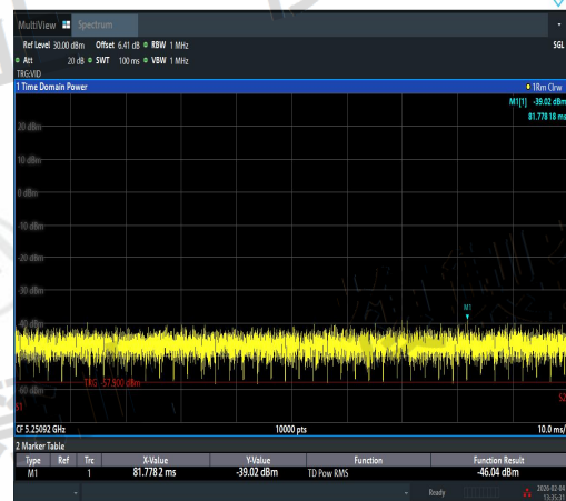
NTVN-11N40MIMO-Ant1-5230-5250~5251-PASS
