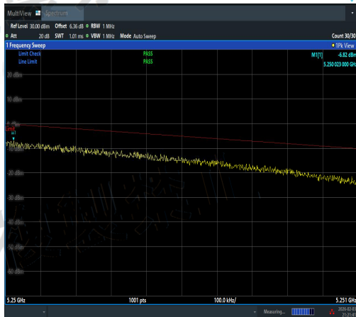
NTVN-11N20MIMO-Ant1-5240-5250~5251-PASS
