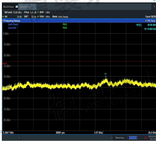
NTNV-11AX20SISO-Ant3-5240-5266.7~26000-P ASS
