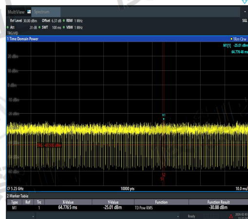
NTVN-11N20MIMO-Ant3-5240-5250~5251-PASS
