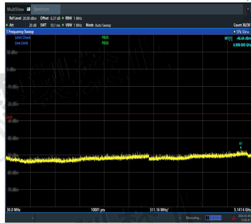
NTNV-11AX40MIMO-Ant2-5230-30~5141.6-PAS
