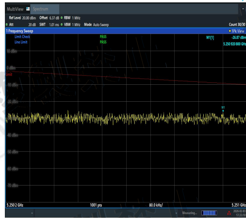
NTNV-11AX20SISO-Ant2-5220-5250.2~5251-PA
