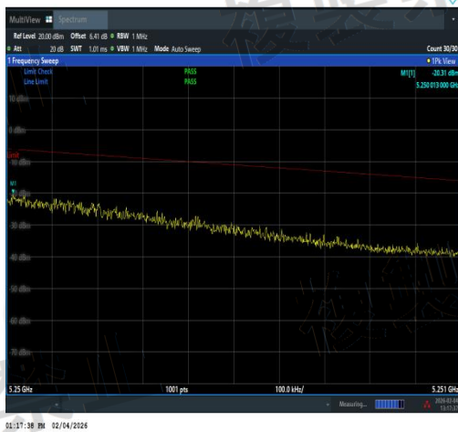
NTVN-11AX80MIMO-Ant1-5210-5250~5251-PAS S
