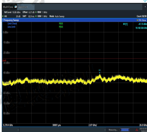
NTNV-11AX40SISO-Ant2-5230-5278.4~26000-P ASS
