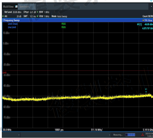
NTNV-11AX40MIMO-Ant3-5230-30~5141.6-PAS
