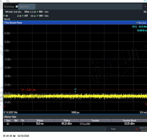
NTNV-11N20SISO-Ant1-5180-5266.7~26000-PA
