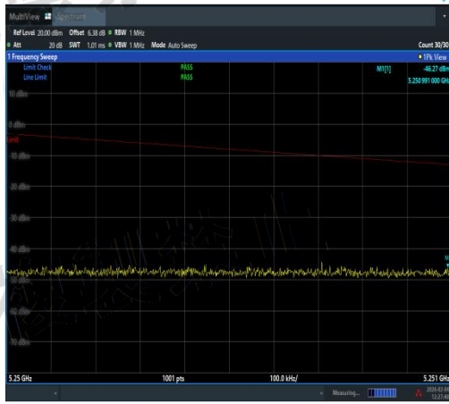
NTNV-11AX40MIMO-Ant3-5190-5250~5251-PAS
