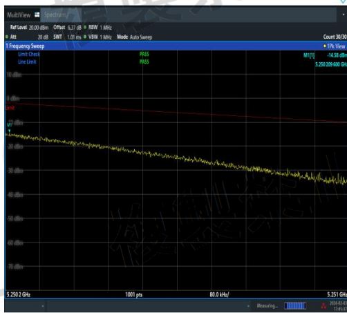
NTNV-11AX20SISO-Ant2-5240-5250.2~5251-PA SS
