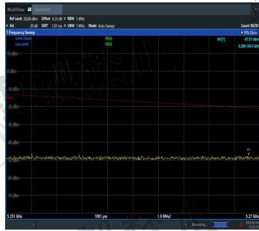
NTNV-11AX40MIMO-Ant1-5190-5251~5270-PAS
