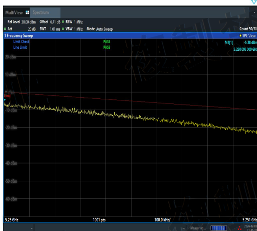
NTVN-11N20MIMO-Ant3-5240-5250~5251-PASS
