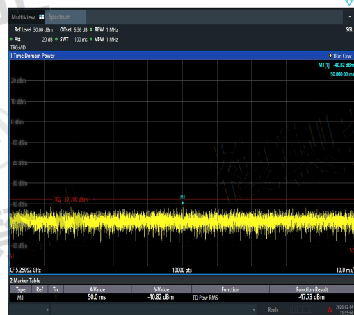
NTNV-11N40MIMO-Ant1-5230-5250~5251-PASS
