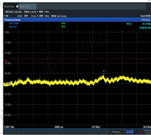
NTVN-11AX20MIMO-Ant3-5180-5266.7~26000-P ASS
