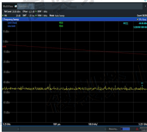
NTNV-11AX40SISO-Ant1-5190-5250~5251-PAS S
