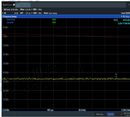
NTVN-11AX20MIMO-Ant2-5180-5250~5250.2-P ASS
