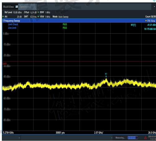
NTNV-11AX40SISO-Ant2-5190-5278.4~26000-P ASS
