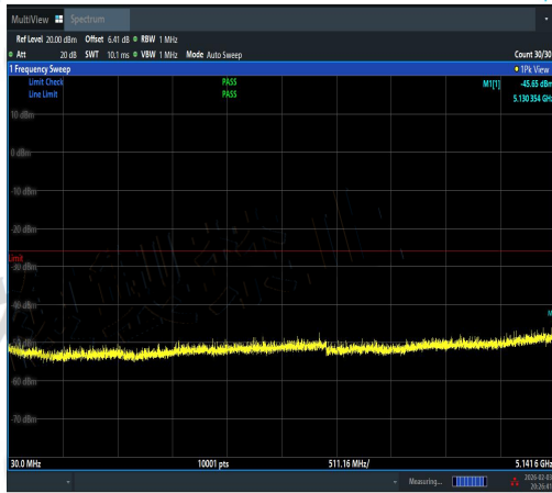
NTNV-11AX40SISO-Ant3-5230-30~5141.6-PASS
