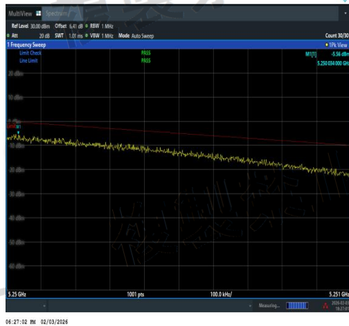
NTNV-11A-Ant3-5240-5250~5251-PASS
