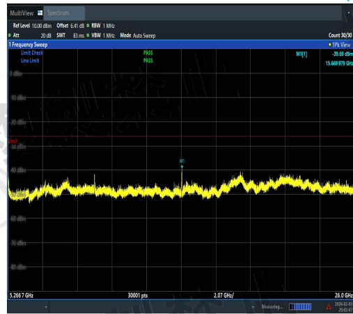
NTNV-11AX20SISO-Ant3-5220-5266.7~26000-P ASS
