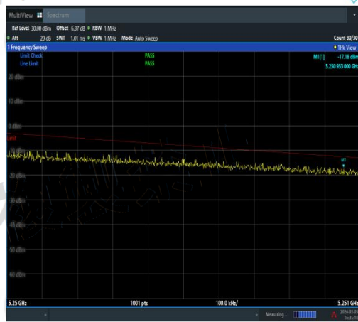
NTNV-11N40SISO-Ant2-5230-5250~5251-PASS
