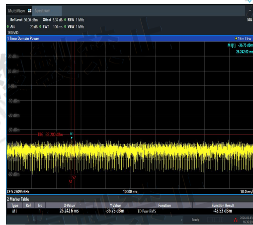
NTNV-11N40SISO-Ant2-5230-5250~5251-PASS
