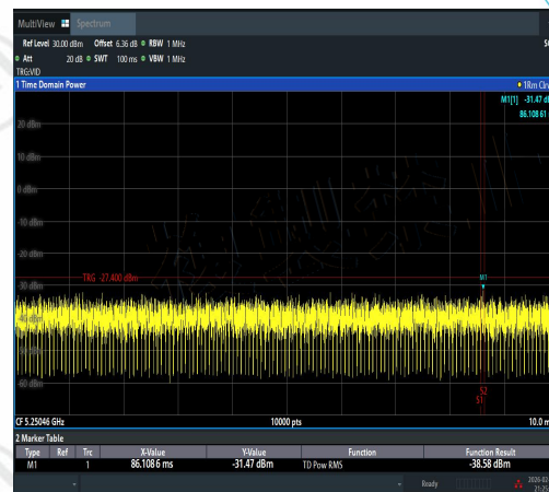
NTNV-11N20MIMO-Ant2-5240-5250~5251-PASS
