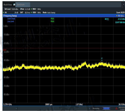
NTNV-11AX40SISO-Ant1-5190-5278.4~26000-P ASS
