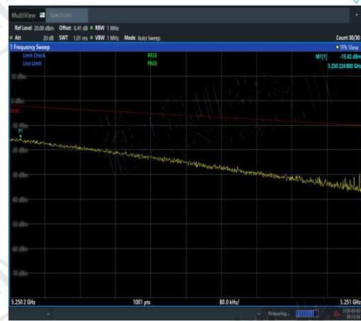
NTNV-11AX20SISO-Ant3-5240-5250.2~5251-PA SS
