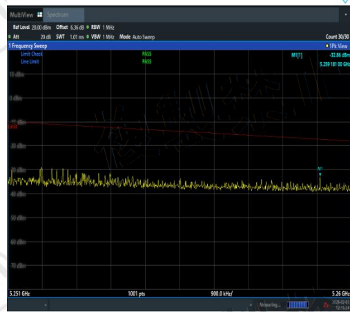
NTNV-11AX20SISO-Ant1-5220-5251~5260-PAS
