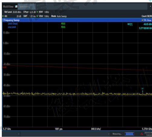
NTNV-11AX40MIMO-Ant1-5230-5270~5278.4-P
