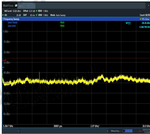
NTNV-11AX20SISO-Ant2-5220-5266.7~26000-P ASS
