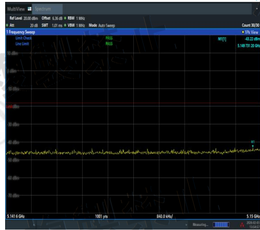
NTNV-11AX40SISO-Ant1-5230-5141.6~5150-PA SS
