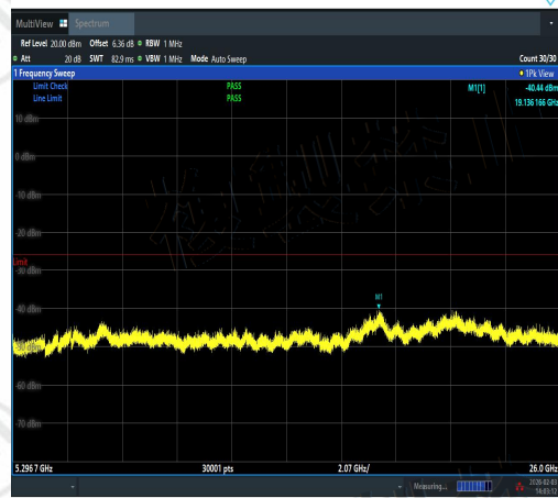
NTNV-11AX80SISO-Ant1-5210-5296.7~26000-P
