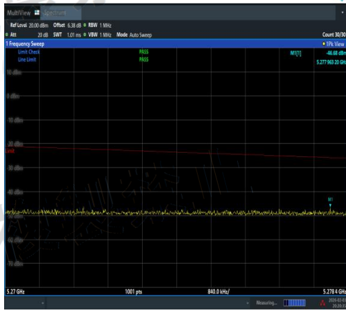
NTNV-11AX40SISO-Ant3-5190-5270~5278.4-PA SS
