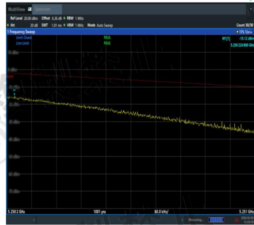
NTNV-11AX20SISO-Ant1-5240-5250.2~5251-PA SS
