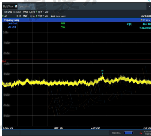
NTVN-11AX20MIMO-Ant2-5180-5266.7~26000-P ASS
