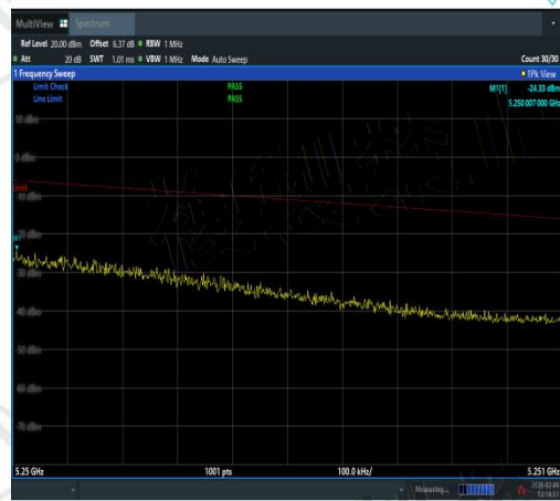
NTVN-11AX80MIMO-Ant2-5210-5250~5251-PAS S
