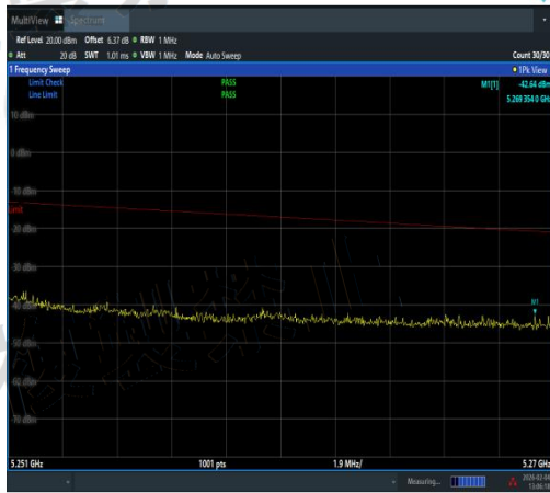
NTNV-11AX40MIMO-Ant2-5230-5251~5270-PAS
