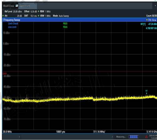
NTNV-11AX40MIMO-Ant1-5230-30~5141.6-PAS
