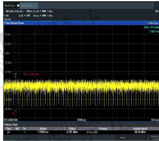
NTNV-11A-Ant2-5240-5250~5251-PASS
