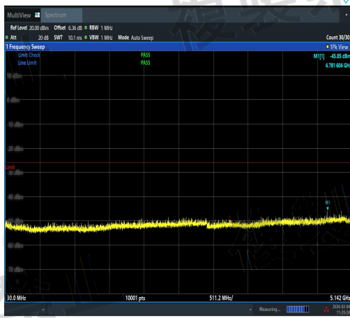
NTVN-11AX20MIMO-Ant2-5180-5266.7~26000-P ASS
