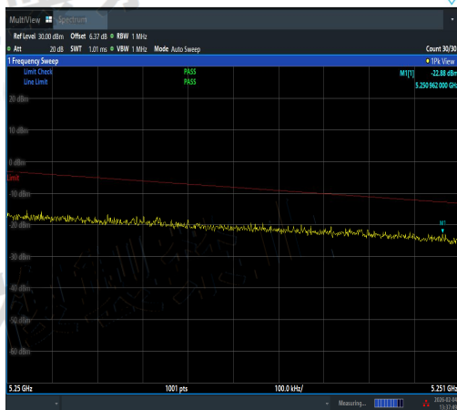
NTVN-11N40MIMO-Ant2-5230-5250~5251-PASS
