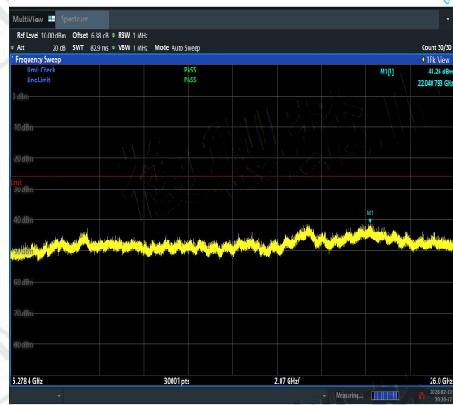
NTNV-11AX40SISO-Ant3-5190-5278.4~26000-P ASS
