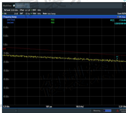
NTNV-11N40SISO-Ant3-5230-5250~5251-PASS
