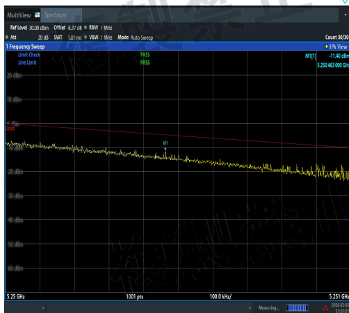
NTVN-11N20MIMO-Ant2-5240-5250~5251-PASS
