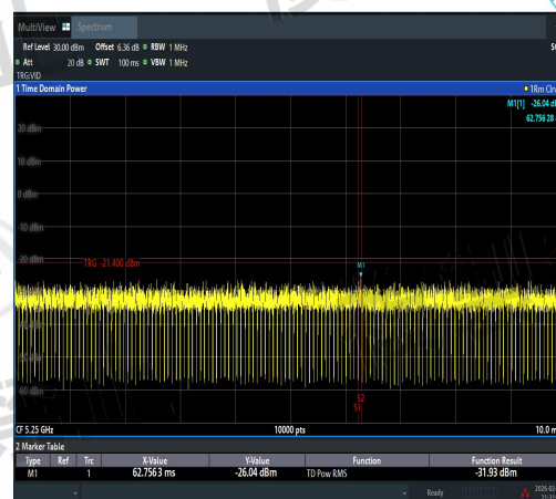
NTNV-11N20MIMO-Ant3-5240-5250~5251-PASS
