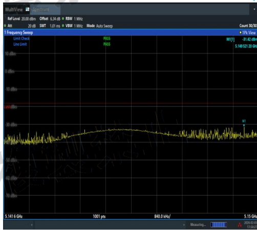
NTNV-11AX40SISO-Ant2-5190-5141.6~5150-PA SS
