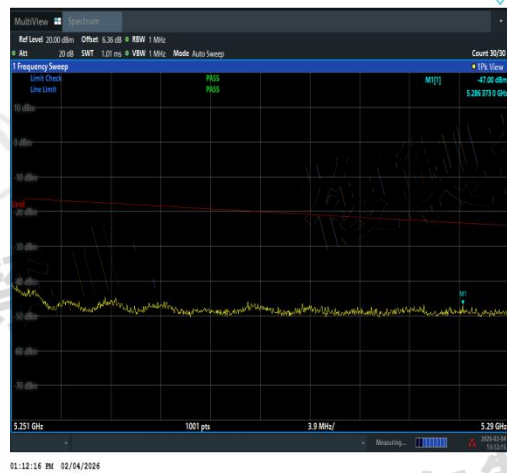
NTVN-11AX80MIMO-Ant2-5210-5250~5251-PAS S
