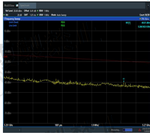
NTNV-11AX40MIMO-Ant3-5230-5251~5270-PAS
