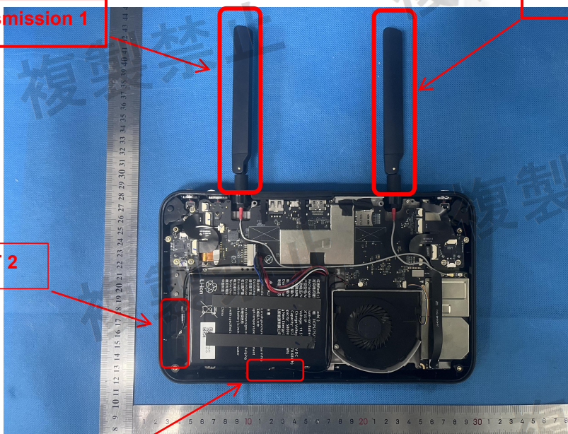
BT & 2.4G & 5G WIFI ANT 1
