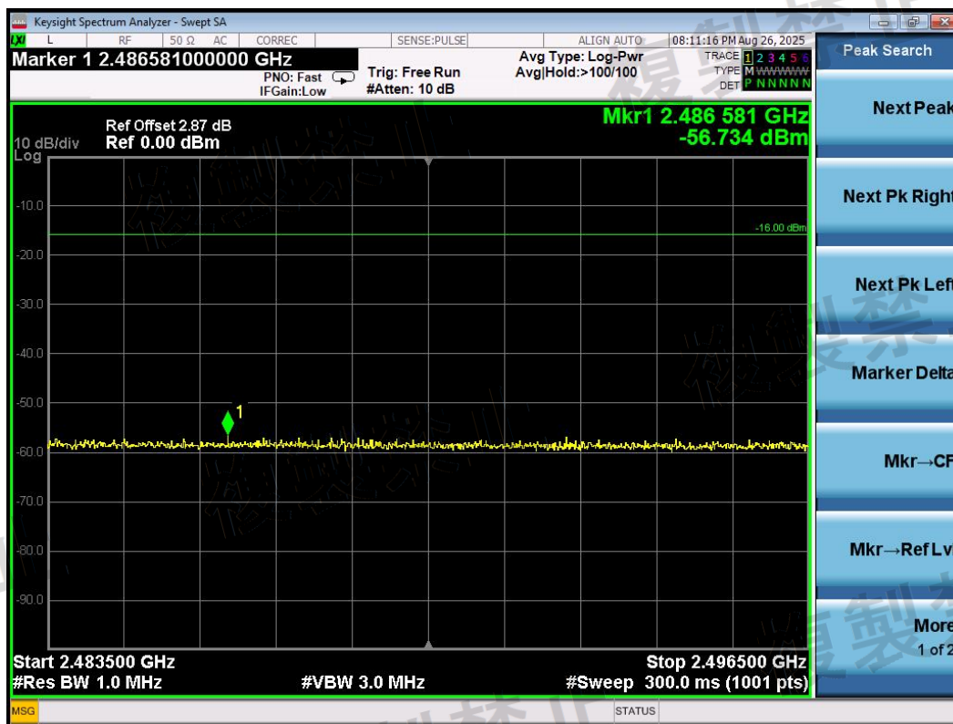
NTNV_BLE_Ant1_2402_2483.5~2496.5
