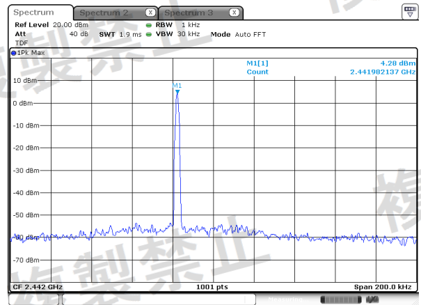
Ch.7: 2442MHz
