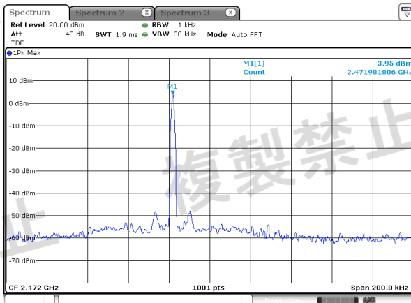
Ch.13: 2472MHz
