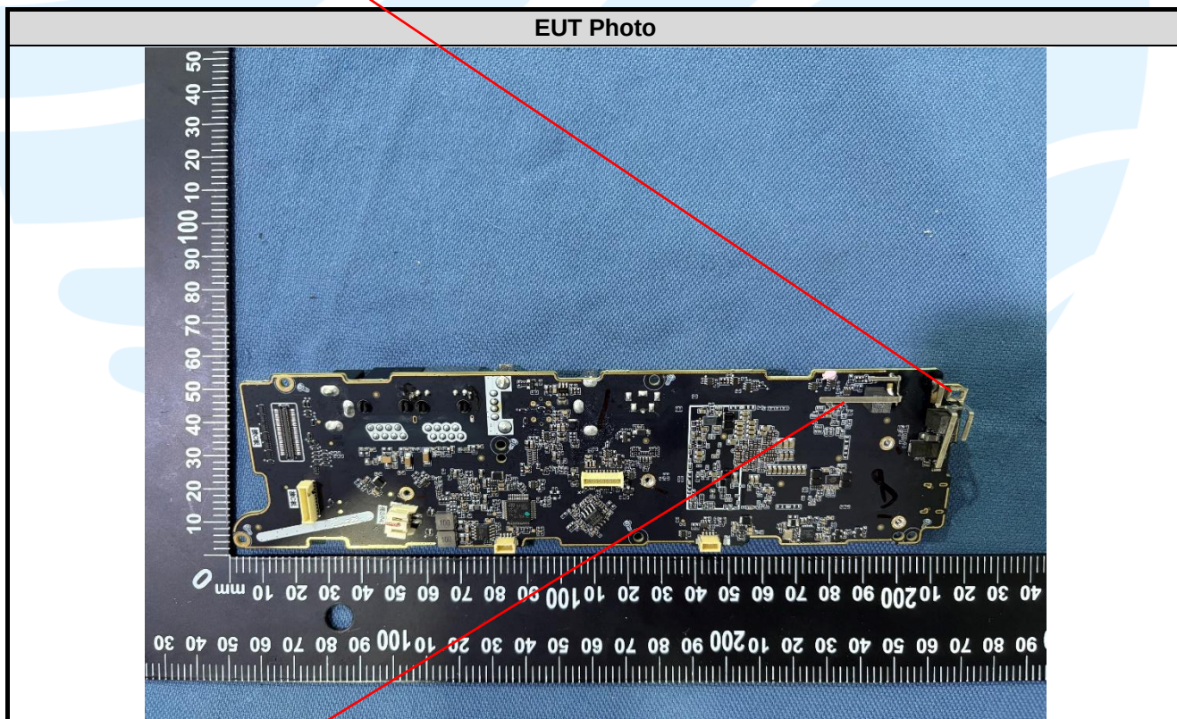
Bluetooth/ Wi-Fi Antenna 0
