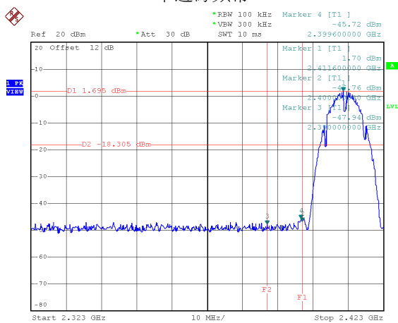
下邊緣頻帶-CH01
