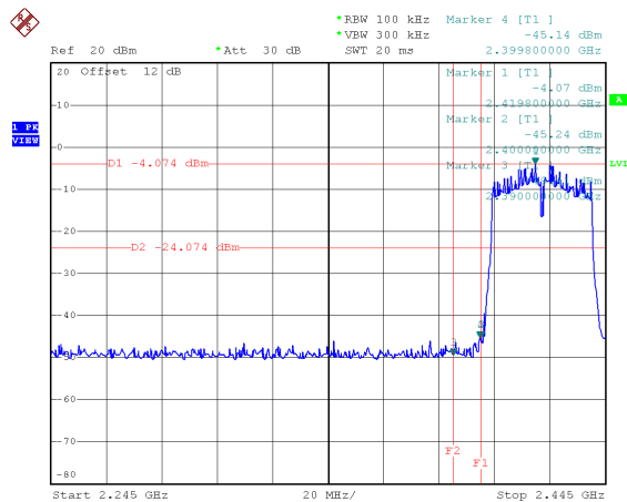
下邊緣頻帶-CH03
