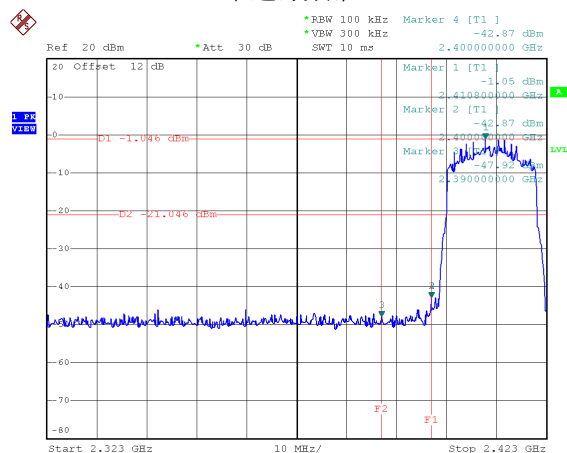
下邊緣頻帶-CH01
