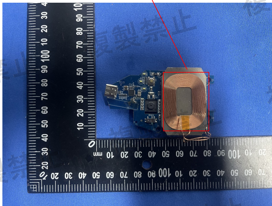
Wireless charging RX Antenna
