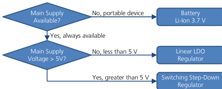
Figure 31: VCC supply concept selection
