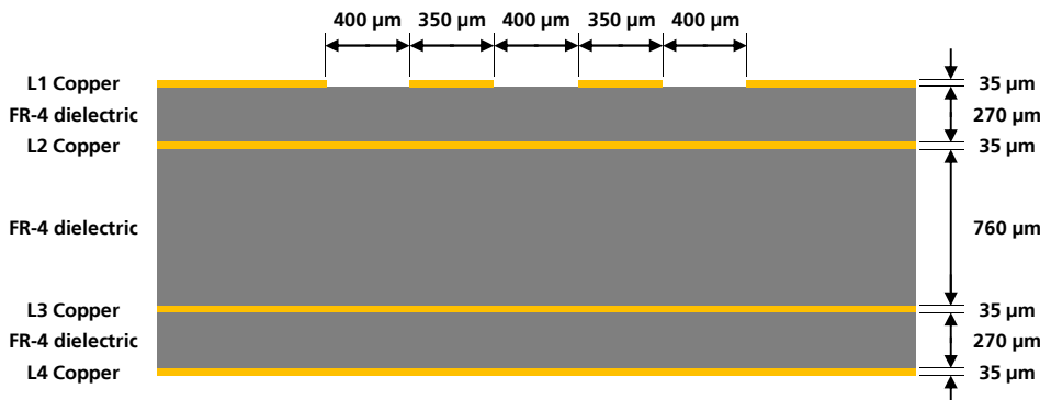
Figure 54: Example of USB line design, with Z_0 close to 90 \Omega and Z_{CM} close to 30 \Omega , for the described 4-layer board layout
