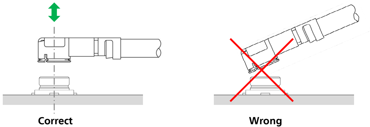
Figure 73: Precautions during RF connector mating
