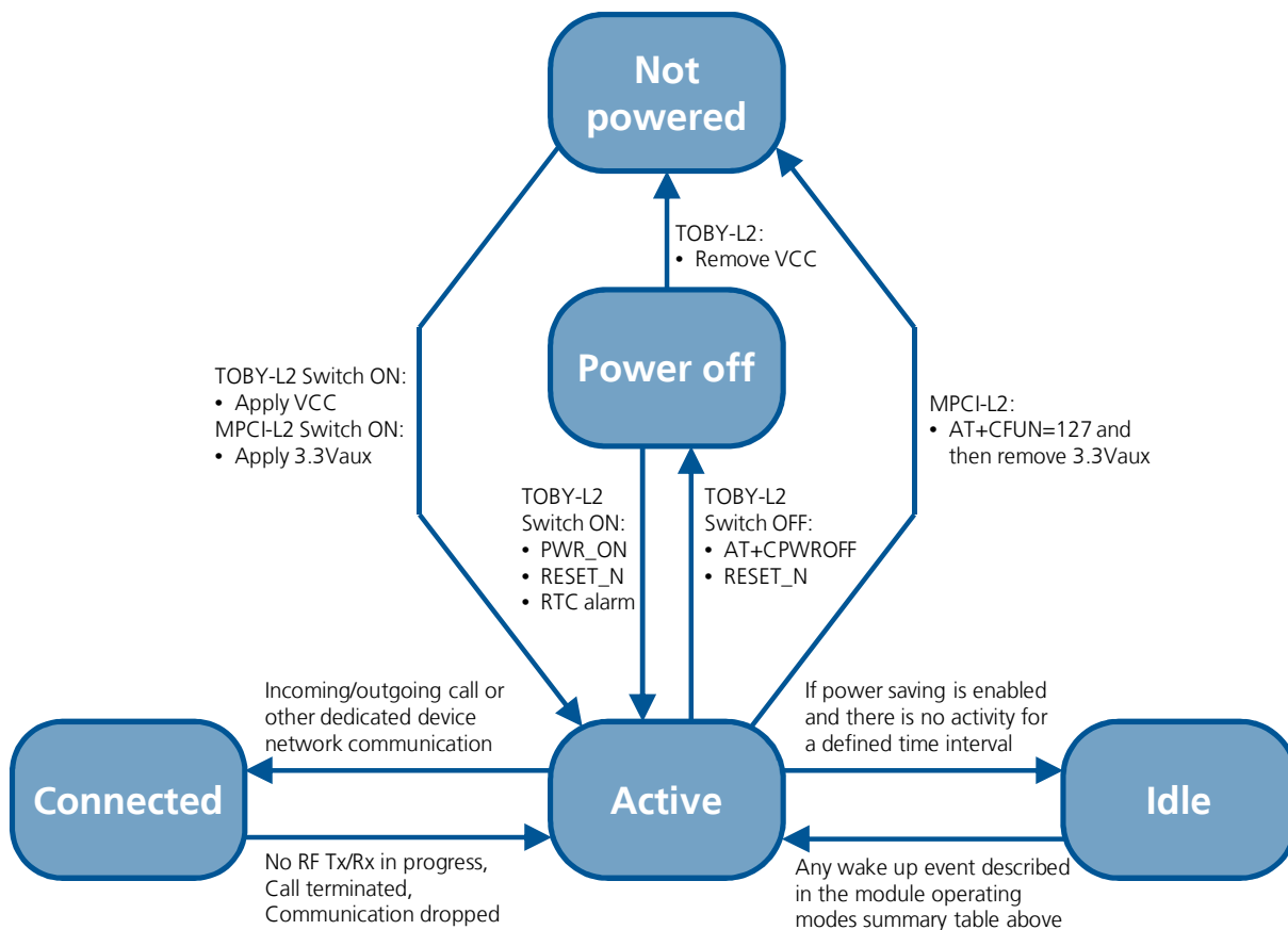
Figure 3: TOBY-L2 and MPC1-L2 series modules operating modes transition
