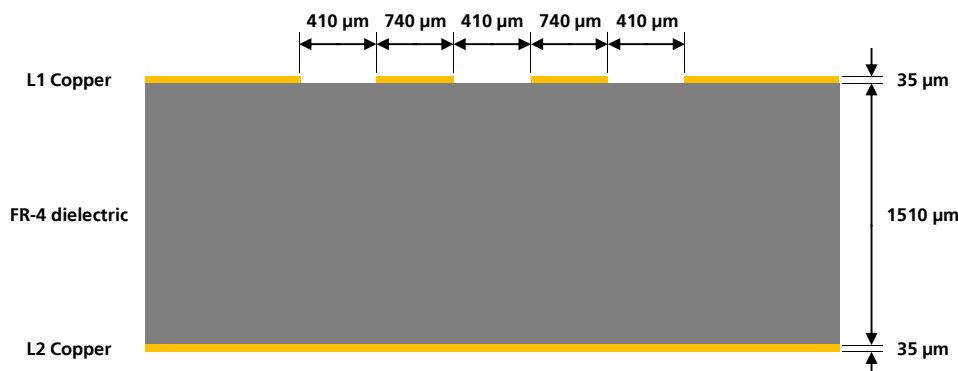
Figure 55: Example of USB line design, with Z_0 close to 90 \Omega and Z_{CM} close to 30 \Omega , for the described 2-layer board layout
