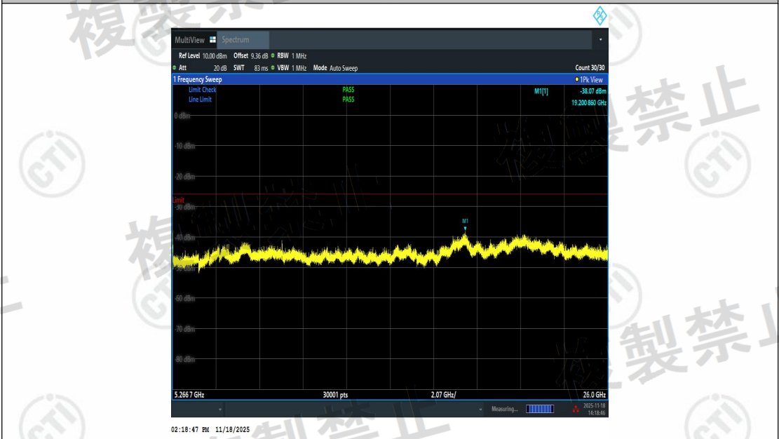
NTNV-11AX20SISO-Ant1-5240-5266.7~26000-PASS
