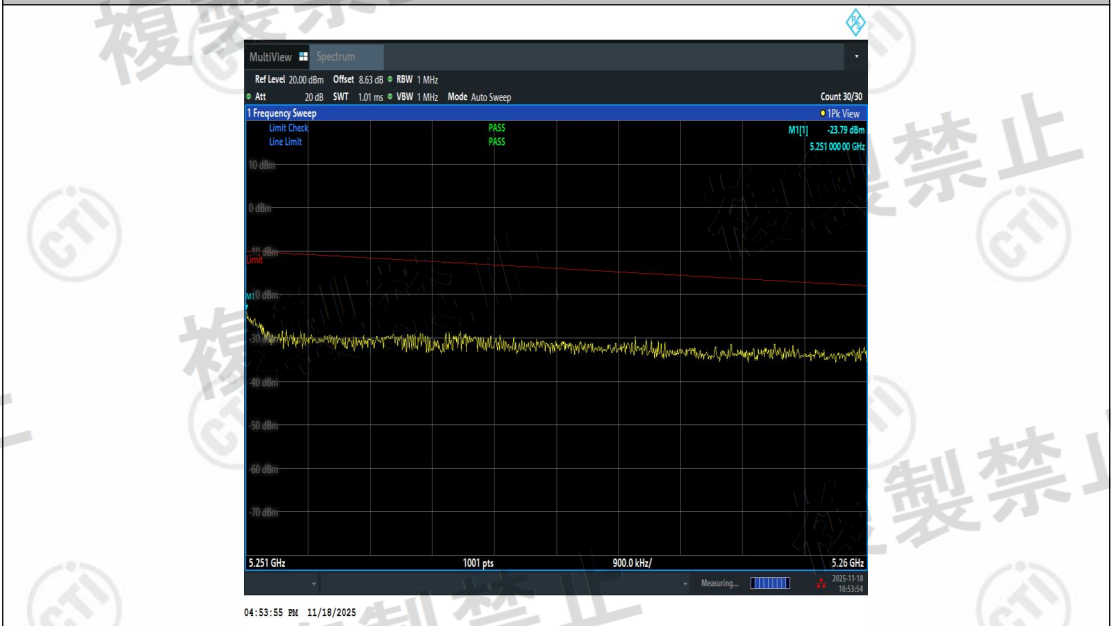
NTNV-11AX20SISO-Ant2-5240-5251~5260-PASS
