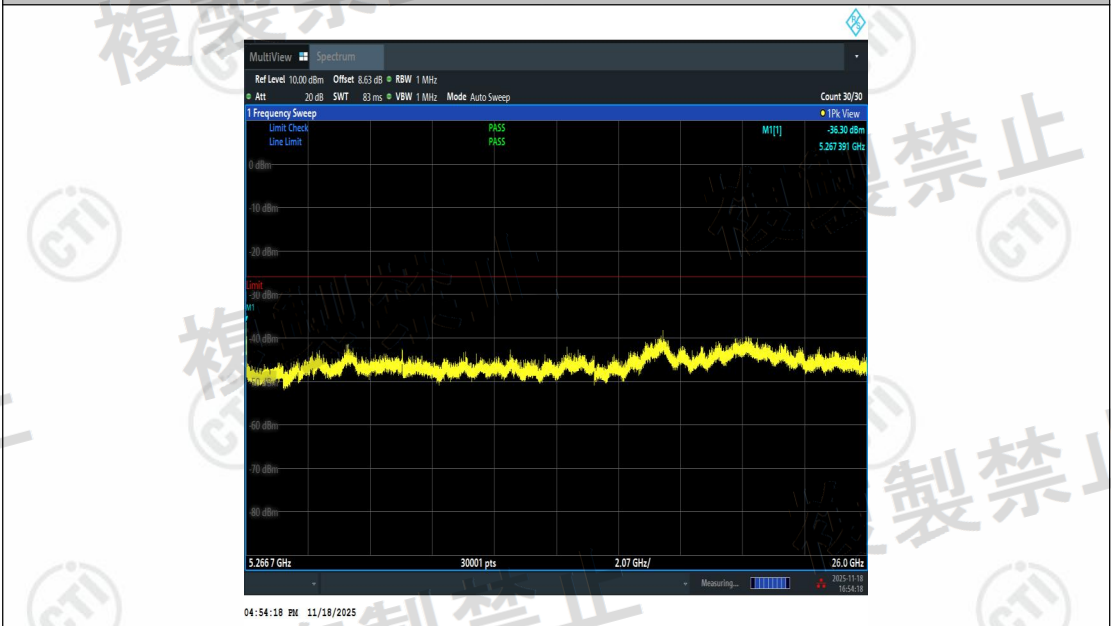
NTNV-11AX20SISO-Ant2-5240-5266.7~26000-PASS
