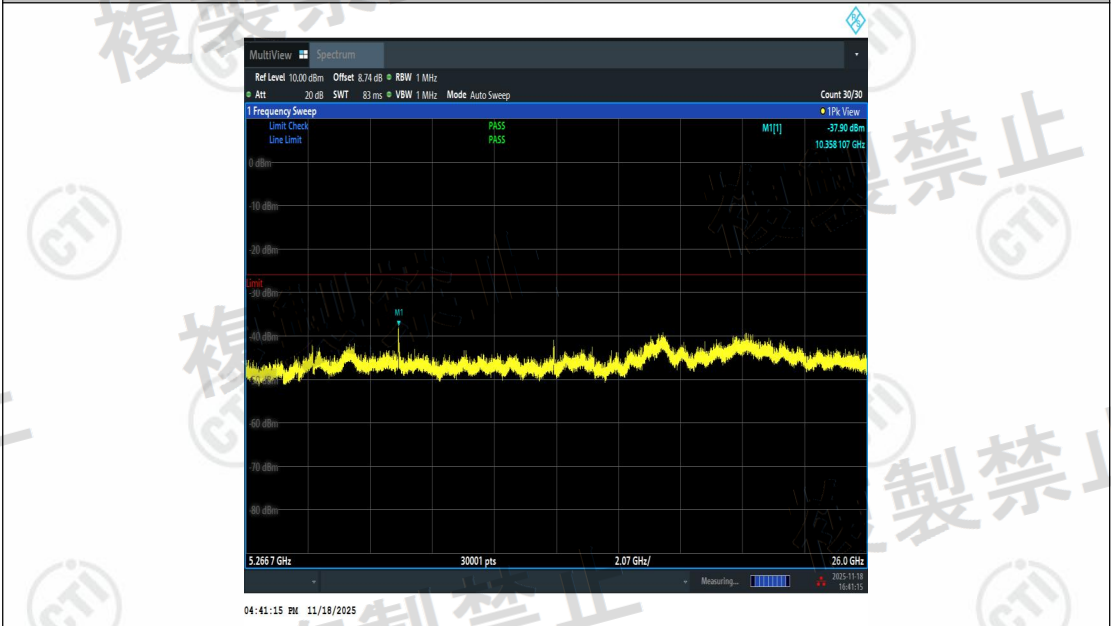
NTNV-11AX20SISO-Ant2-5180-5266.7~26000-PASS
