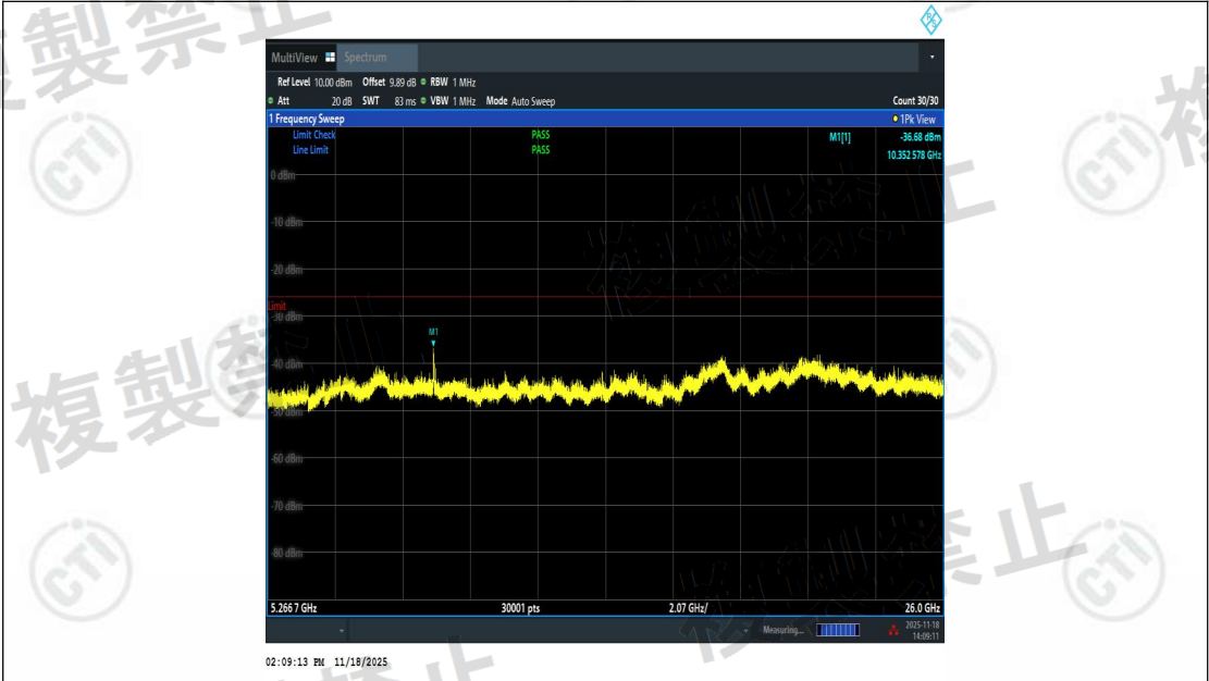
NTNV-11AX20SISO-Ant1-5180-5266.7~26000-PASS
