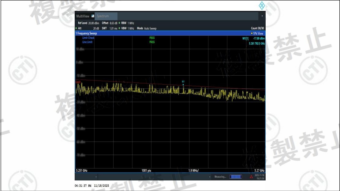
NTNV-11AC40SISO-Ant2-5230-5251~5270-See table below
