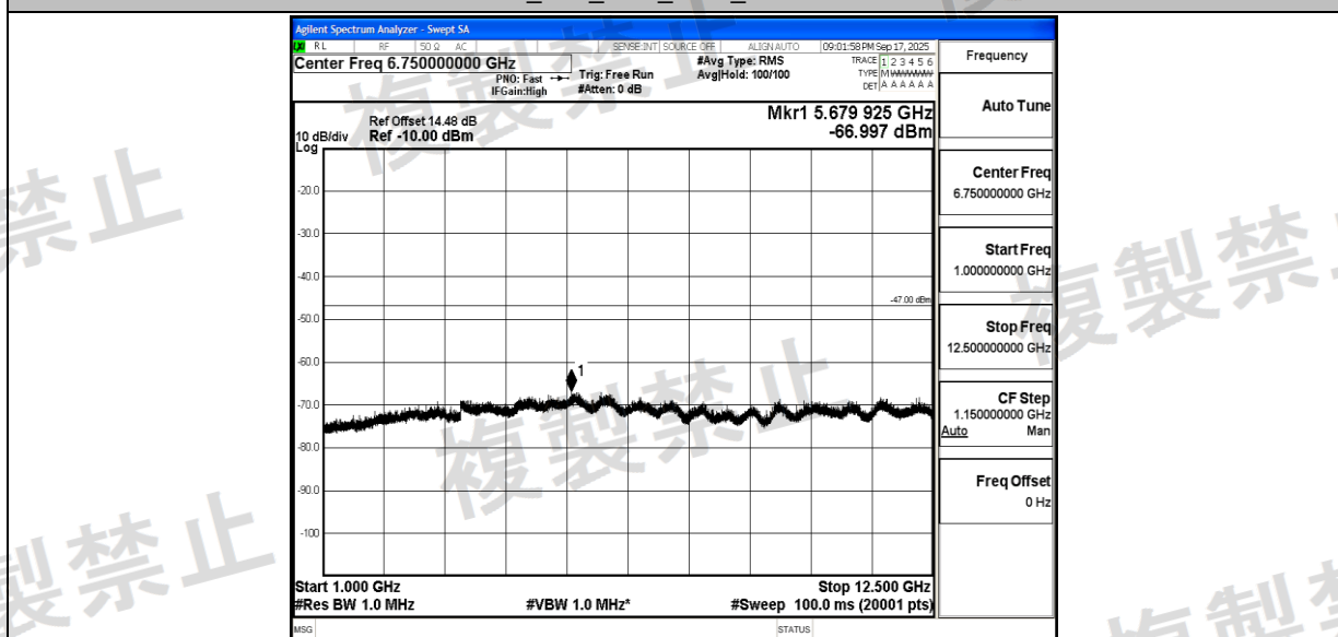
NTNV_11G_Ant1_2442_1000~12500
