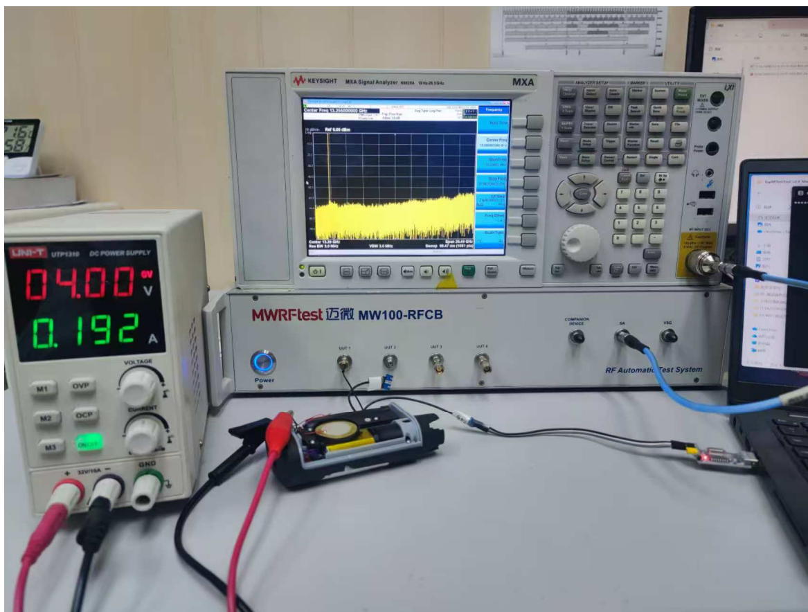
Picture 1 Test Setup
