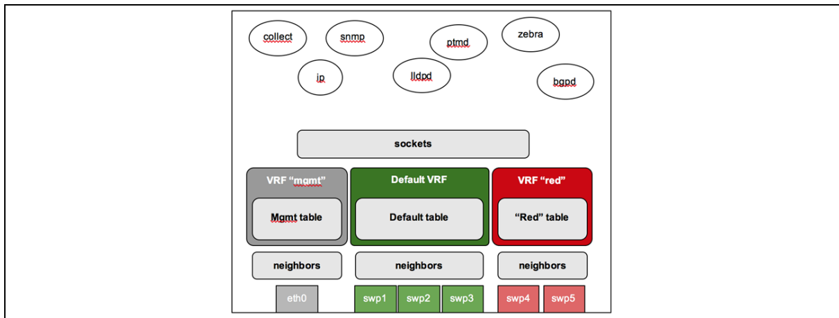
Figure 89: VRF architecture
