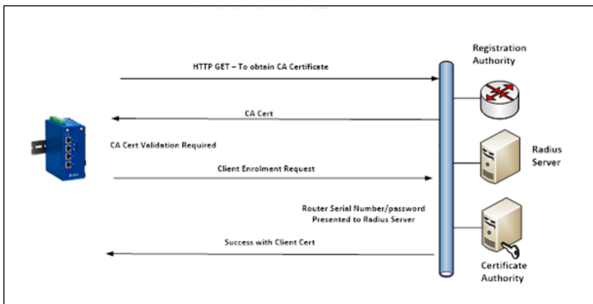
Figure 173: The SCEP process between router and PKI infrastructure
