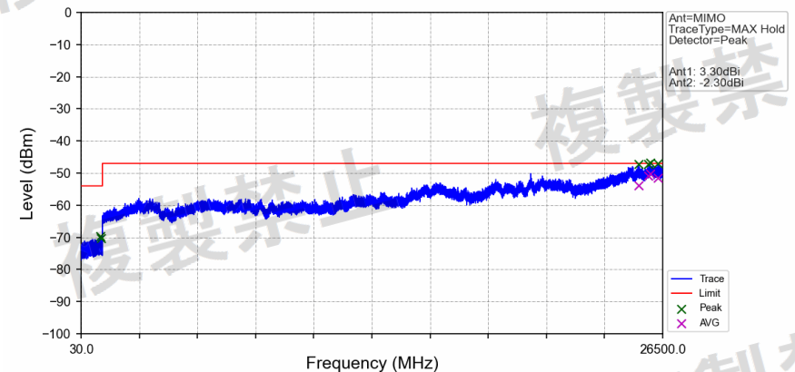
802.11ac(VHT20)_MCH_5600MHz_MIMO_NTNV
