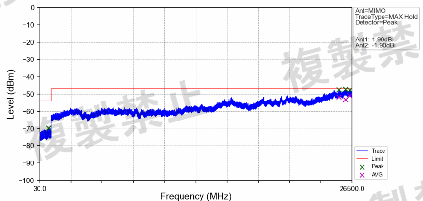
802.11n(HT20)_LCH_5260MHz_MIMO_NTNV
