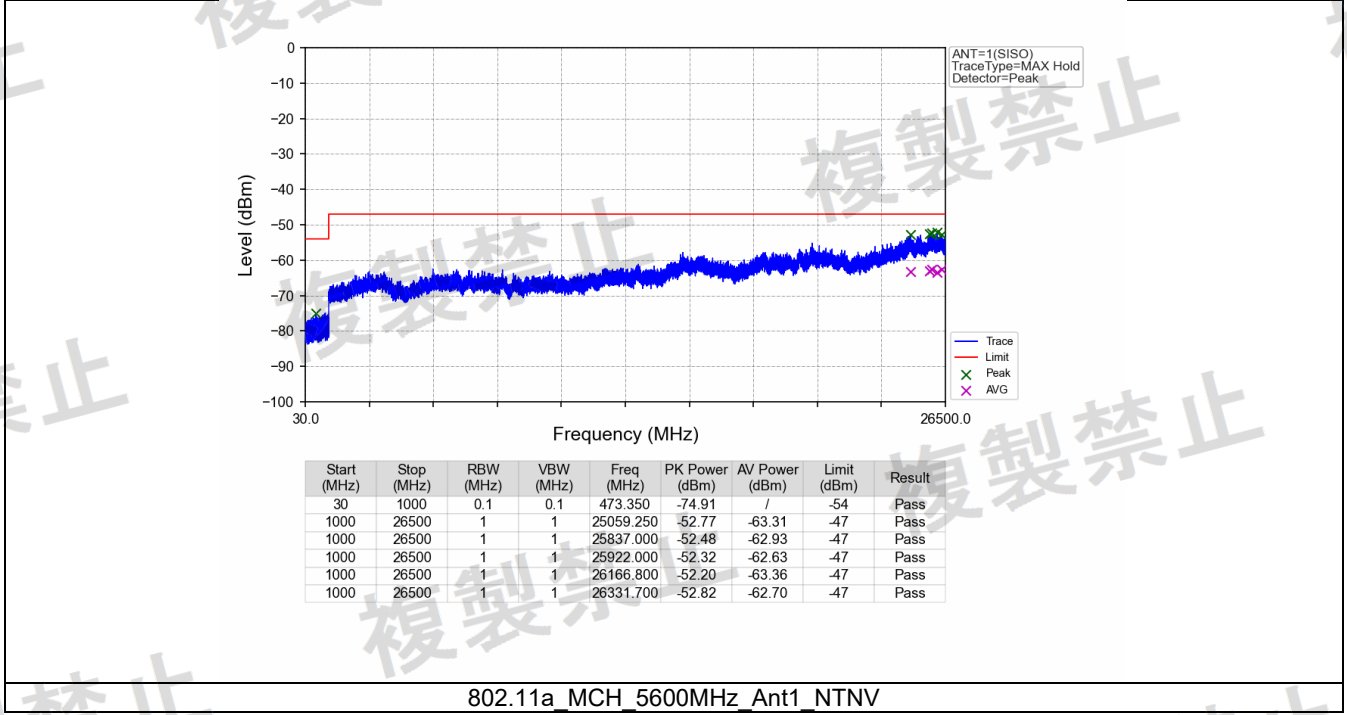
802.11a_MCH_5600MHz_Ant1_NTNV
