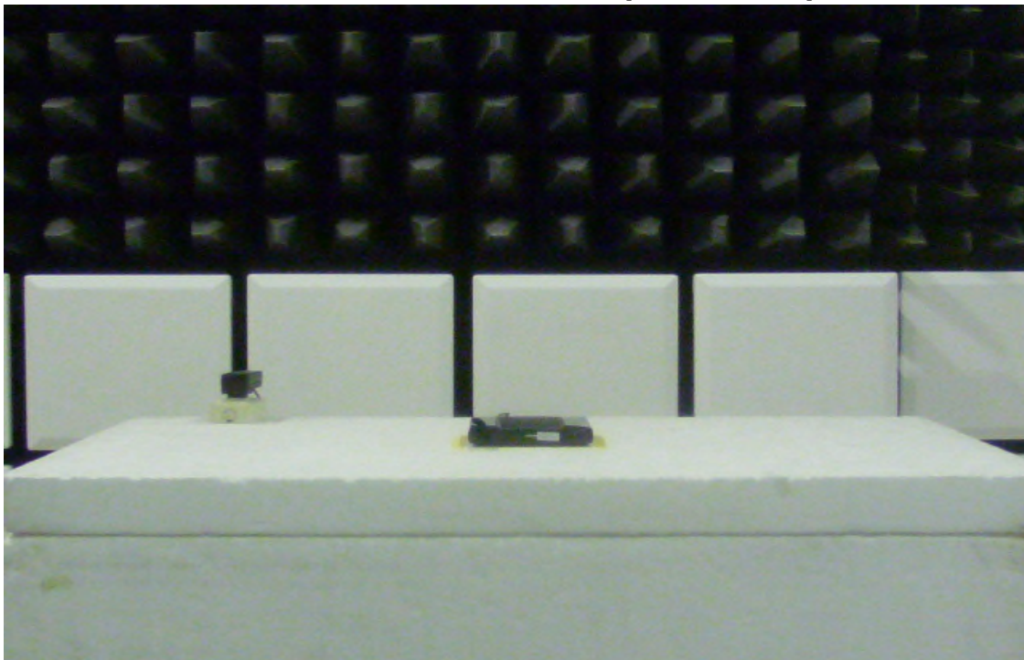
Radiated 量測之配置照片 (Front View)
