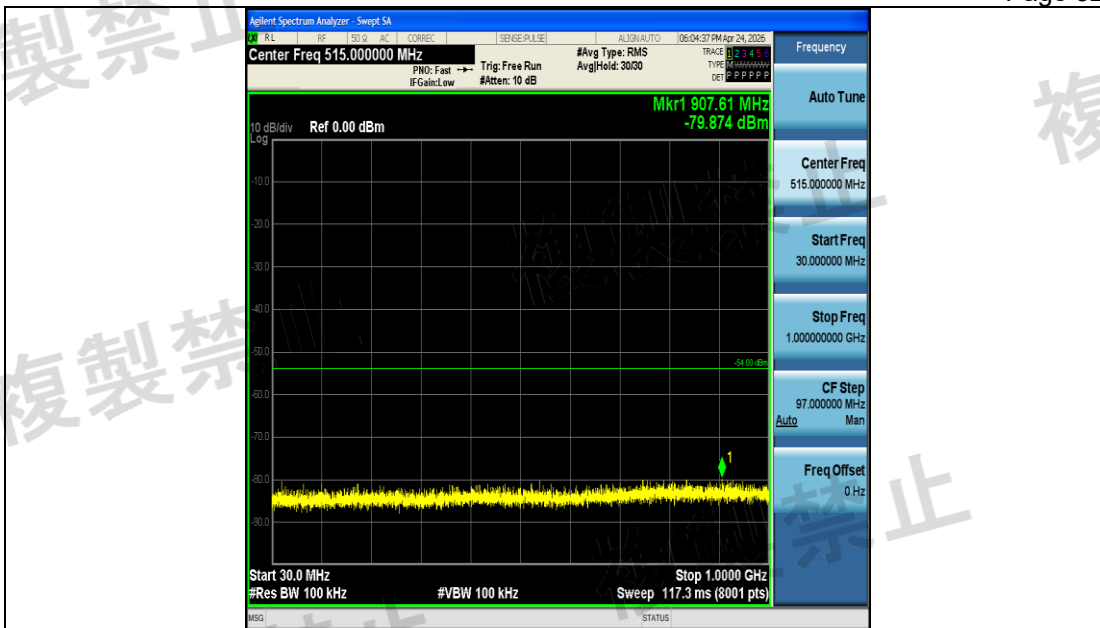
NTNV-11N40SISO-Ant1-5190-30~1000-PASS
