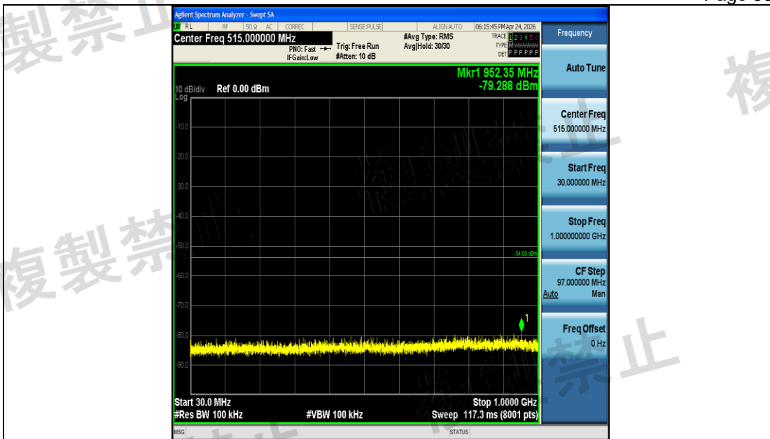
NTNV-11AC20SISO-Ant1-5280-30~1000-PASS
