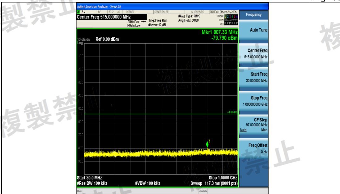
NTNV-11A-Ant1-5600-30~1000-PASS
