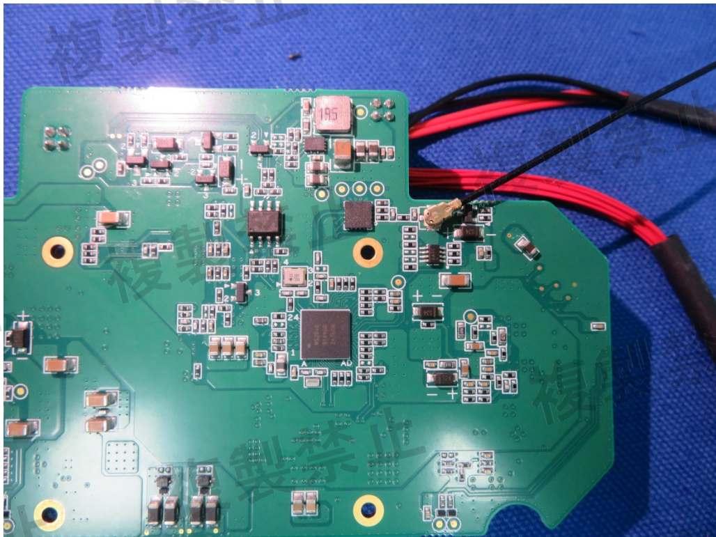
Picture 12 – Internal view
