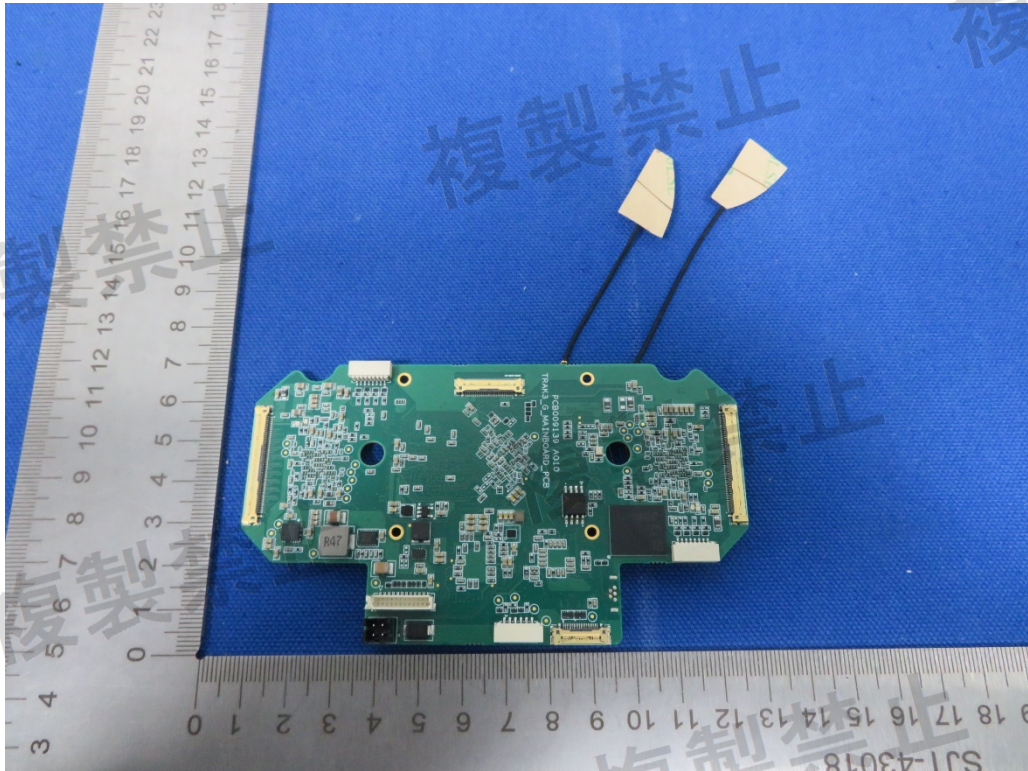
Picture 5 – Internal view
