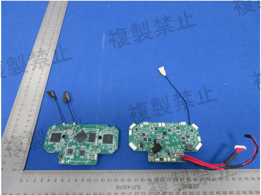
Picture 3 – Internal view
