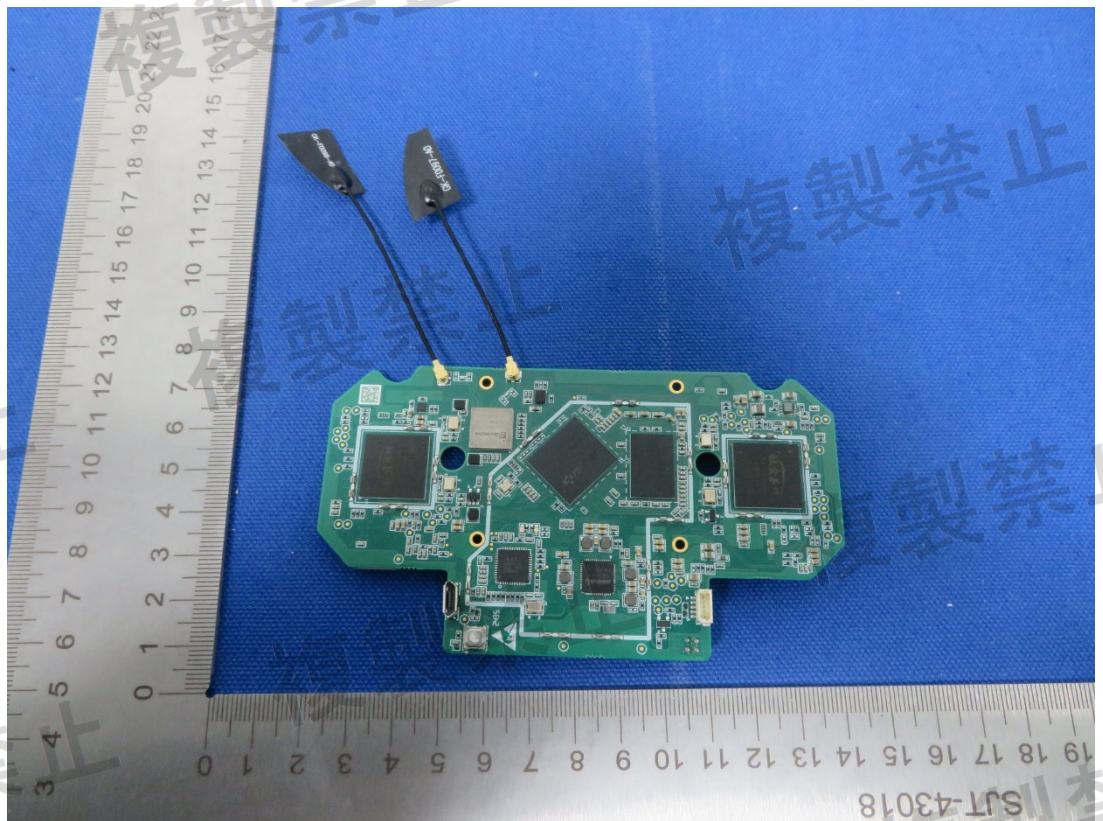
Picture 4 – Internal view
