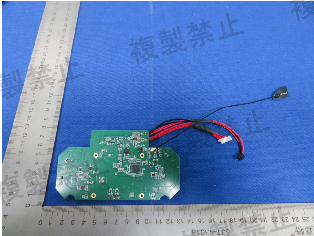
Picture 11 – Internal view
