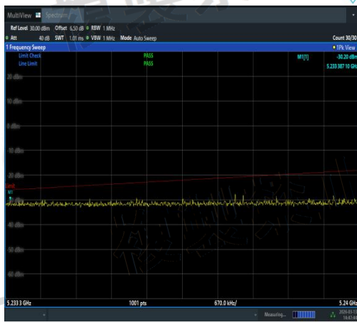
NTNV-11AX20SISO-Ant2-5260-5233.3~5240-PA SS
