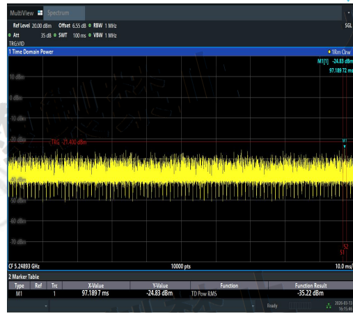
NTNV-11AX20SISO-Ant3-5260-5240~5249-PAS
