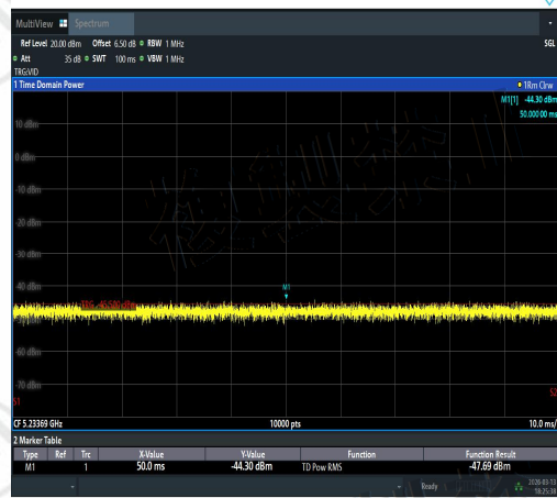
NTNV-11AC20MIMO-Ant1-5320-5233.3~5240-P ASS
