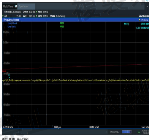
NTNV-11AC40SISO-Ant2-5310-5221.6~5230-PA SS
