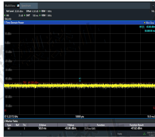
NTNV-11AC40SISO-Ant1-5310-5221.6~5230-PA SS
