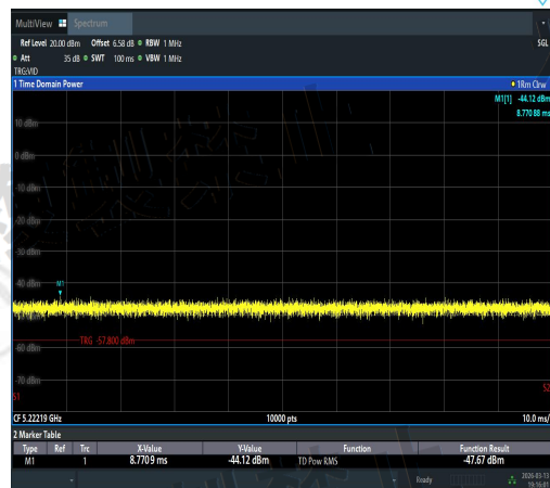
NTNV-11AC40MIMO-Ant3-5310-5221.6~5230-P ASS
