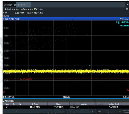
NTNV-11AC20MIMO-Ant3-5260-5233.3~5240-P ASS
