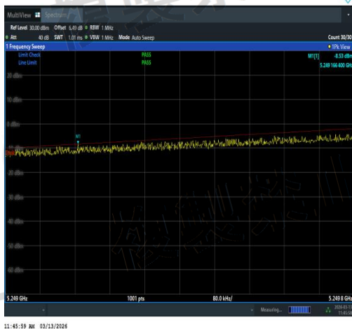
NTNV-11AX20SISO-Ant1-5260-5249~5249.8-PA
