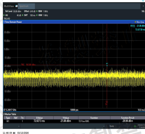
NTNV-11AX20SISO-Ant1-5260-5249~5249.8-PA
