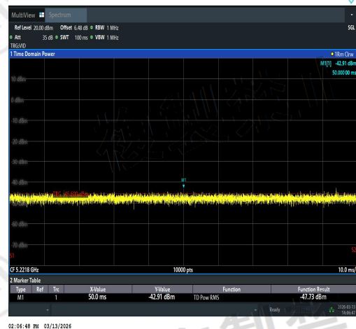
NTNV-11AC40SISO-Ant2-5310-5221.6~5230-PA SS
