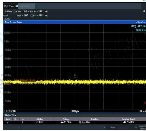
NTNV-11AC20MIMO-Ant1-5320-5233.3~5240-P ASS
