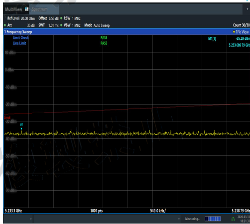
NTNV-11AC20MIMO-Ant3-5300-5233.3~5240-P ASS
