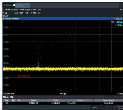
NTNV-11AC20MIMO-Ant1-5260-5233.3~5240-P ASS
