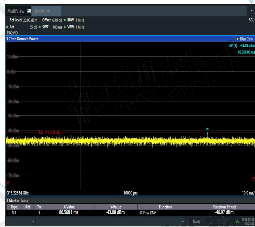
NTNV-11AC40SISO-Ant1-5270-5221.6~5230-PA
