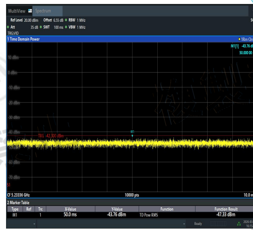
NTNV-11AX20SISO-Ant2-5260-5233.3~5240-PA SS
