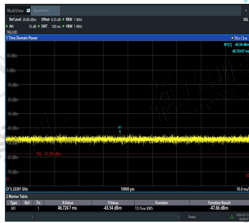
NTNV-11AC20MIMO-Ant1-5260-5233.3~5240-P ASS
