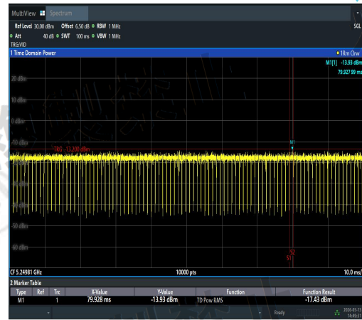
NTNV-11AX20SISO-Ant2-5260-5249.8~5250-PA
