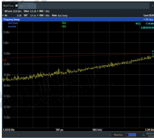
NTNV-11AX20SISO-Ant3-5260-5240~5249-PAS
