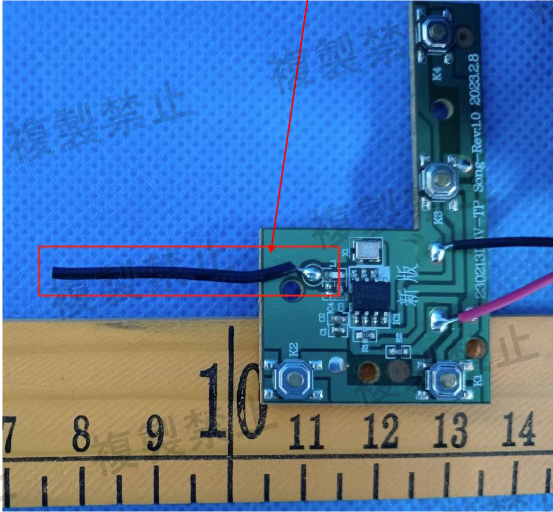
wireless antenna
