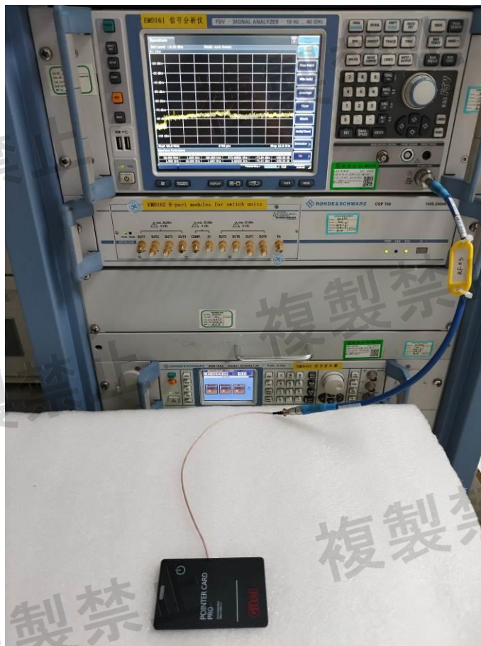
Measurement Test Set Up
