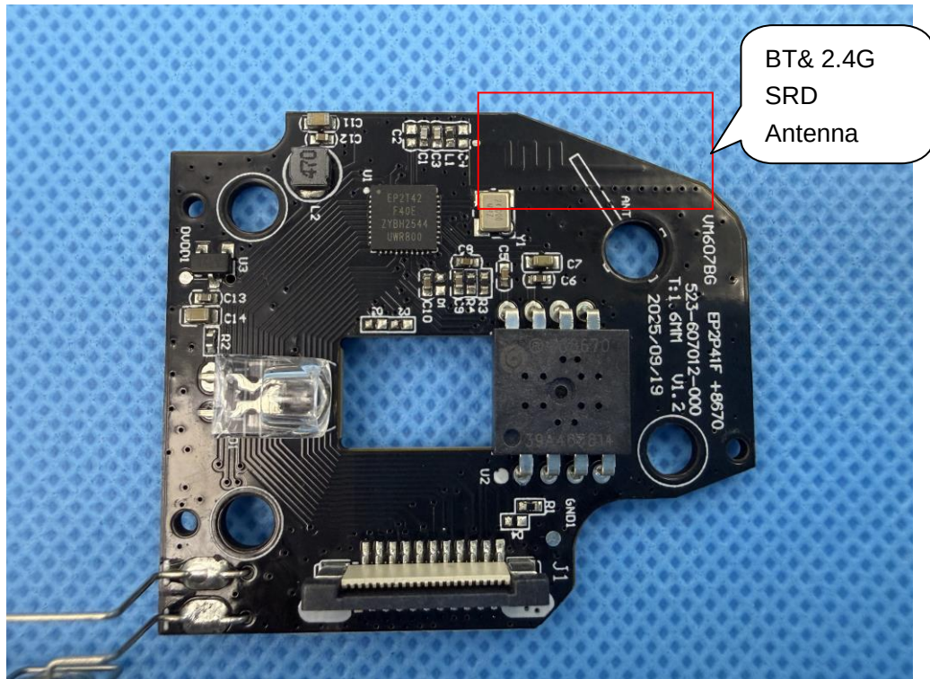
INTERNAL VIEW OF EUT (FIGURE 7)
