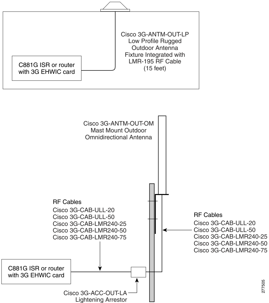
Figure 7 Antenna Options
