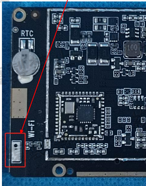
View of wireless antenna
