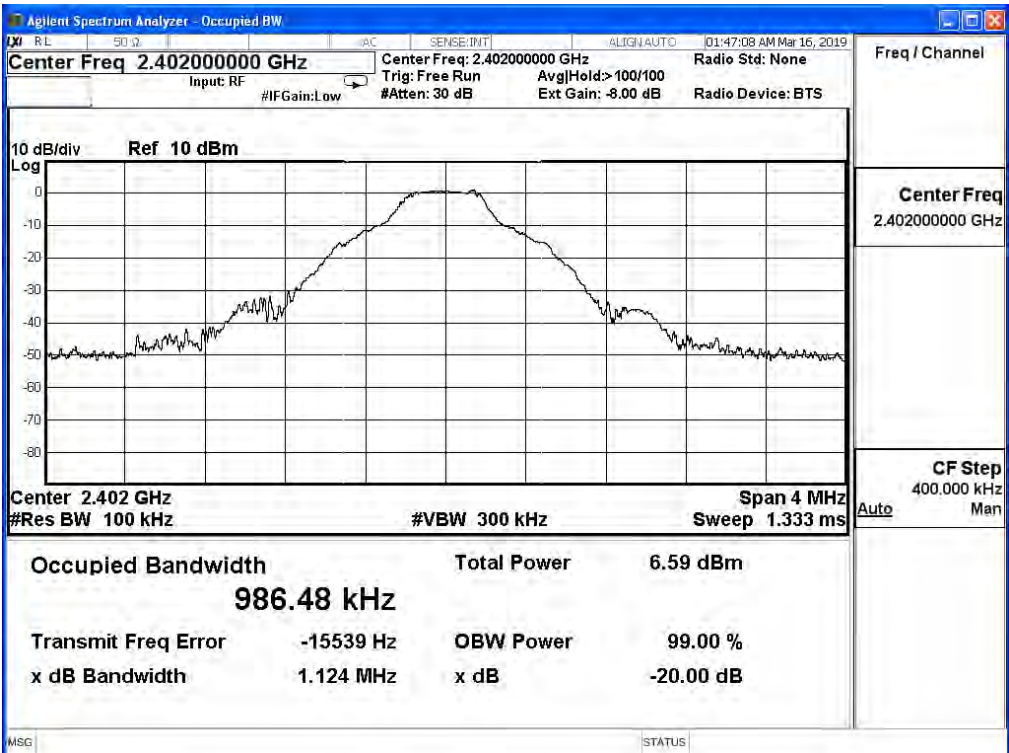
Channel 00
