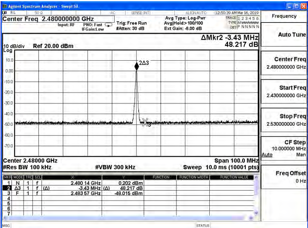
Channel 78
