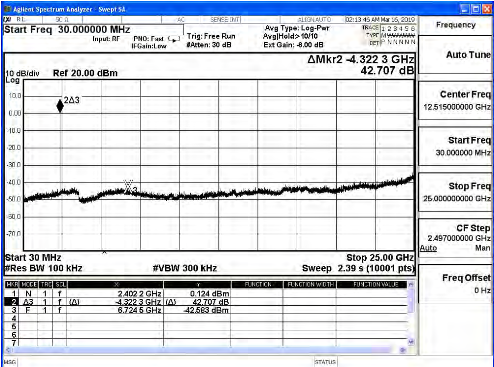
Channel 39 (30MHz-25GHz)-8-DPSK
