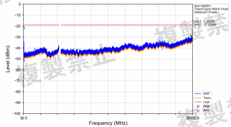
802.11n(HT40)_LCH_5510MHz_MIMO_NTNV
