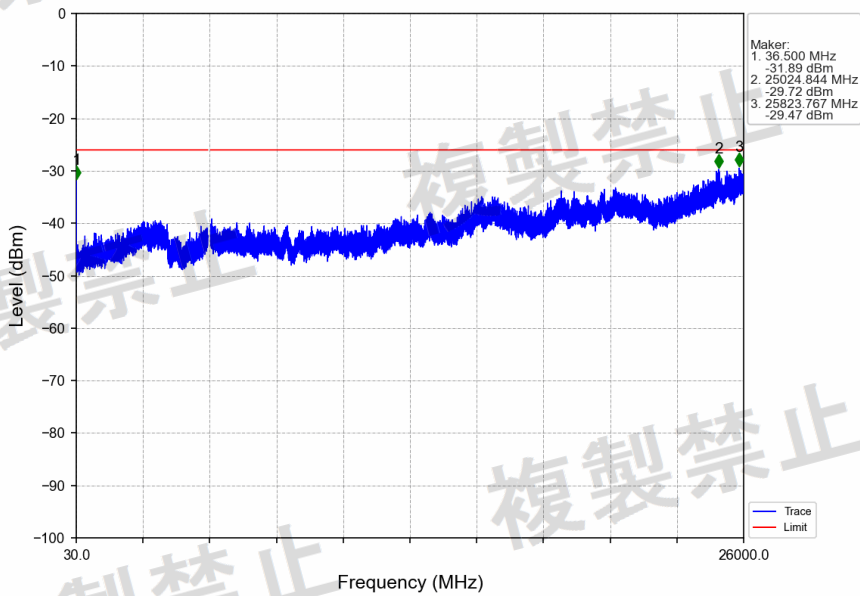
802.11ax(HEW20)_MCH_5200MHz_SU_ / Ant2_NTNV
