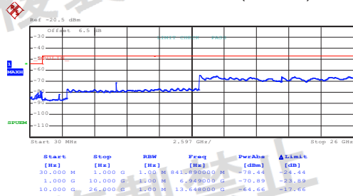
802.11n-HT20 (Band 1)
