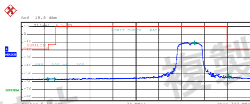
Middle channel
