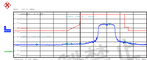
Lowest channel
