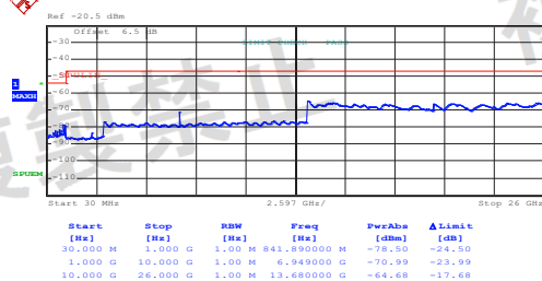
802.11ac-HT80 (Band 3)
