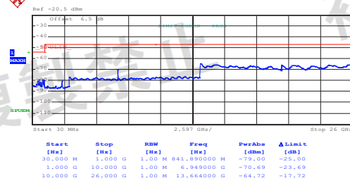
802.11n-HT20 (Band 3)
