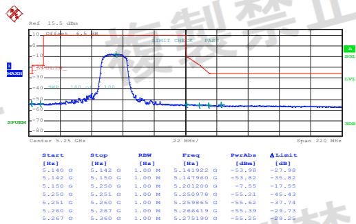
Lowest channel
