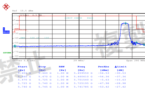
Middle channel
