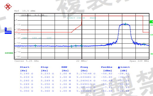
Middle channel
