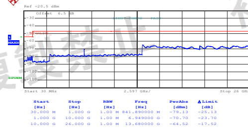
802.11ac-HT40 (Band 2)
