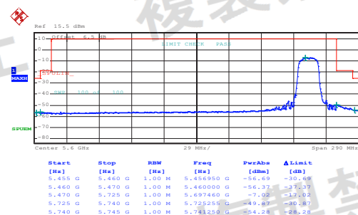
Middle channel
