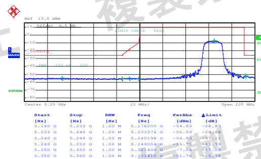
Middle channel
