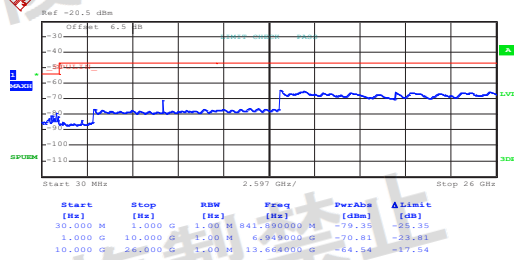
802.11ac-HT40 (Band 1)
