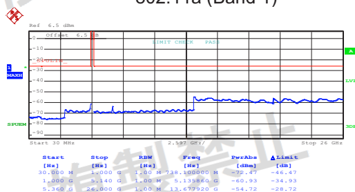
802.11a (Band 1)
