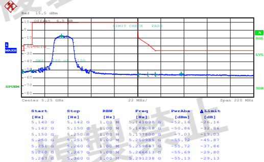
802.11ac-HT20 (Band 1)
