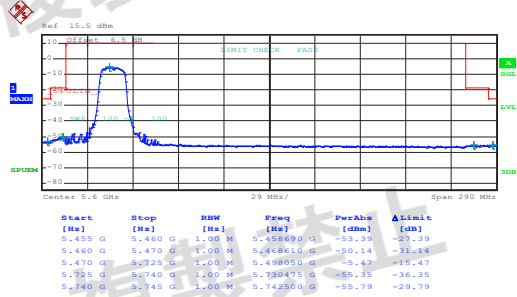
802.11a (Band 3)
