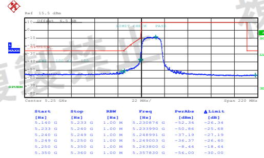
802.11n-HT20 (Band 2)
