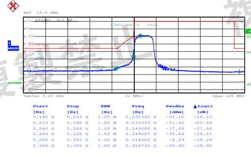
802.11ac-HT20 (Band 2)
