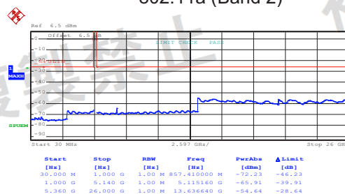
802.11a (Band 2)
