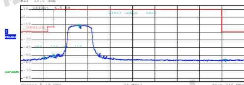
802.11ac-HT40 (Band 3)
