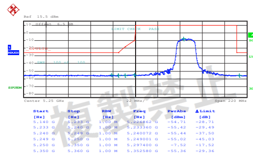
Lowest channel
