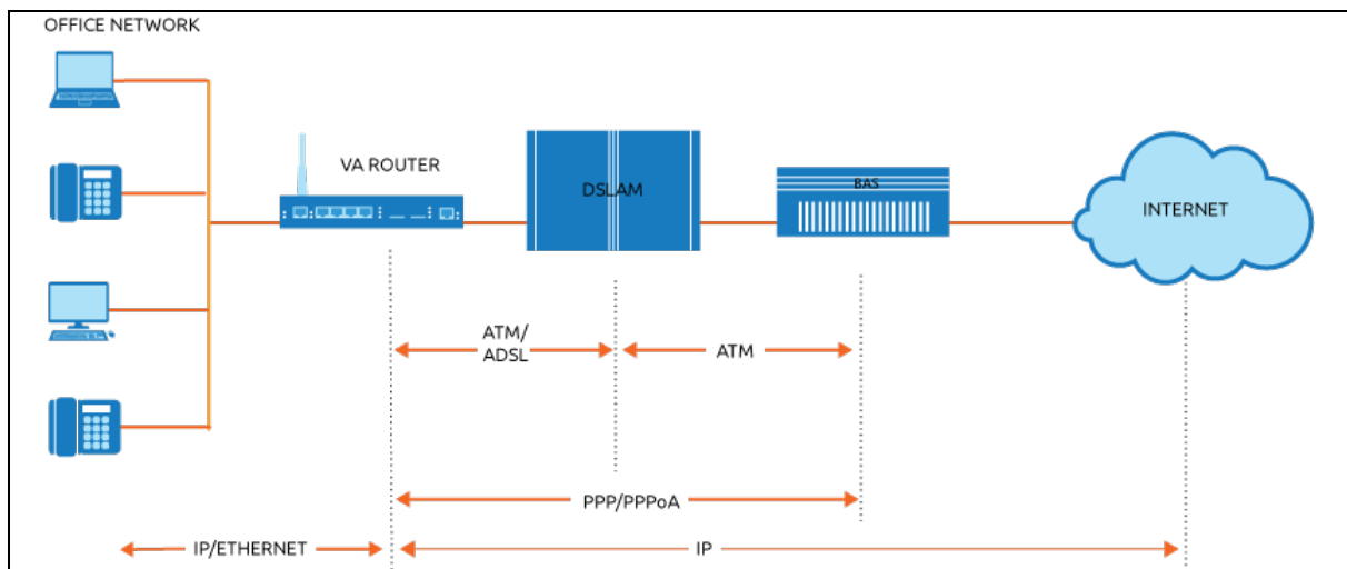
Figure 64: A routed ADSL connection over PPPoA
