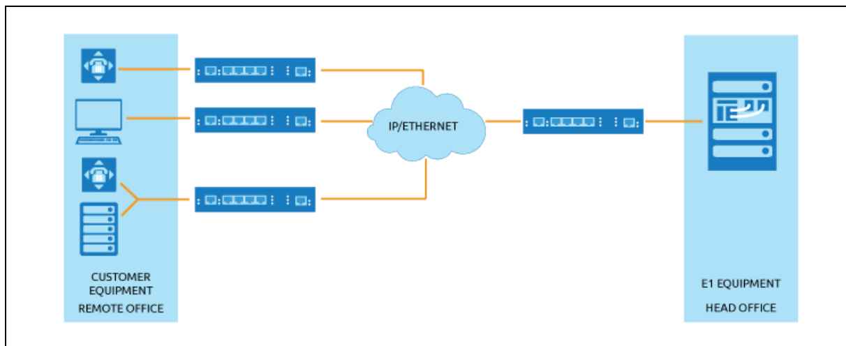
Figure 229: SAToP/CESoPSN P2MP architecture
