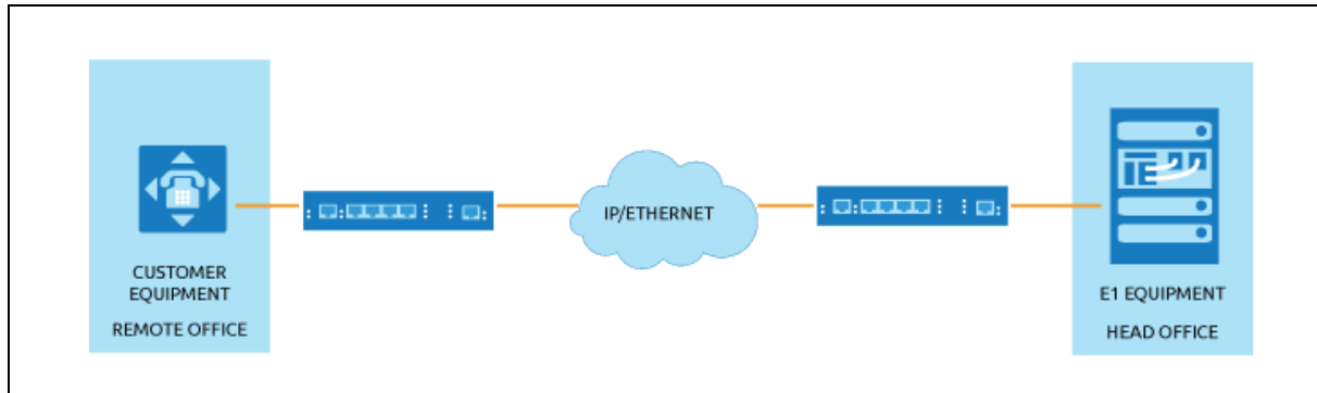
Figure 228: SAToP/CESoPSN P2P architecture
