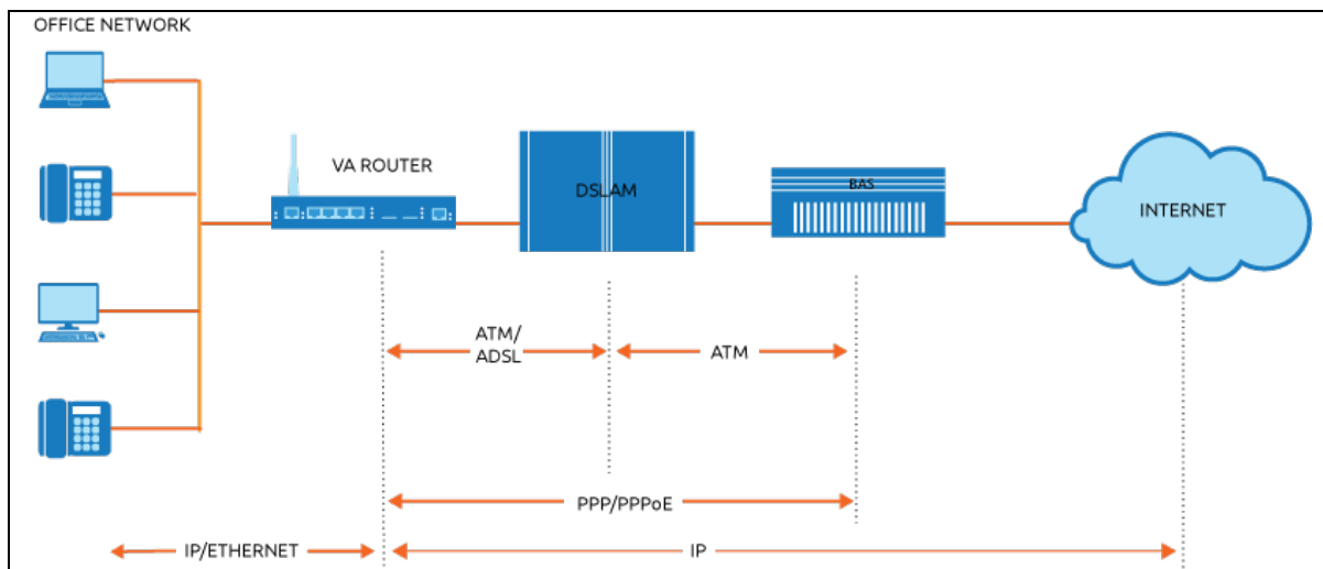
Figure 65: A routed ADSL connection over PPPoE
