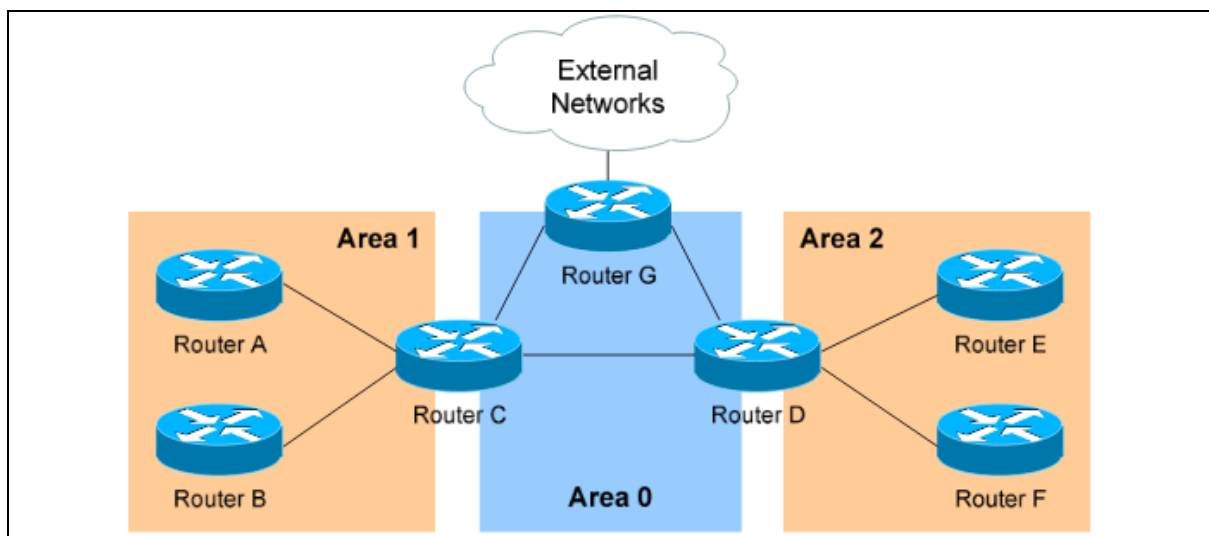
Figure 110: OSPF hierarchy
