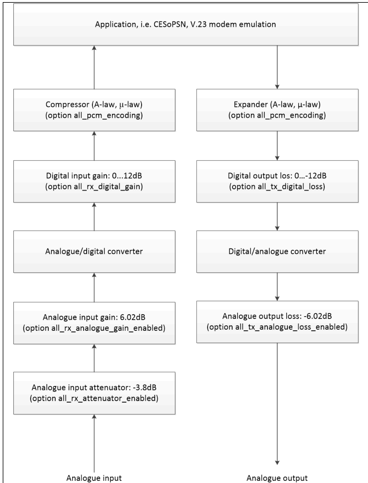
Figure 238: Gain and attenuation flow
