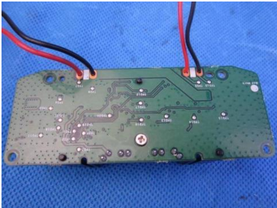
Protect PCB view 2
