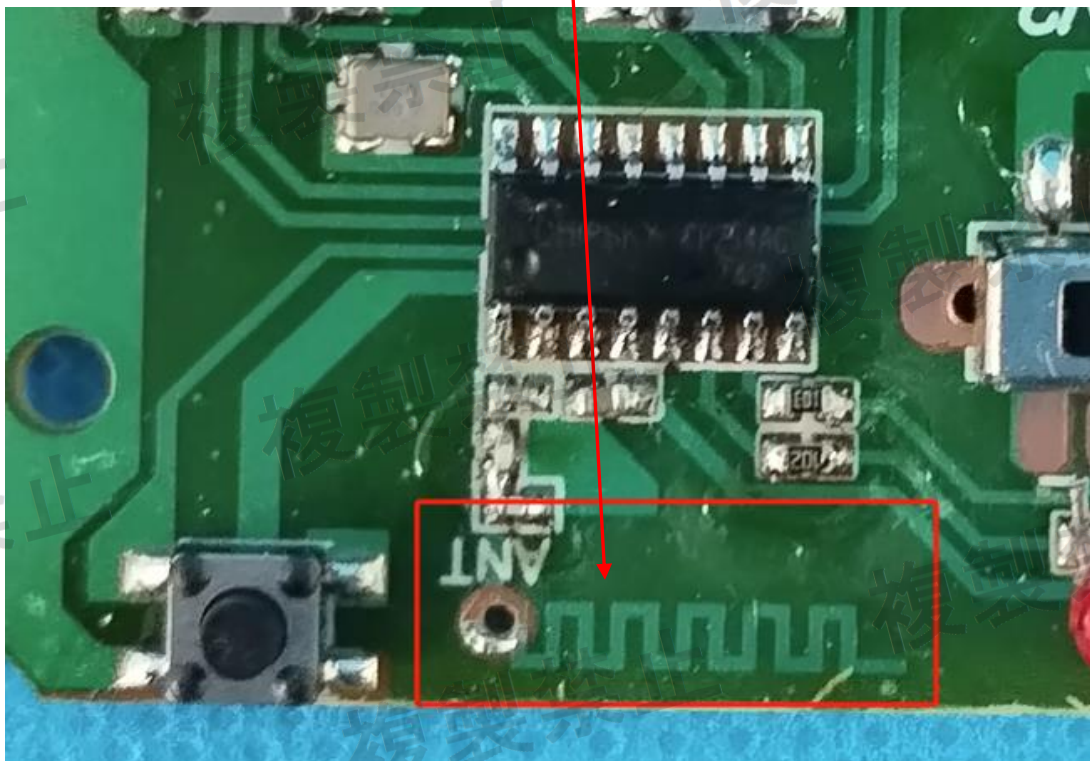
wireless antenna
