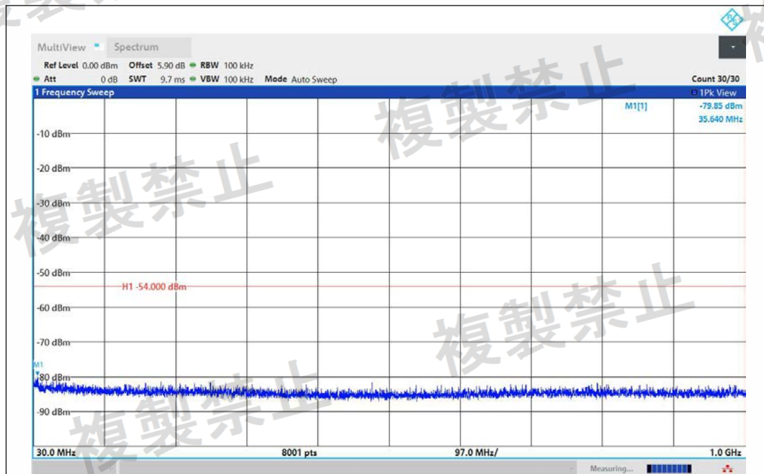
NTNV-11AX40MIMO-Ant1-2422-30~1000-PASS
