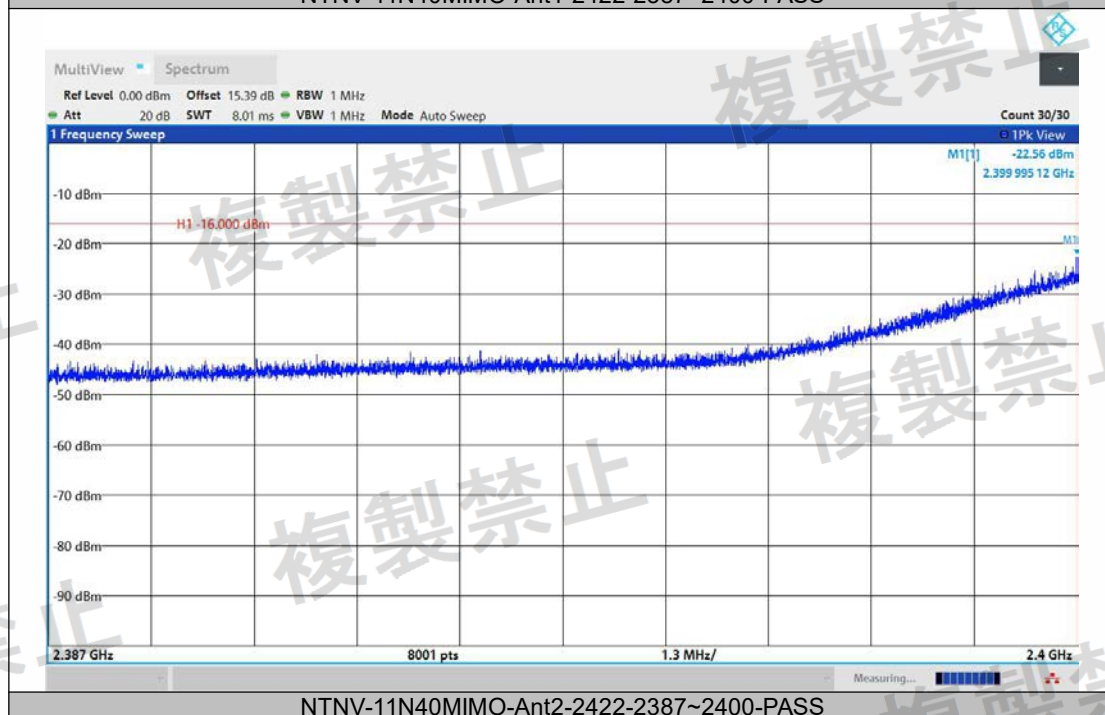
NTVN-11N40MIMO-Ant2-2422-2387~2400-PASS
