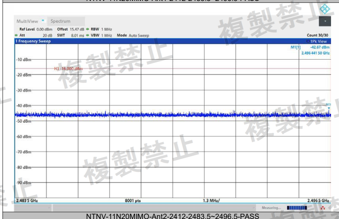
NTNV-11N20MIMO-Ant2-2412-2483.5~2496.5-PASS
