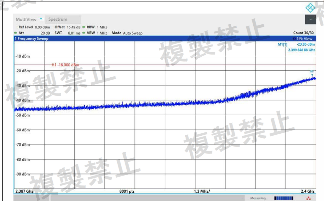
NTNV-11G-Ant1-2412-2387~2400-PASS
