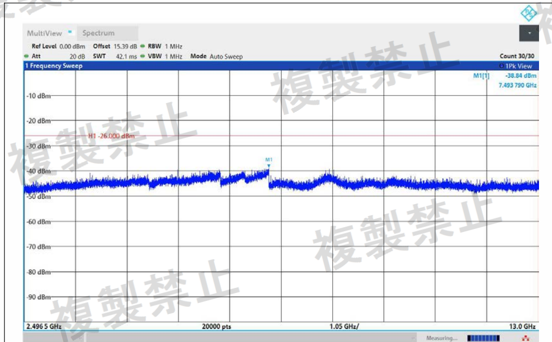
NTNV-11AX20MIMO-Ant1-2442-2496.5~13000-PASS
