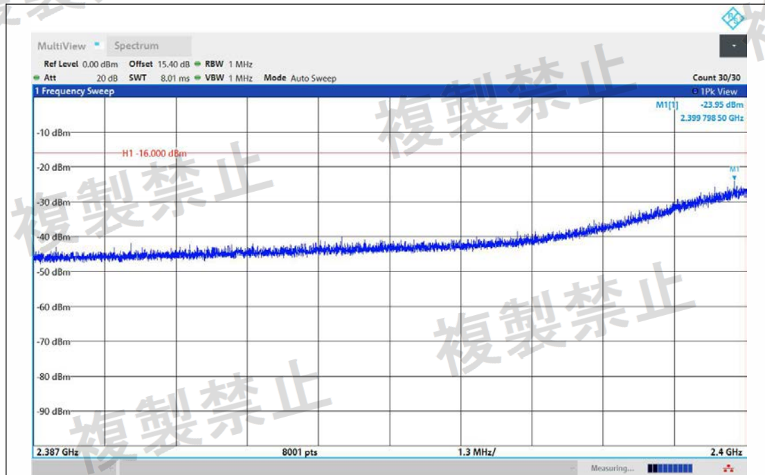
NTVN-11N40MIMO-Ant1-2422-2387~2400-PASS
