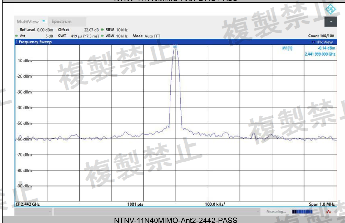
NTNV-11N40MIMO-Ant2-2442-PASS
