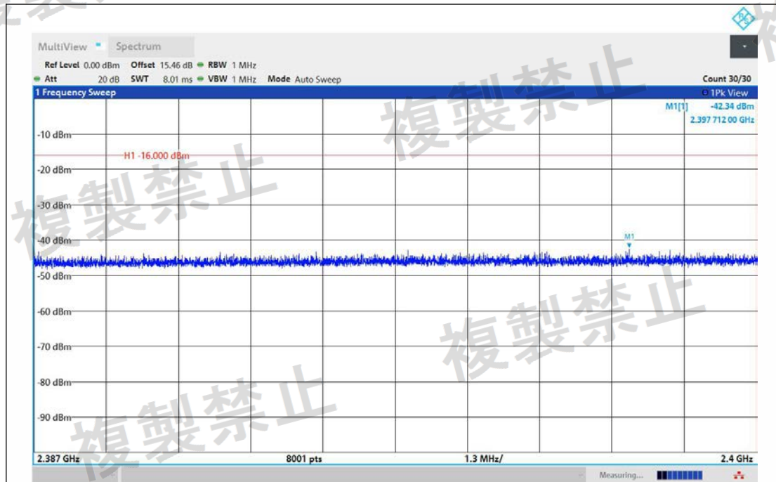
NTNV-11N40MIMO-Ant1-2462-2387~2400-PASS
