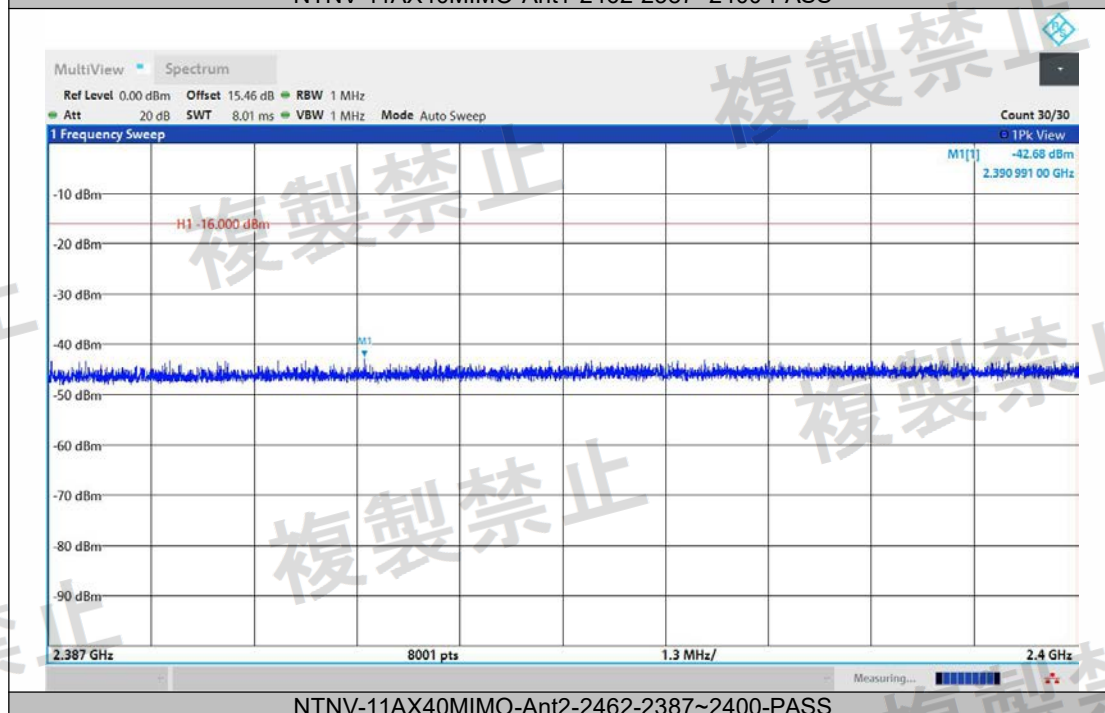
NTNV-11AX40MIMO-Ant2-2462-2387~2400-PASS
