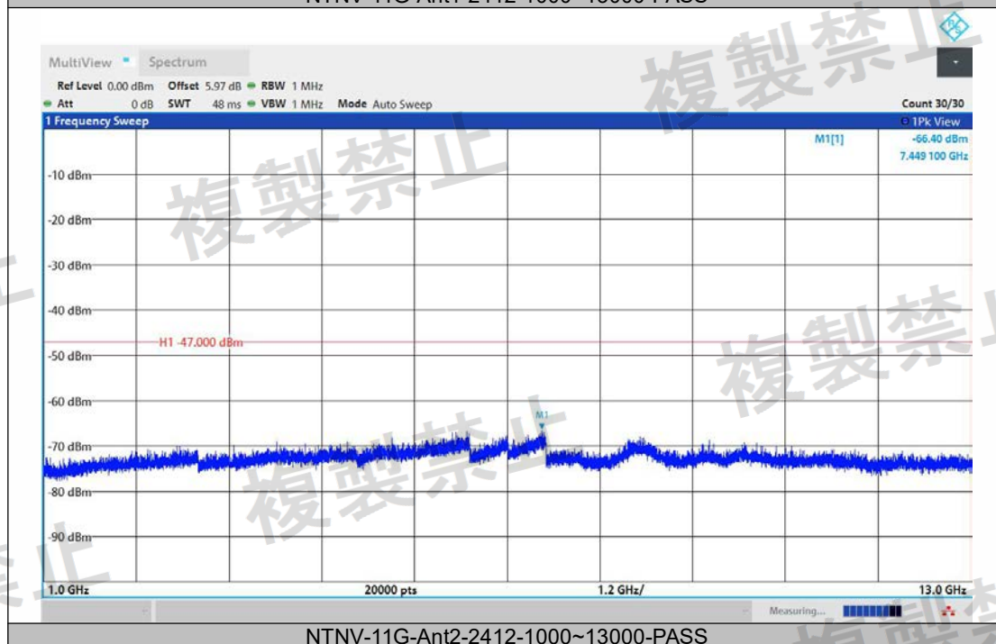
NTNV-11G-Ant2-2412-1000~13000-PASS
