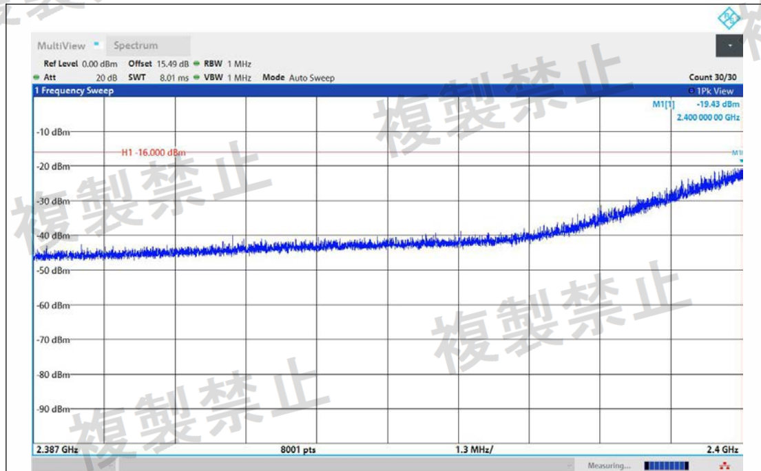
NTVN-11AX20MIMO-Ant1-2412-2387~2400-PASS
