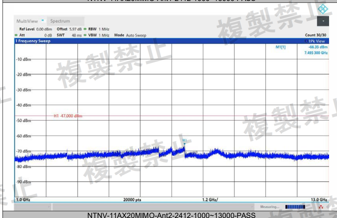
NTVN-11AX20MIMO-Ant2-2412-1000~13000-PASS
