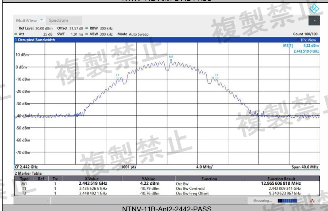
NTNV-11B-Ant2-2442-PASS
