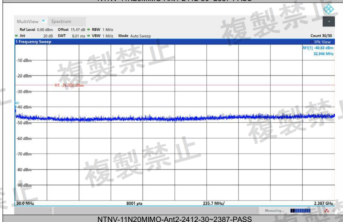
NTNV-11N20MIMO-Ant2-2412-30~2387-PASS
