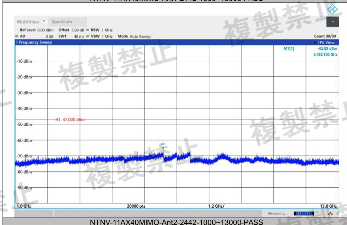
NTVN-11AX40MIMO-Ant2-2442-1000~13000-PASS
