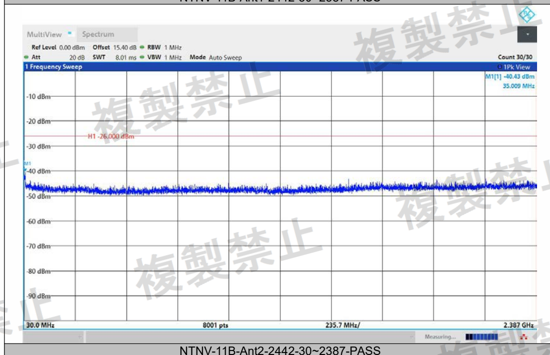
NTNV-11B-Ant2-2442-30~2387-PASS
