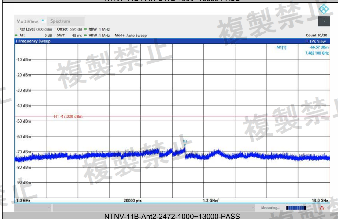
NTNV-11B-Ant2-2472-1000~13000-PASS
