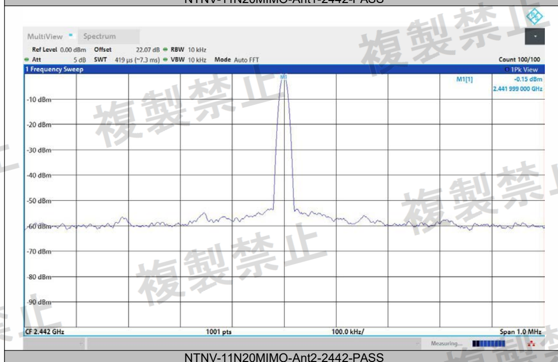
NTNV-11N20MIMO-Ant2-2442-PASS
