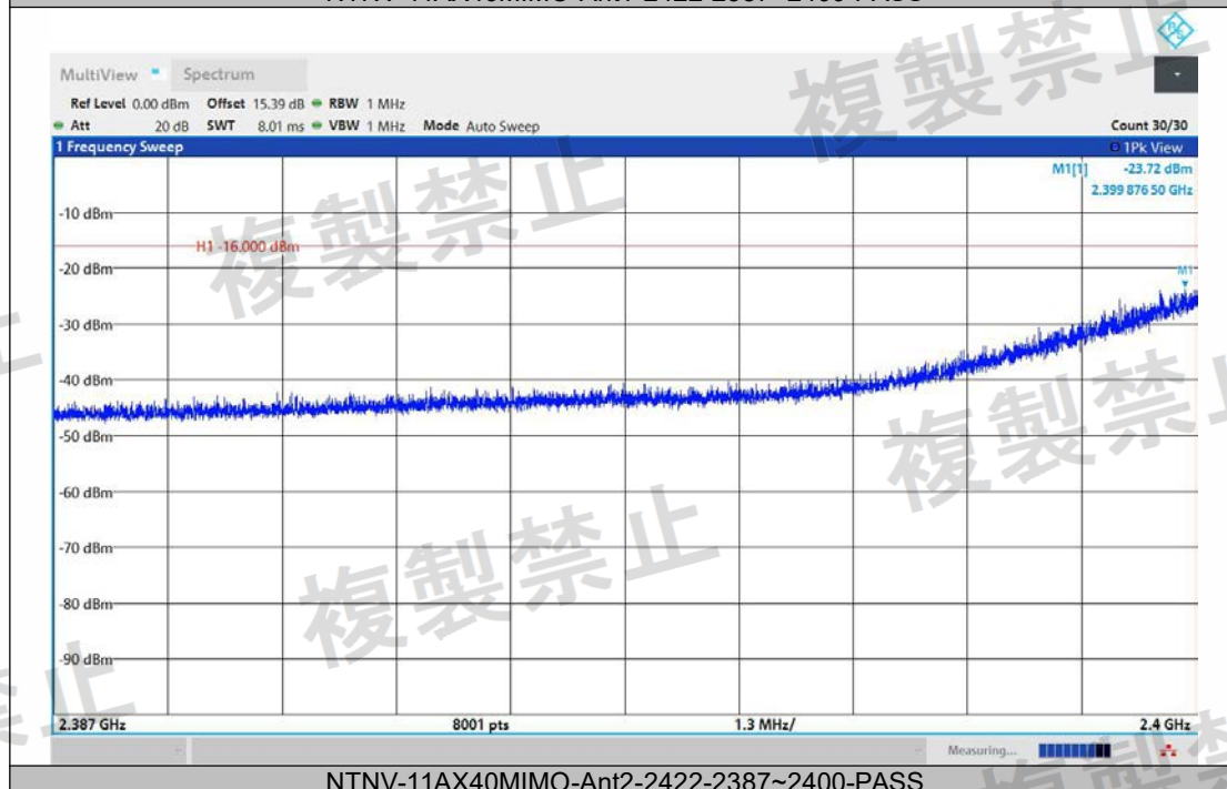
NTVN-11AX40MIMO-Ant2-2422-2387~2400-PASS
