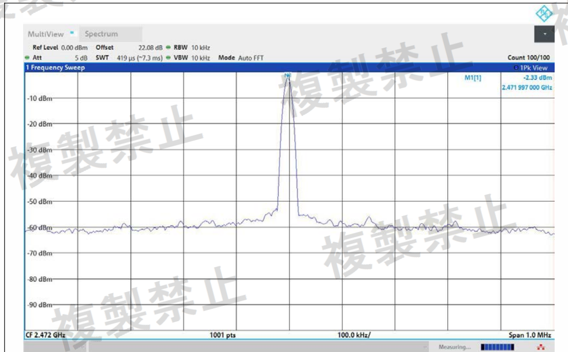
NTVN-11N20MIMO-Ant1-2472-PASS
