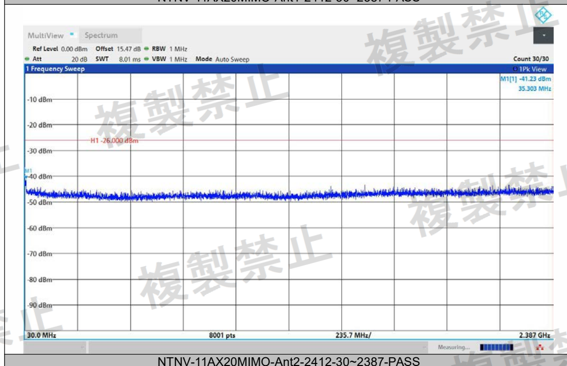
NTNV-11AX20MIMO-Ant2-2412-30~2387-PASS
