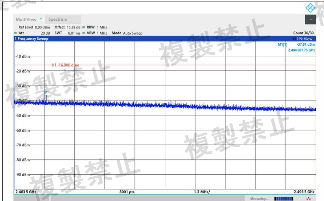
NTNV-11AX40MIMO-Ant1-2442-2483.5~2496.5-PASS
