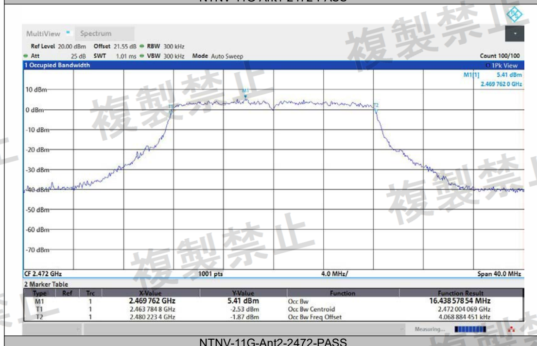
NTNV-11G-Ant2-2472-PASS
