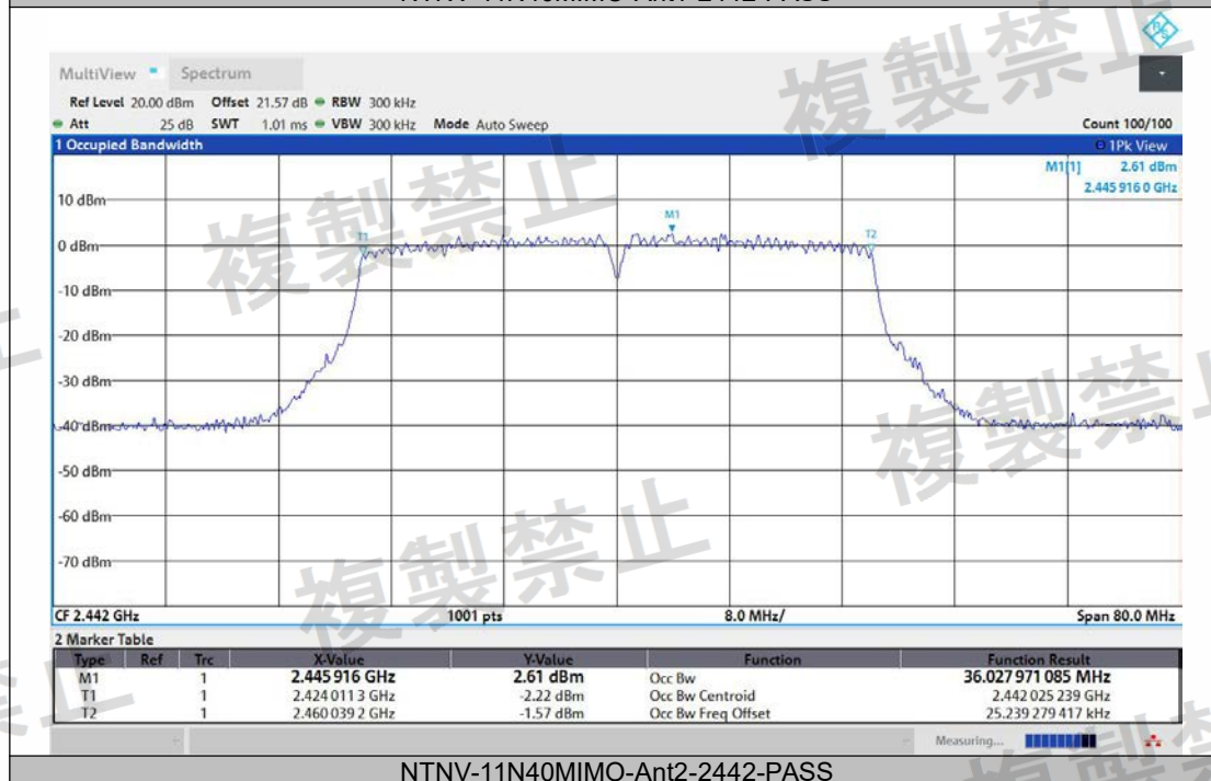
NTNV-11N40MIMO-Ant2-2442-PASS
