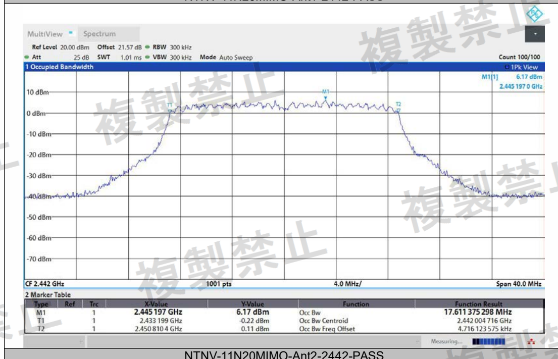
NTNV-11N20MIMO-Ant2-2442-PASS
