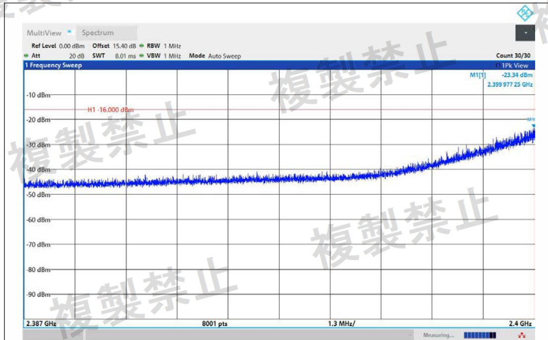
NTVN-11AX40MIMO-Ant1-2422-2387~2400-PASS
