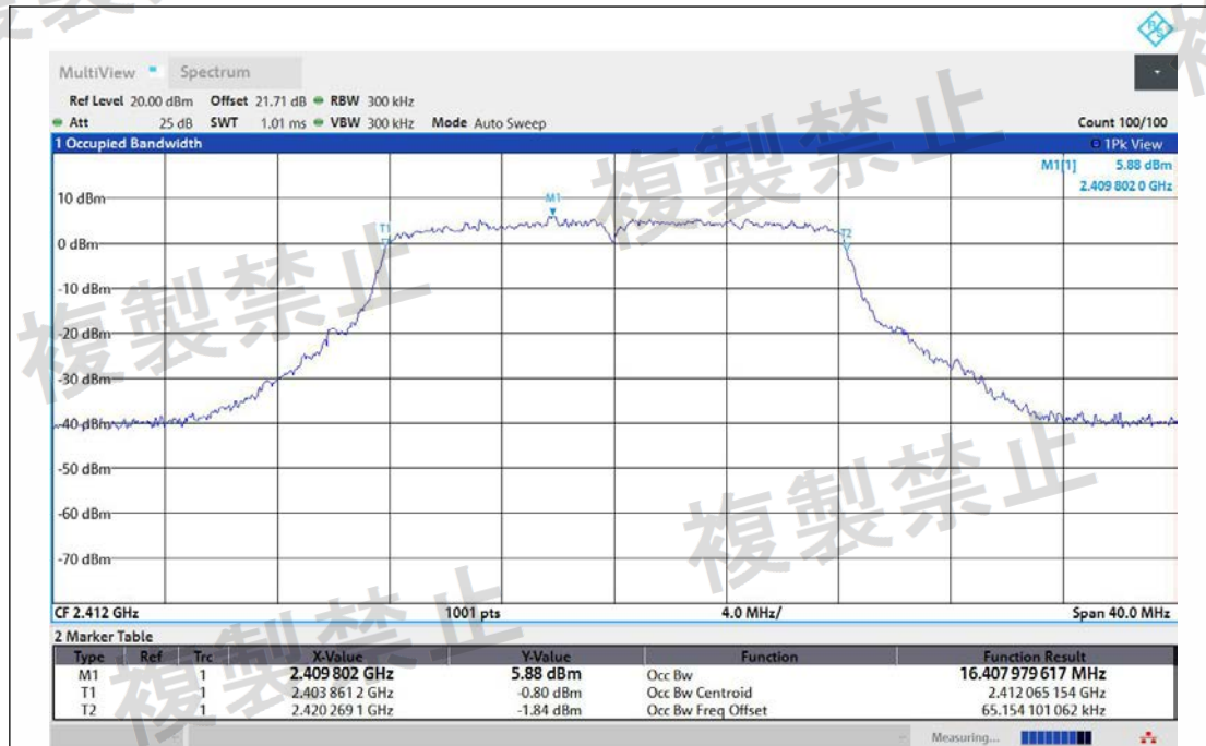
NTNV-11G-Ant1-2412-PASS
