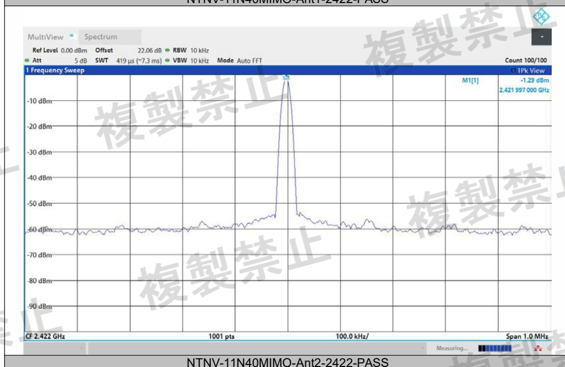
NTNV-11N40MIMO-Ant2-2422-PASS
