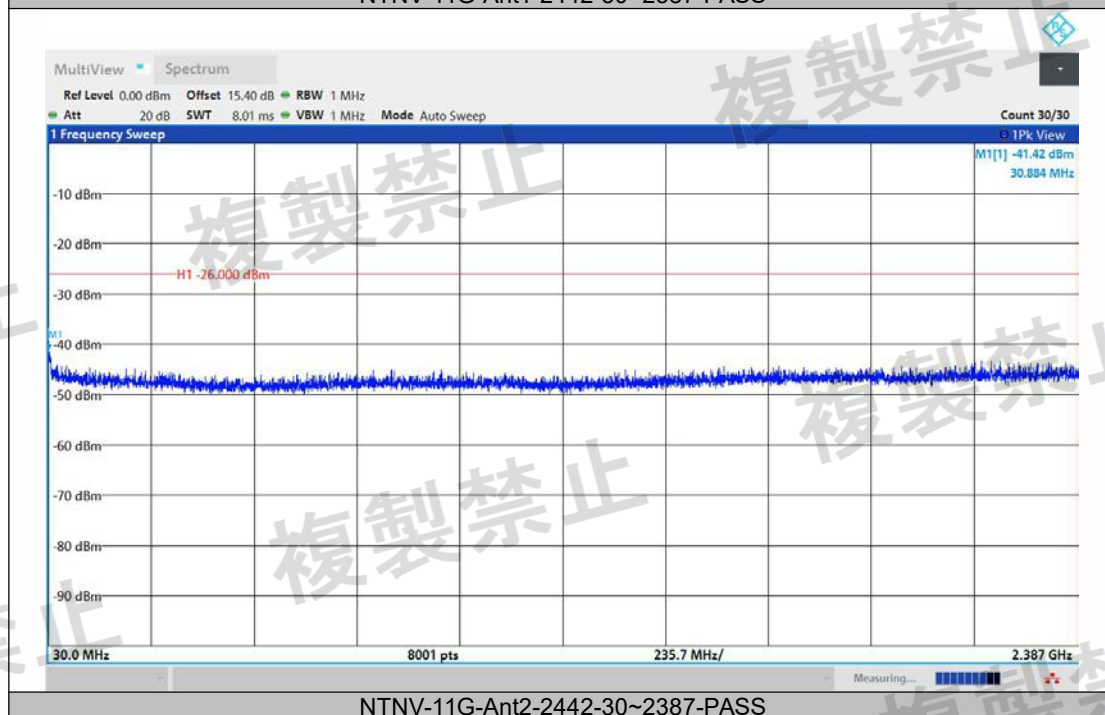
NTNV-11G-Ant2-2442-30~2387-PASS
