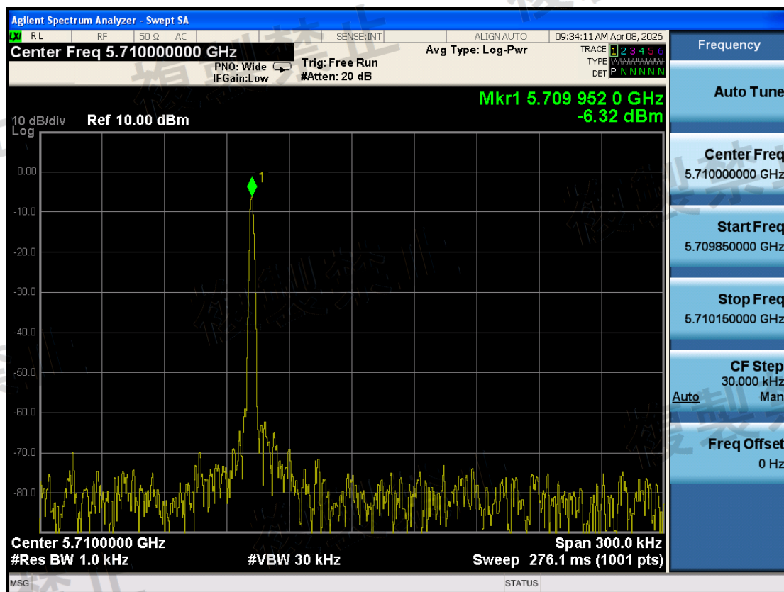
W56\Frequency Error Measurement\802.11ax HE40\5710-TX1-N
