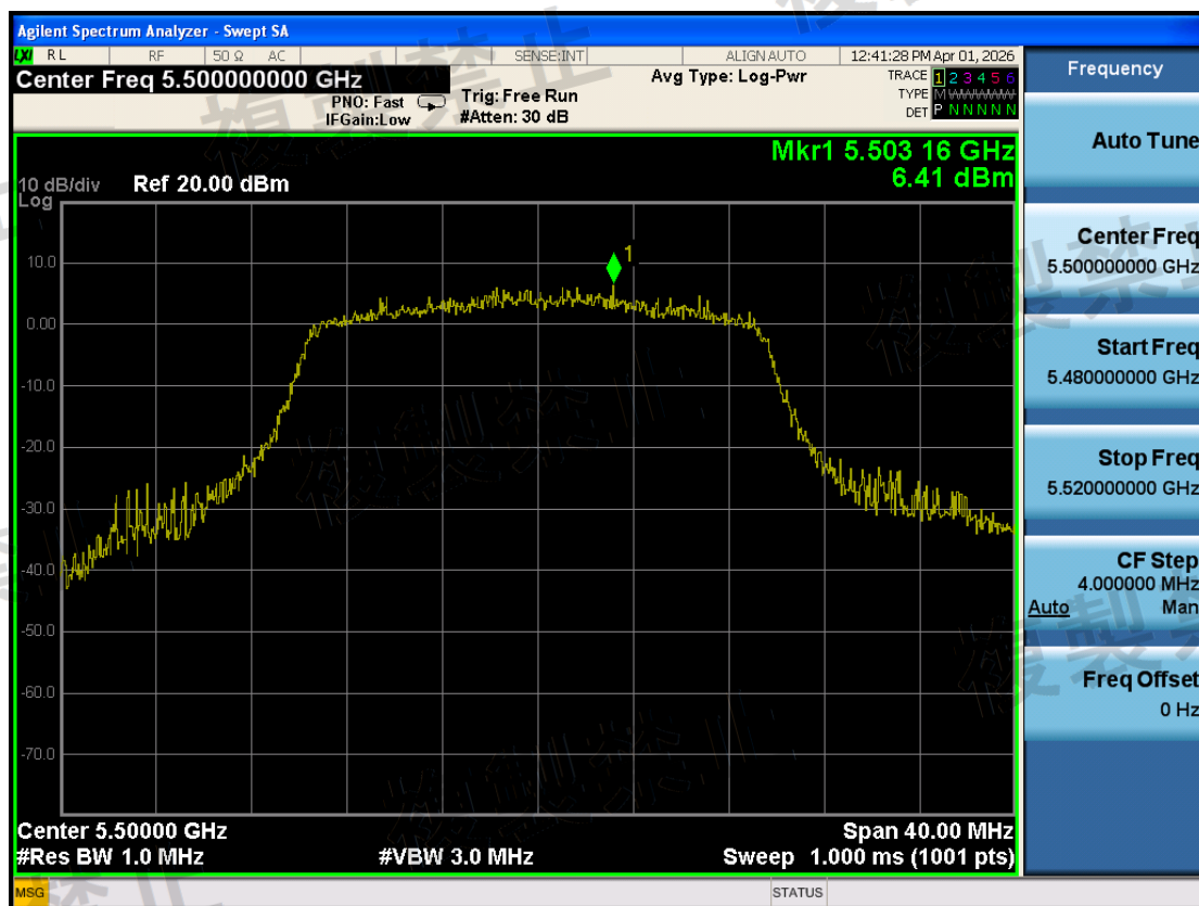
W56\Antenna Power Error\802.11ax HE20\1-5500-TX1-N
