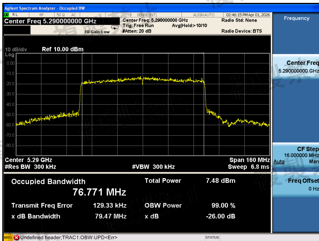
W53\Occupied Bandwidth\802.11ax HE80\5290-TX0-N
