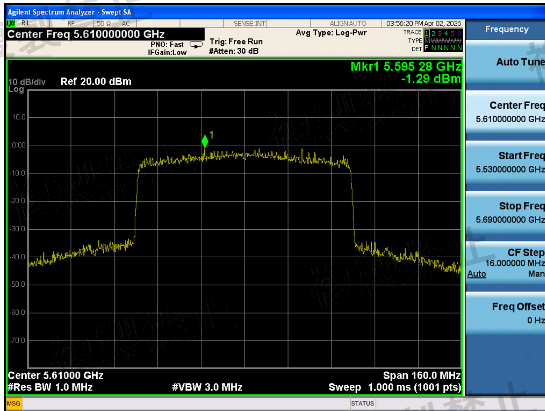
W56\Antenna Power Error\802.11ax HE80\1-5610-TX0-N
