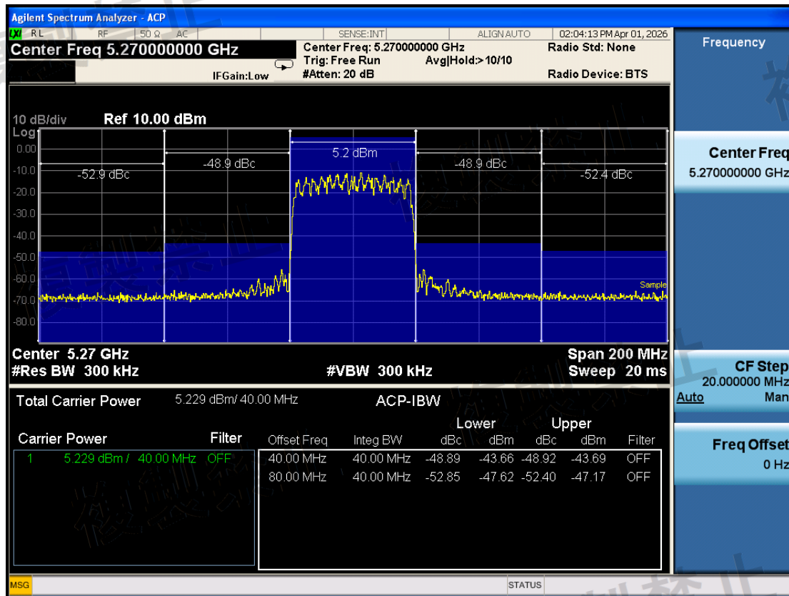
W53\Adjacent Channel Leakage Power\802.11ax HE40\5270-X-N
