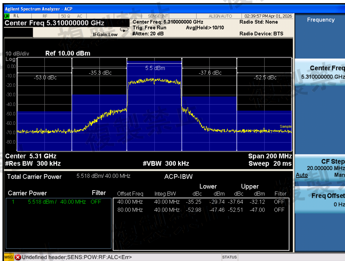
W53\Adjacent Channel Leakage Power\802.11ax HE40\5310-TX0-N
