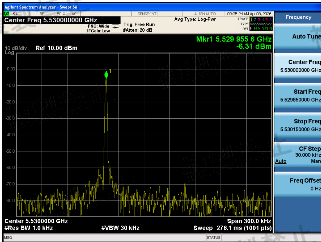
W56\Frequency Error Measurement\802.11ax HE80\5530-TX1-N
