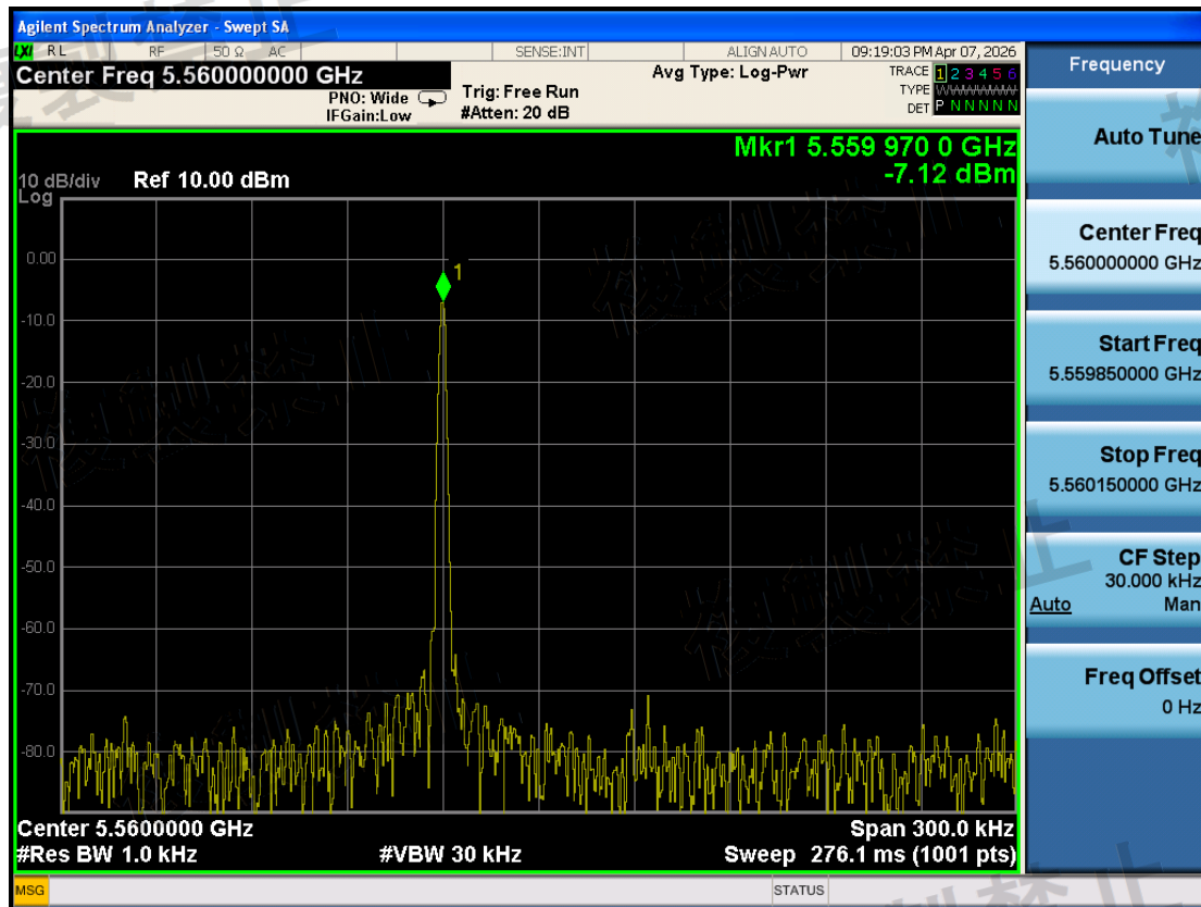
W56\Frequency Error Measurement\802.11a\5560-TX0-N
