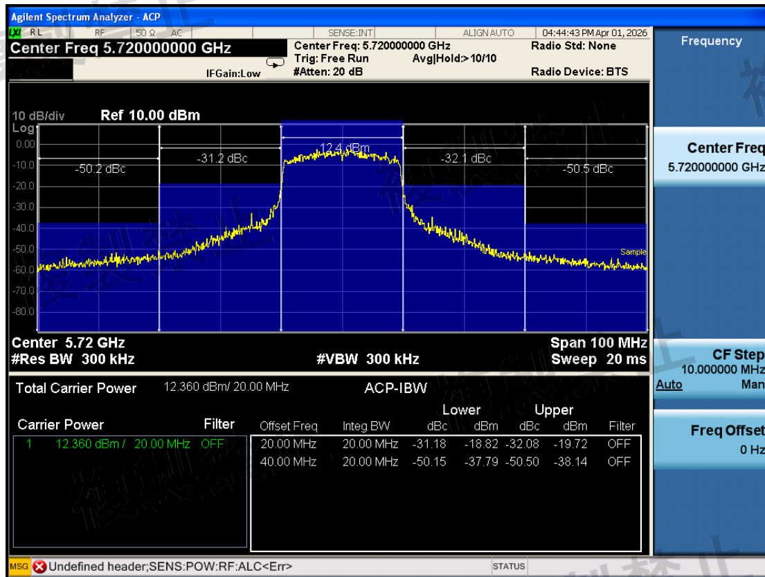
W56\Adjacent Channel Leakage Power\802.11ax HE20\5720-TX0-N
