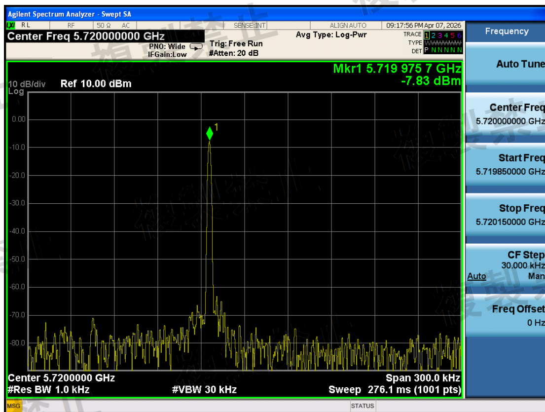
W56\Frequency Error Measurement\802.11ax HE20\5720-TX0-N
