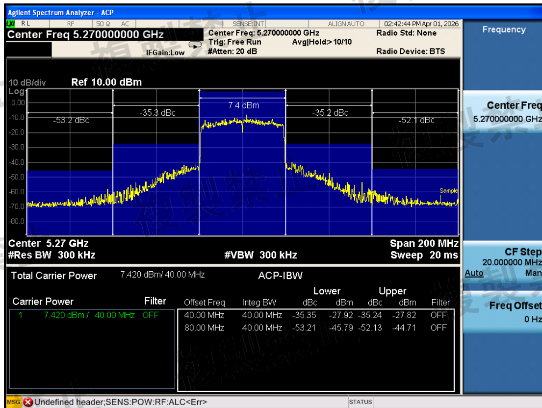
W53\Adjacent Channel Leakage Power\802.11ax HE40\5270-TX1-N
