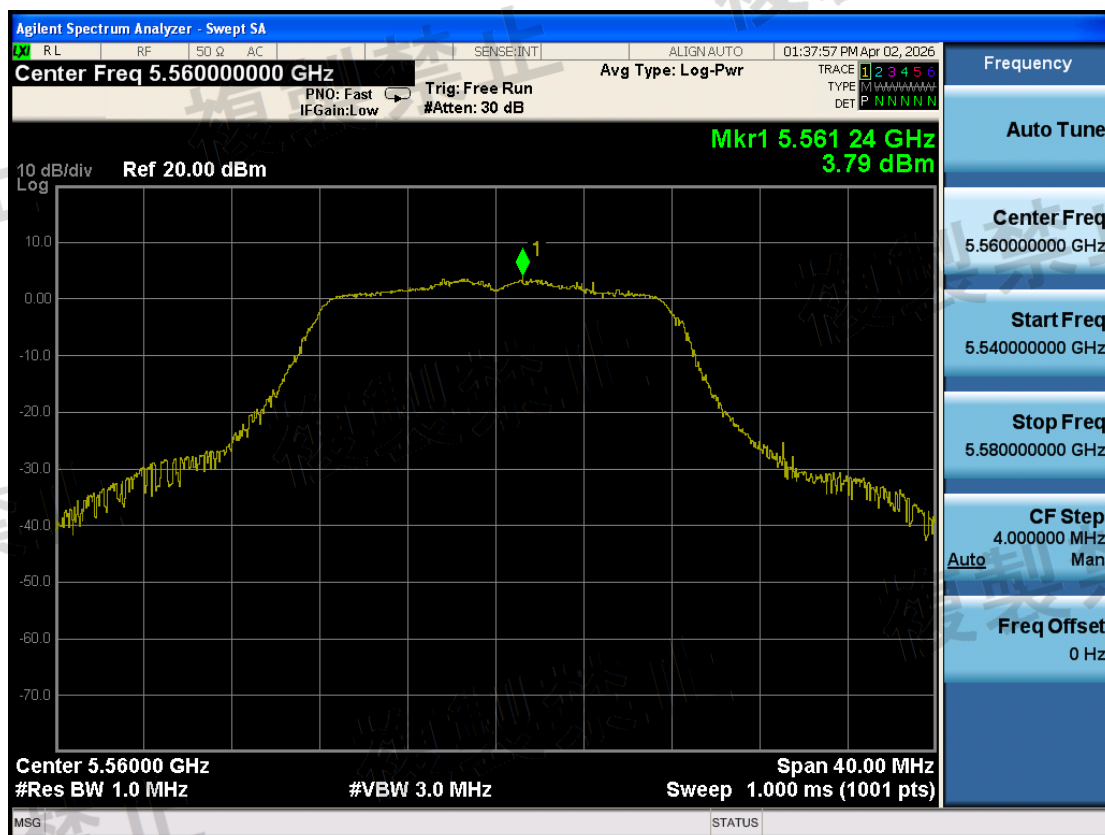
W56\Antenna Power Error\802.11a\1-5560-TX0-N
