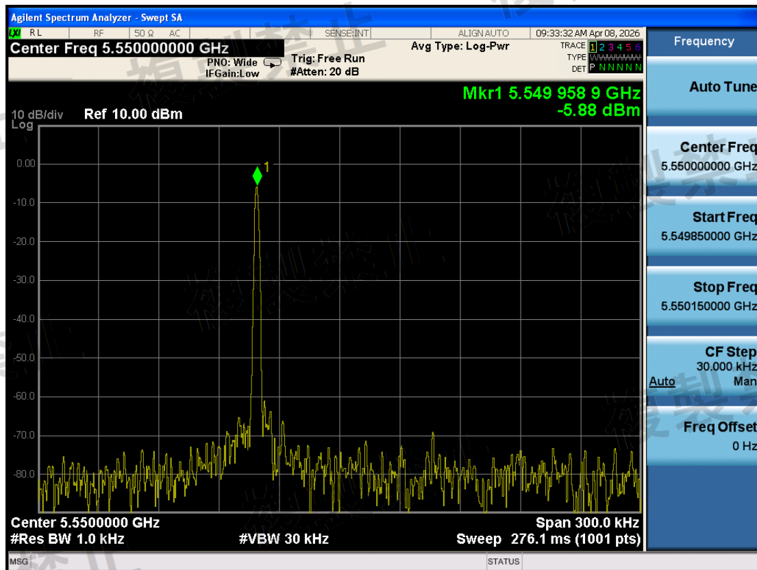
W56\Frequency Error Measurement\802.11ax HE40\5550-TX1-N
