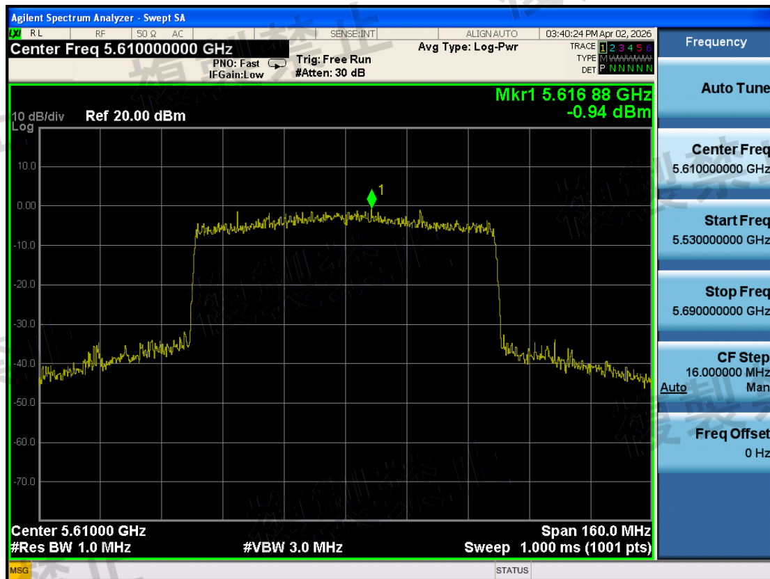
W56\Antenna Power Error\802.11ax HE80\1-5610-TX1-N
