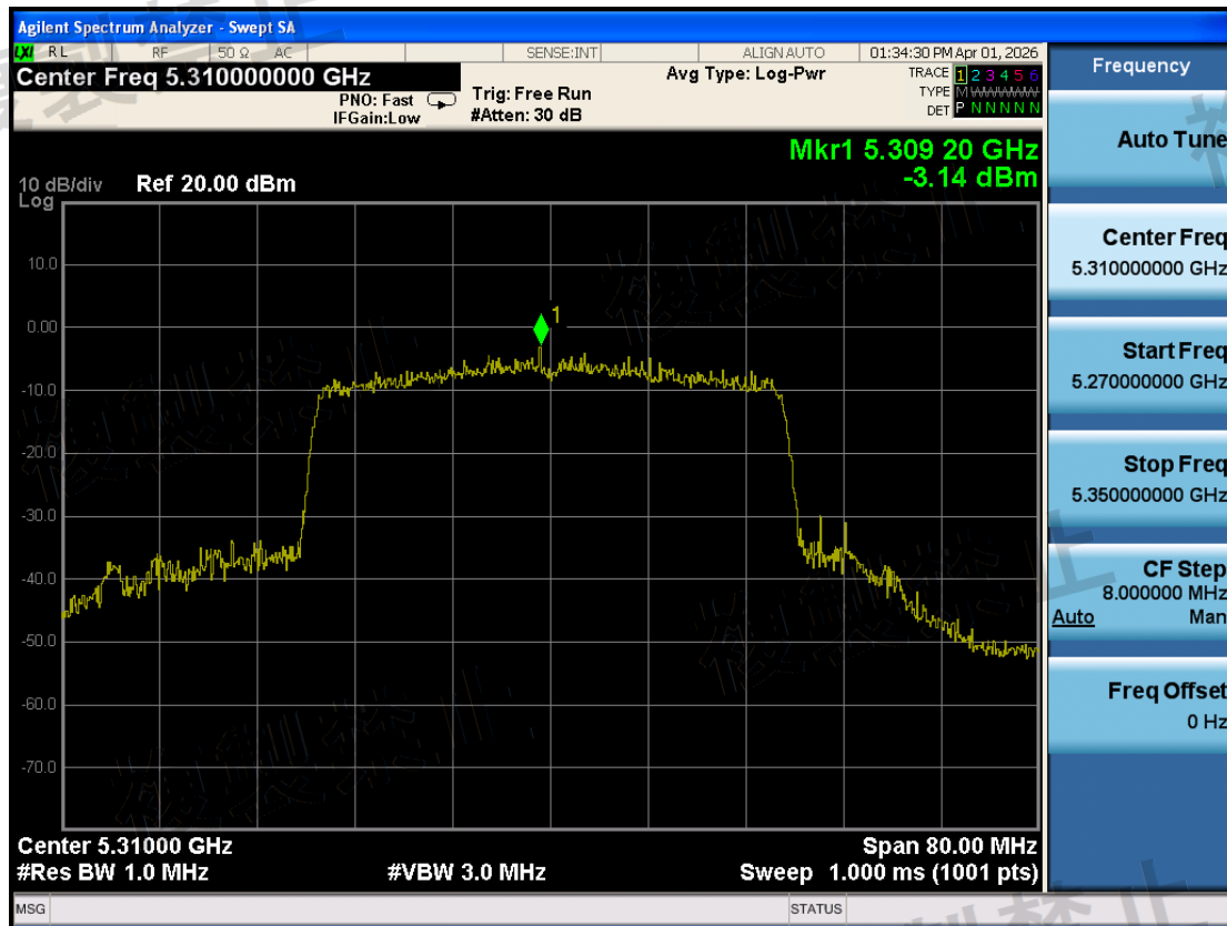
W53\Antenna Power Error\802.11ax HE40\1-5310-TX0-N
