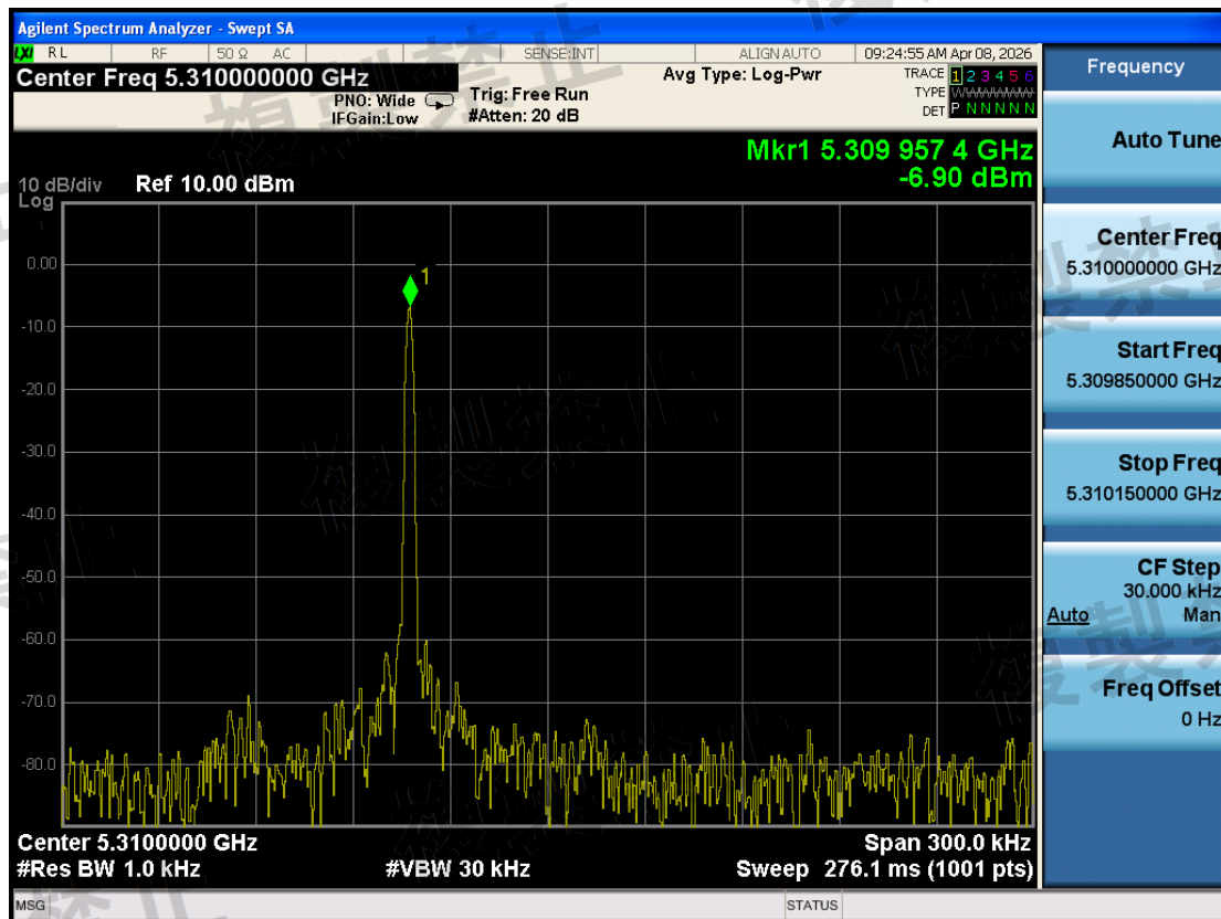
W53\Frequency Error Measurement\802.11ax HE40\5310-TX1-N
