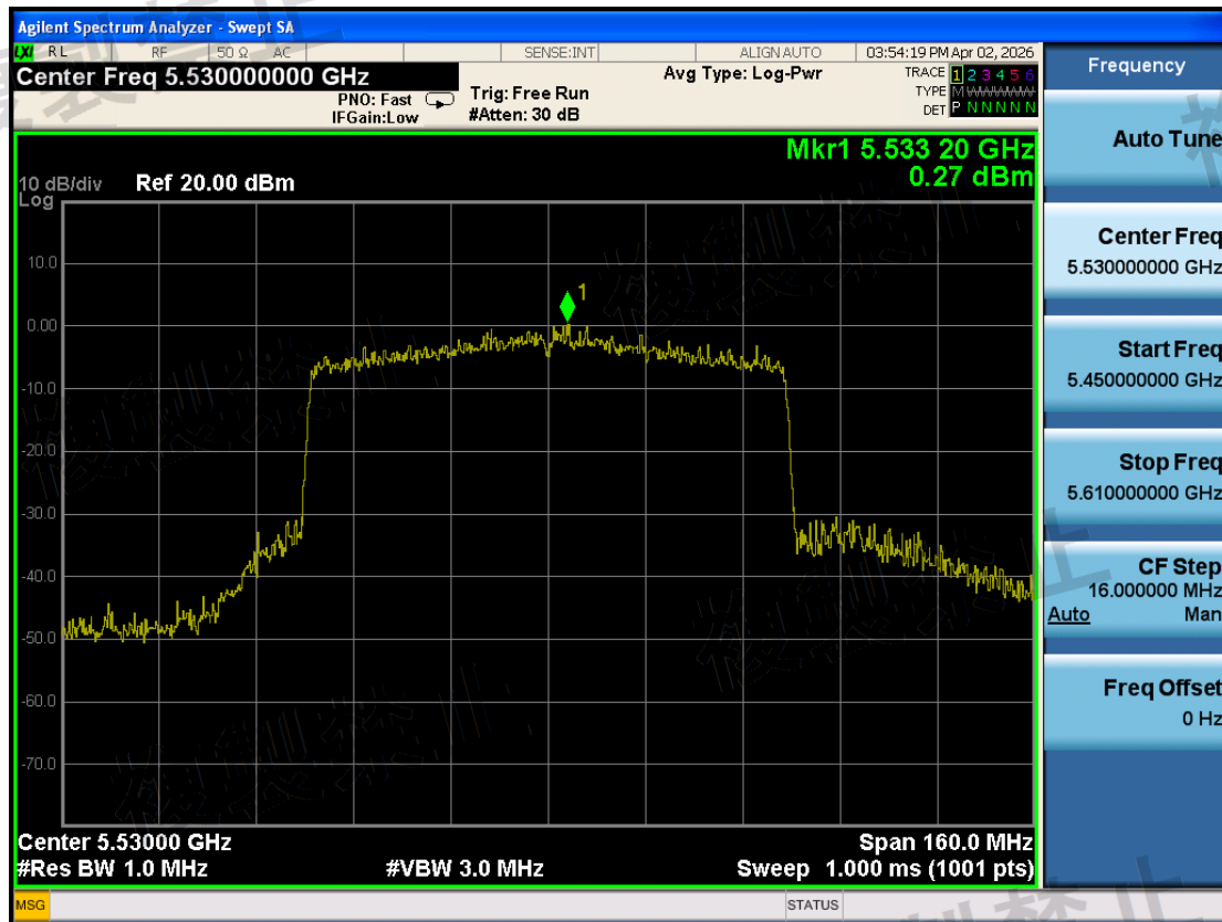
W56\Antenna Power Error\802.11ax HE80\1-5530-TX0-N
