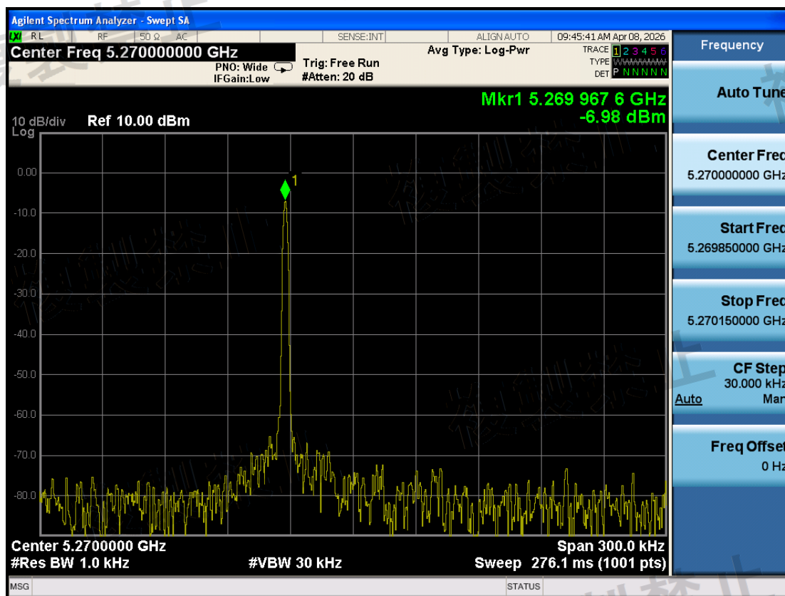
W53\Frequency Error Measurement\802.11ax HE40\5270-TX0-N
