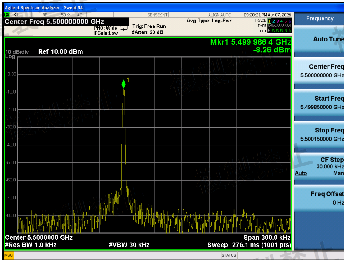
W56\Frequency Error Measurement\802.11a\5500-TX0-N
