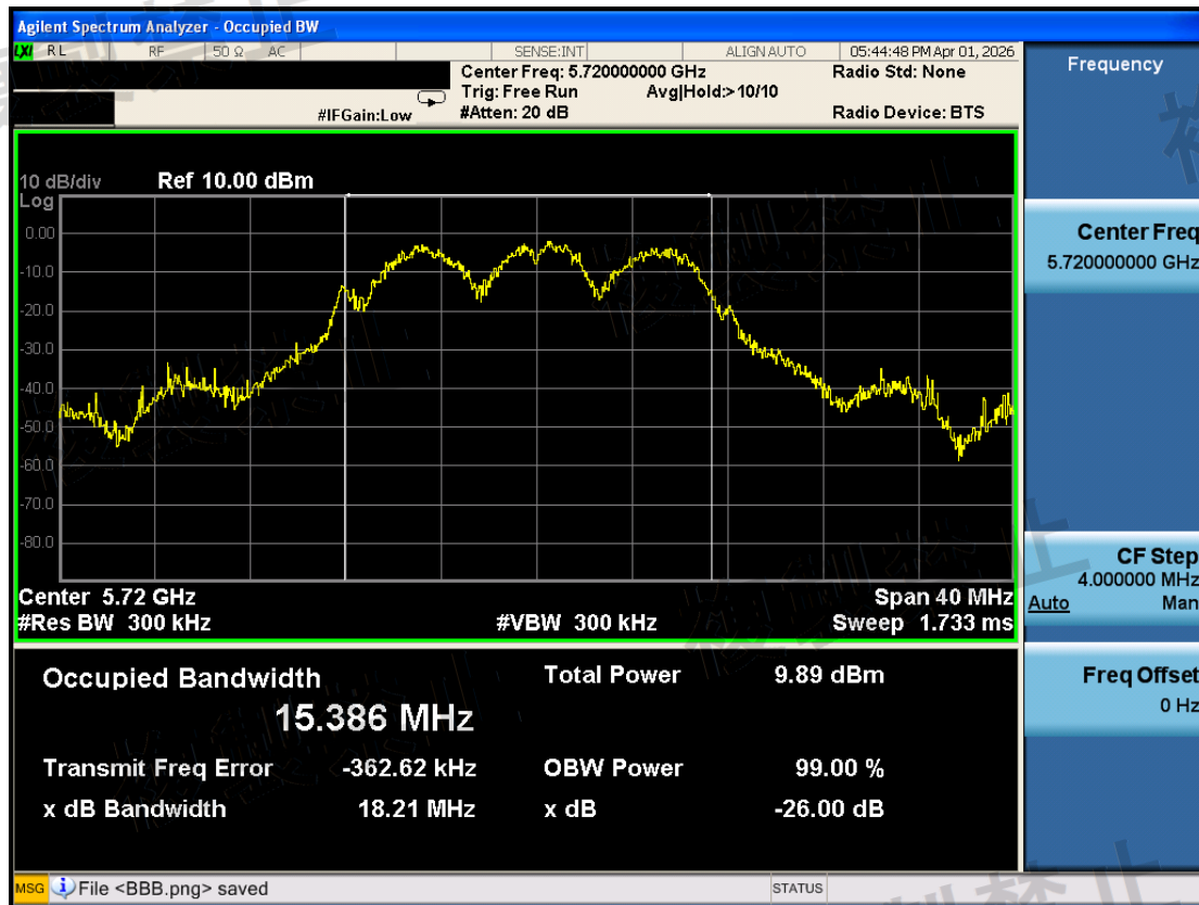
W56\Occupied Bandwidth\802.11a\5720-X-N
