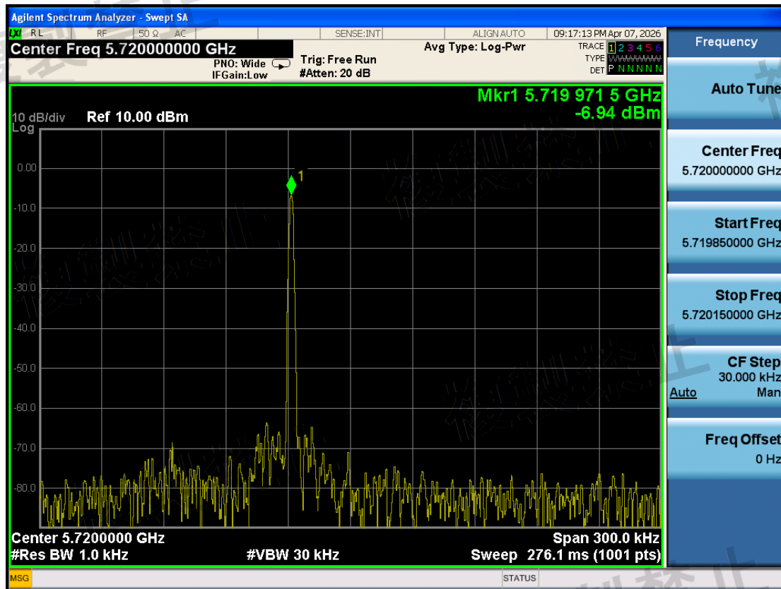
W56\Frequency Error Measurement\802.11ax HE20\5720-TX1-N
