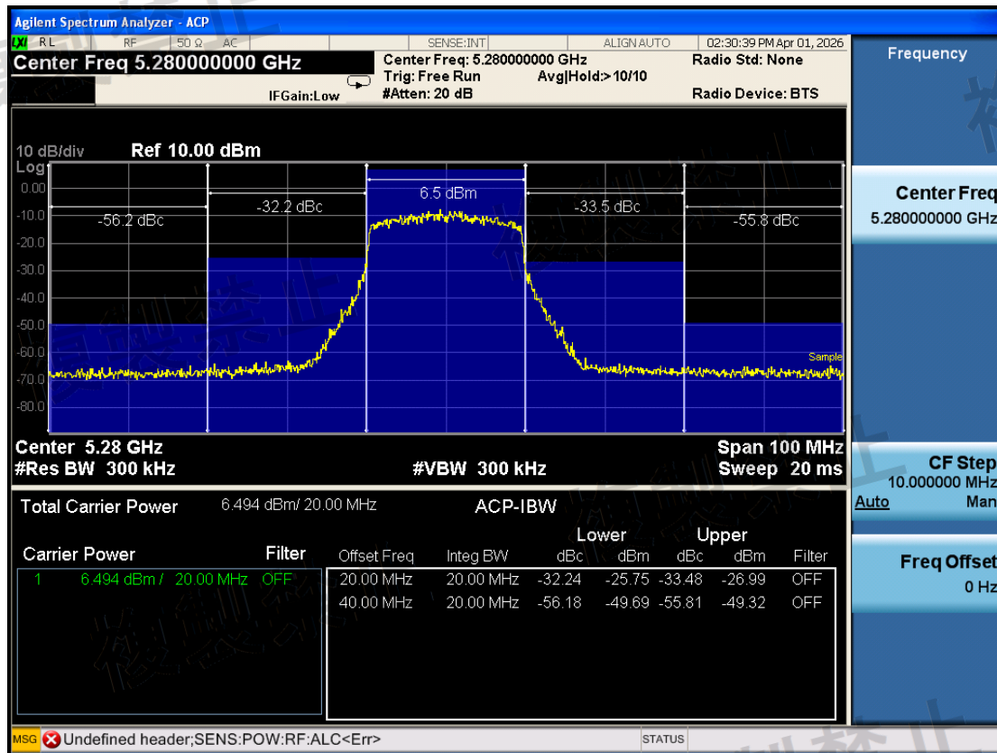
W53\Adjacent Channel Leakage Power\802.11ax HE20\5280-TX1-N
