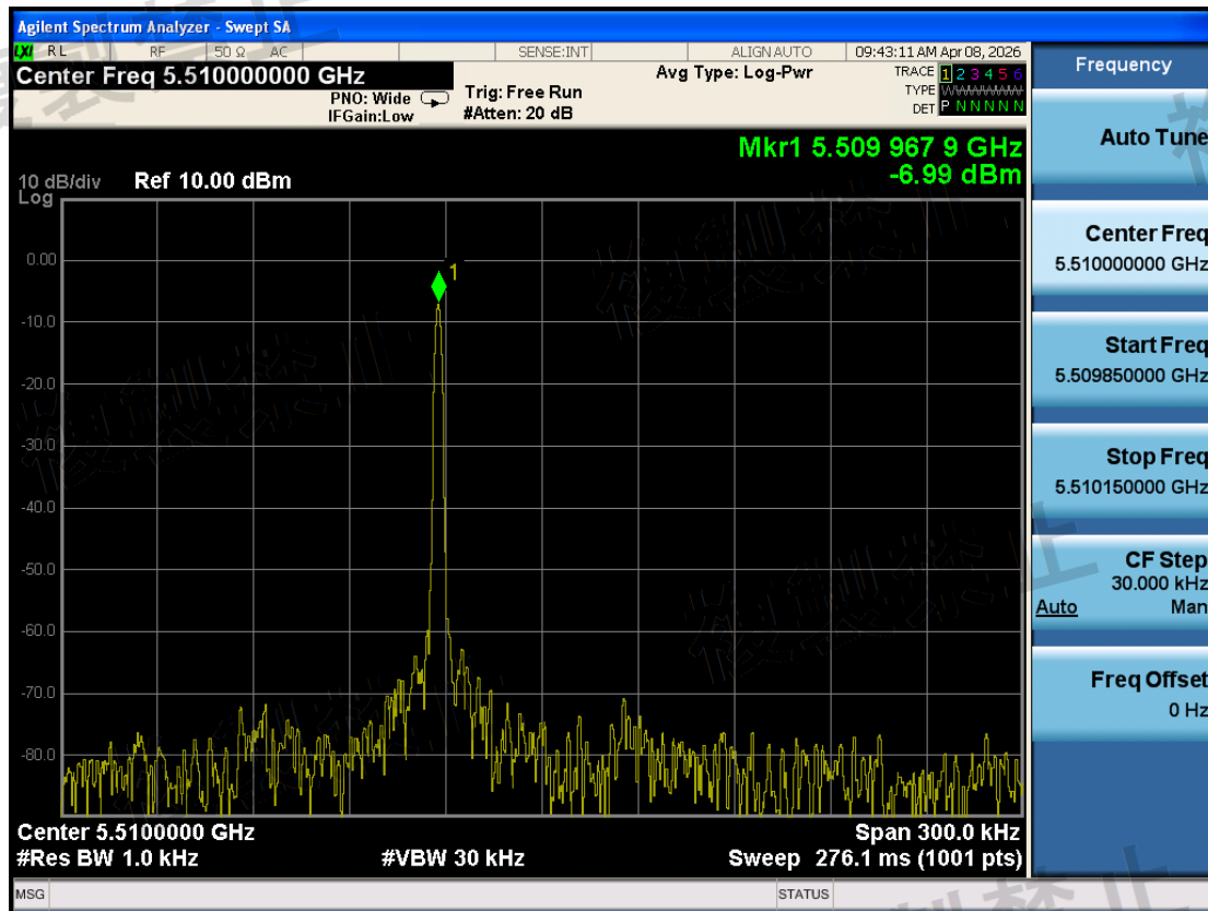
W56\Frequency Error Measurement\802.11ax HE40\5510-TX0-N
