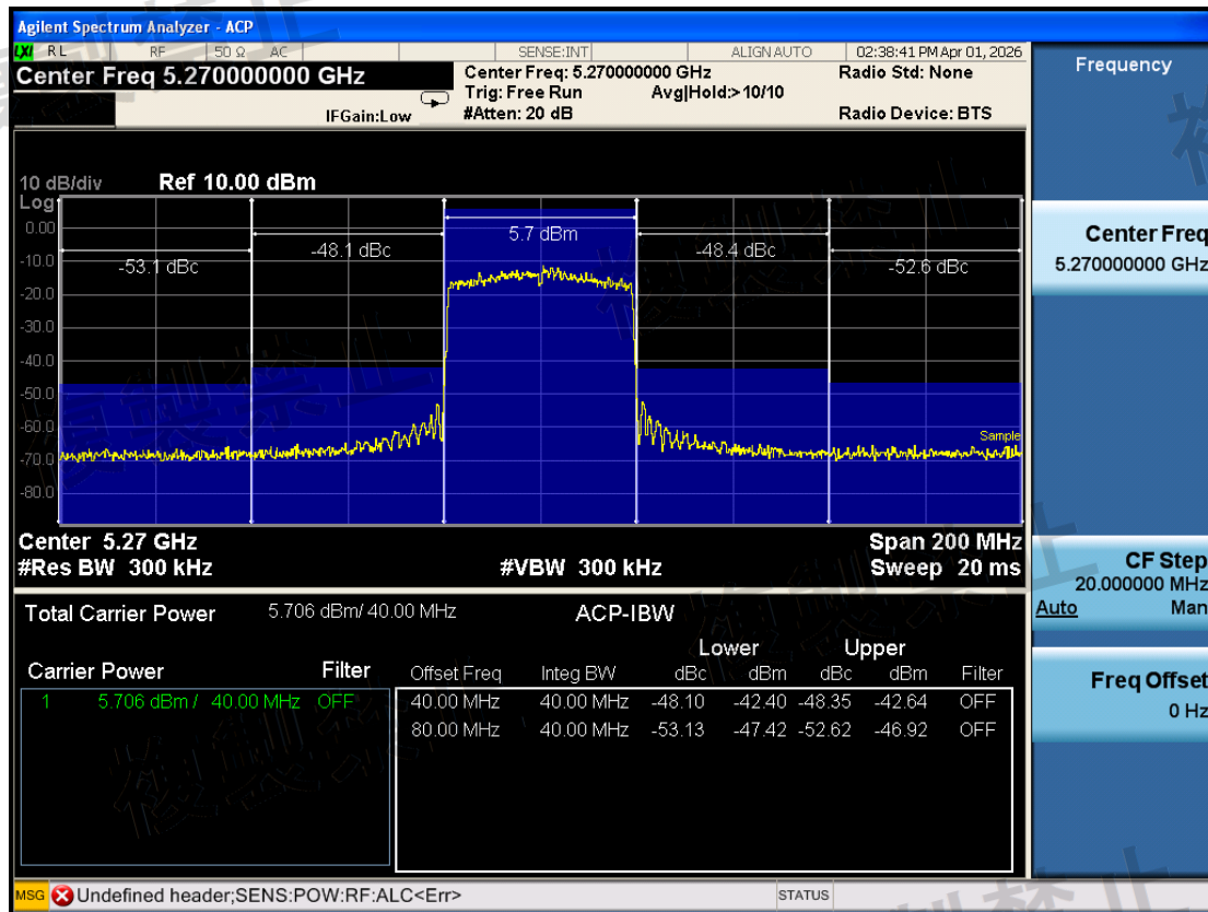
W53\Adjacent Channel Leakage Power\802.11ax HE40\5270-TX0-N
