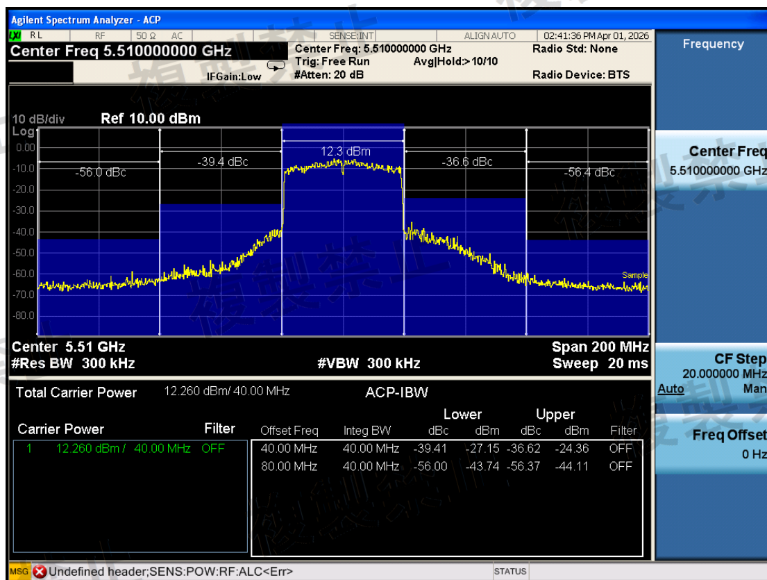
W56\Adjacent Channel Leakage Power\802.11ax HE40\5510-TX0-N
