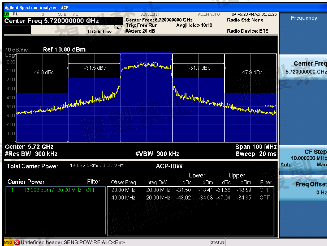
W56\Adjacent Channel Leakage Power\802.11ax HE20\5720-TX1-N
