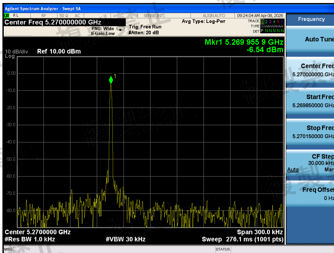
W53\Frequency Error Measurement\802.11ax HE40\5270-TX1-N
