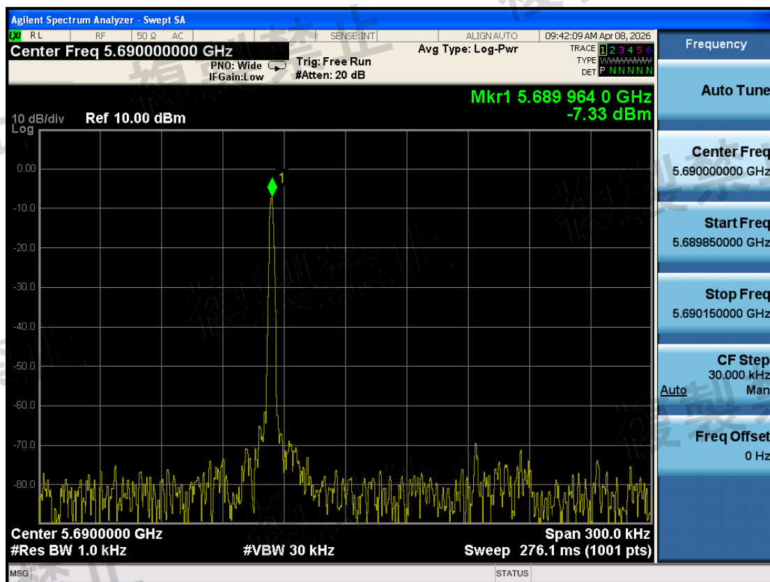
W56\Frequency Error Measurement\802.11ax HE80\5690-TX0-N
