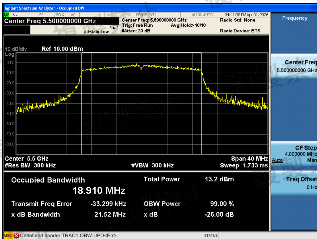
W56\Occupied Bandwidth\802.11ax HE20\5500-TX0-N
