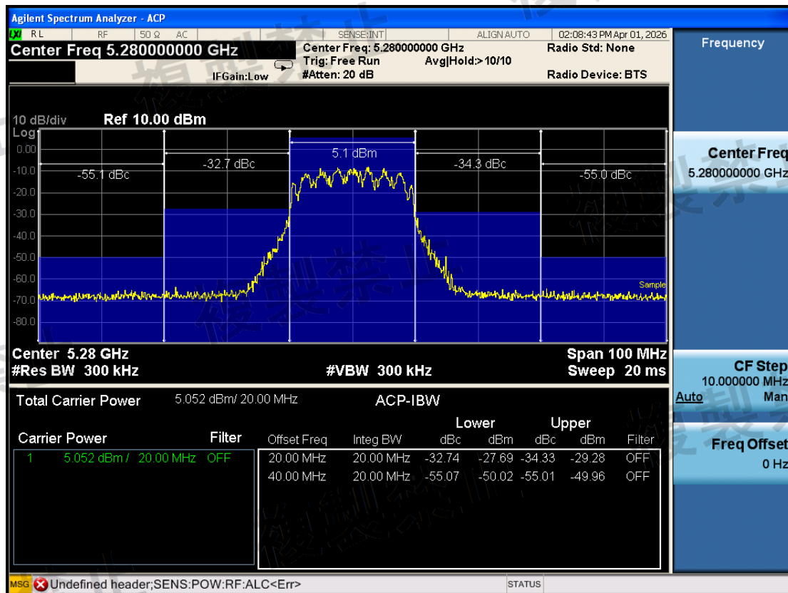
W53\Adjacent Channel Leakage Power\802.11ax HE20\5280-X-N
