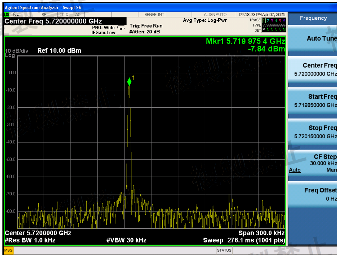
W56\Frequency Error Measurement\802.11a\5720-TX0-N
