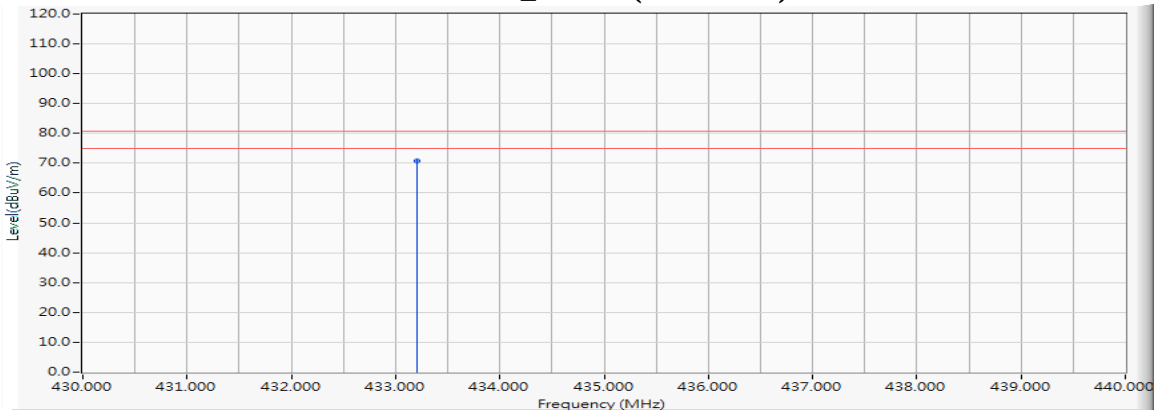
VERTICAL_Y- Axis (AVERAGE)
