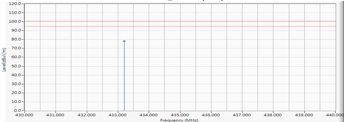
VERTICAL_Z- Axis (Peak)
