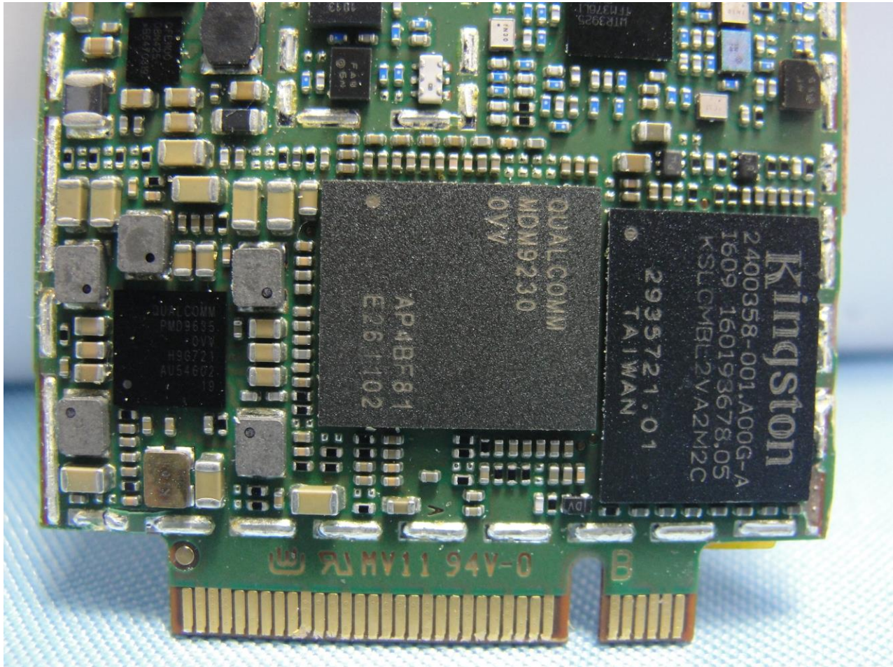
EUT: WWAN module (Brand Name: AirPrime / Model Name: EM7455)
