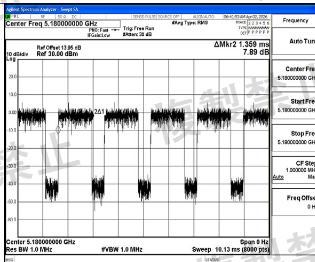
NTNV-11N20MIMO-Ant2-5180-PASS
