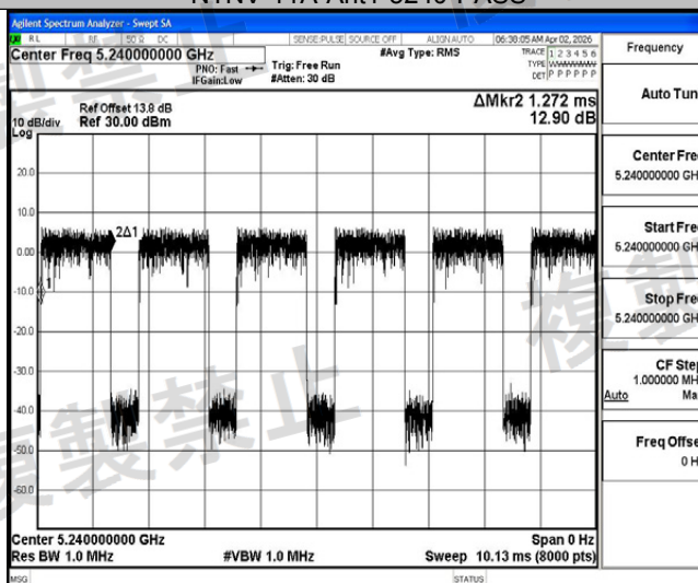
NTHV-11A-Ant1-5240-PASS
