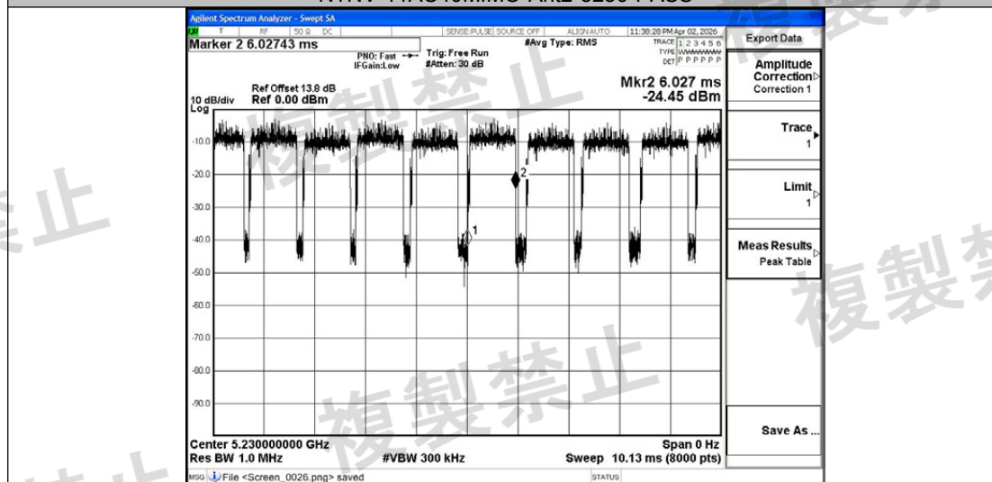
NTHV-11AC40MIMO-Ant2-5230-PASS
