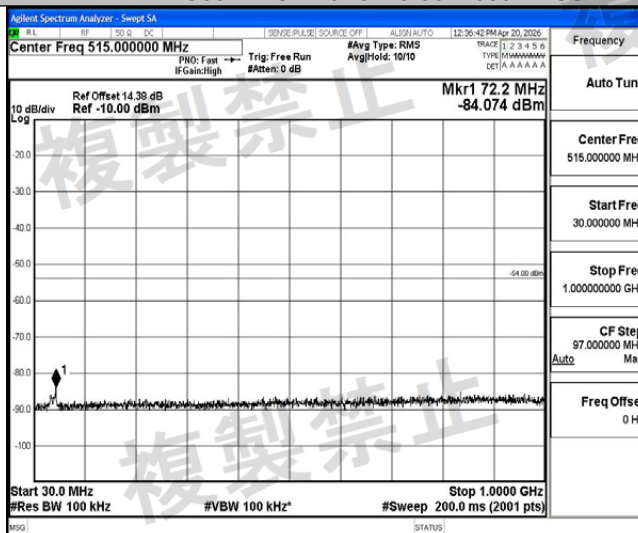
NTNV-11AC80MIMO-Ant2-5210-30~1000-PASS
