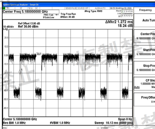
NTNV-11AC20MIMO-Ant2-5180-PASS
