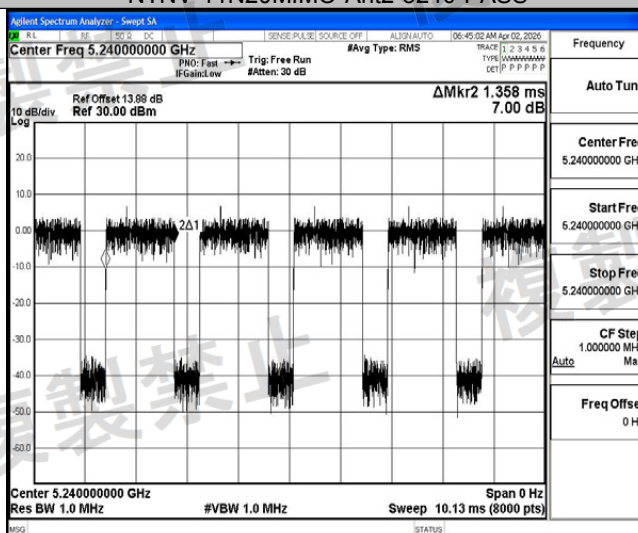
NTHV-11N20MIMO-Ant2-5240-PASS
