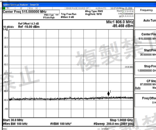
NTHV-11AC20MIMO-Ant1-5220-30~1000-PASS
