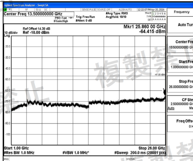
NTHV-11N40MIMO-Ant2-5230-1000~26000-PASS
