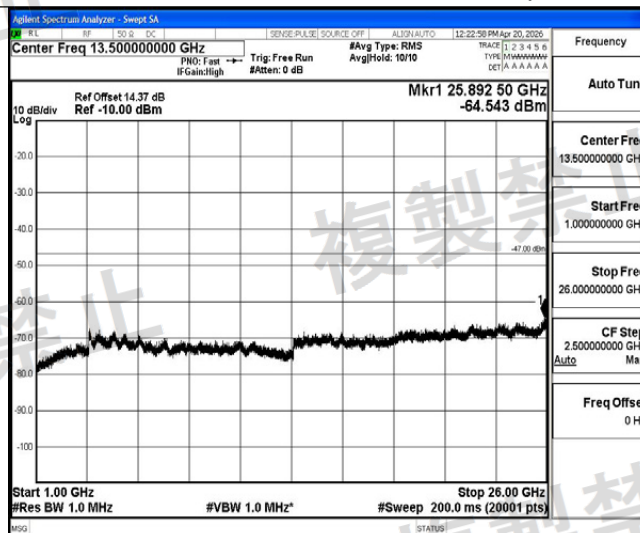
NTNV-11AC20MIMO-Ant1-5180-1000~26000-PASS
