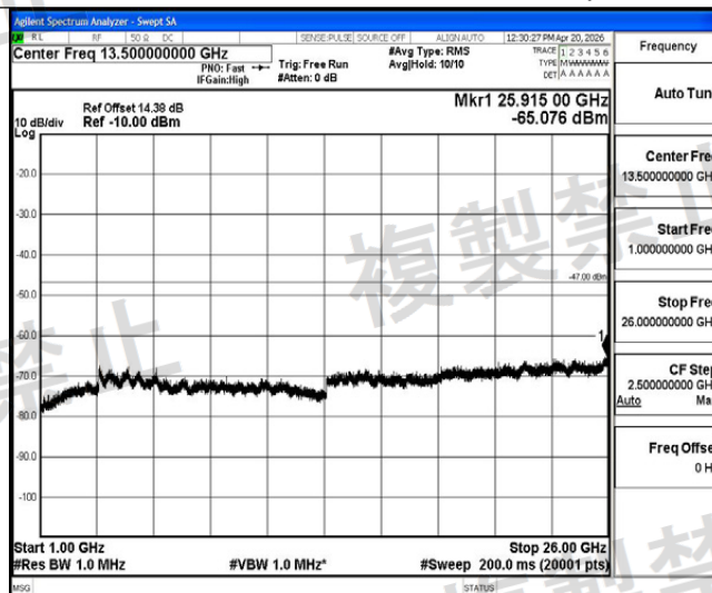
NTNV-11AC20MIMO-Ant2-5240-1000~26000-PASS
