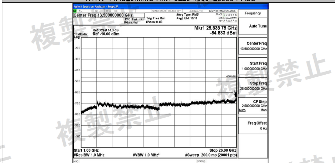
NTHV-11AC20MIMO-Ant1-5220-1000~26000-PASS
