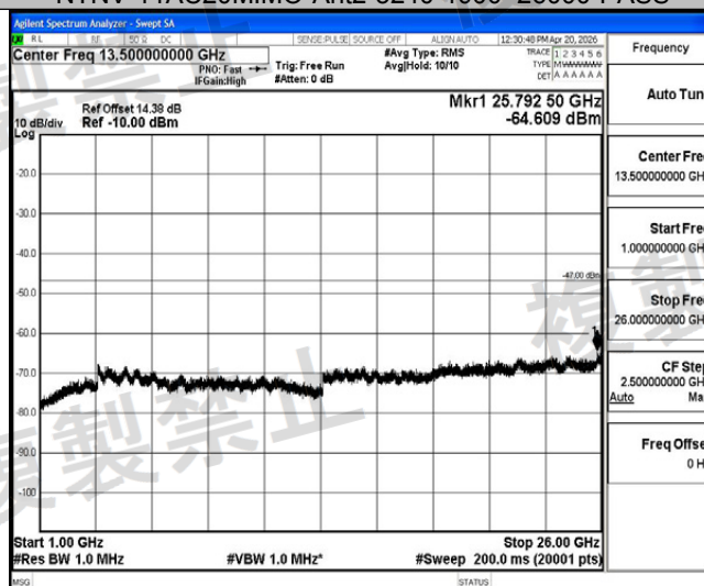
NTHV-11AC20MIMO-Ant2-5240-1000~26000-PASS
