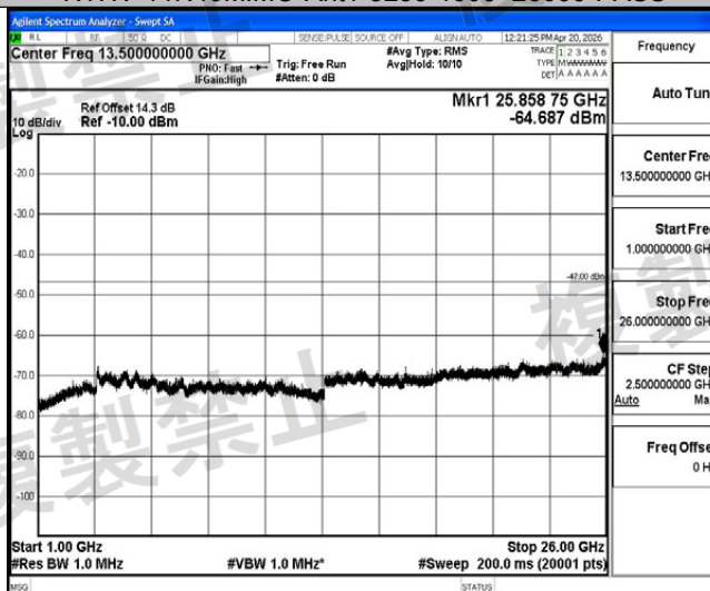
NTLV-11N40MIMO-Ant2-5230-1000~26000-PASS
