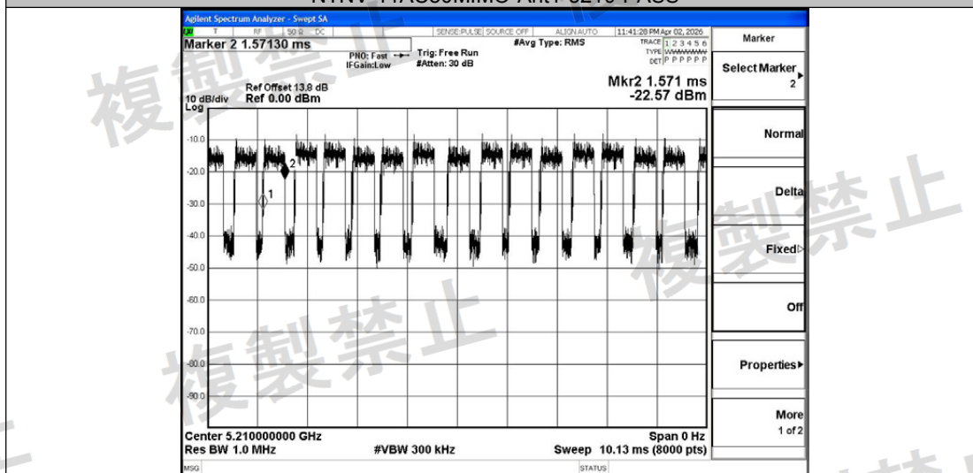
NTHV-11AC80MIMO-Ant1-5210-PASS
