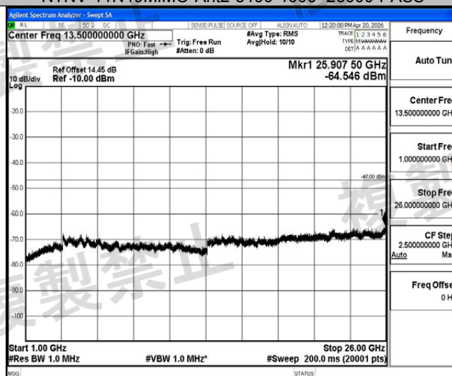
NTHV-11N40MIMO-Ant2-5190-1000~26000-PASS
