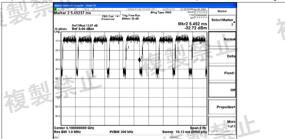
NTHV-11N40MIMO-Ant1-5190-PASS
