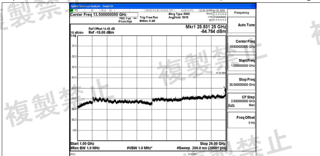
NTNV-11AC20MIMO-Ant2-5200-1000~26000-PASS
