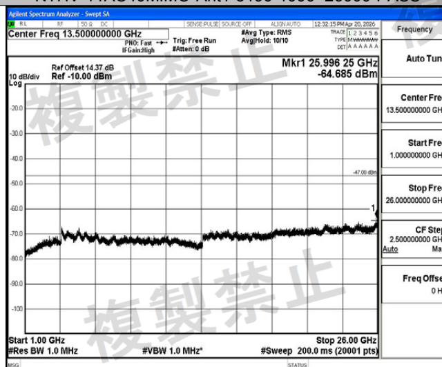
NTLV-11AC40MIMO-Ant2-5190-1000~26000-PASS
