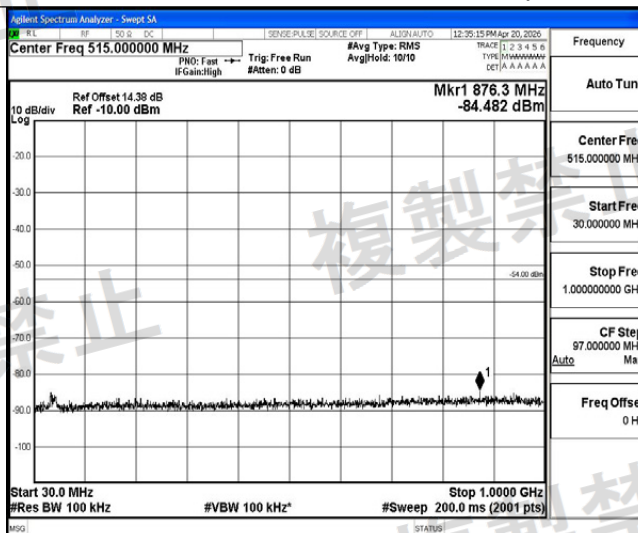
NTLV-11AC40MIMO-Ant1-5230-30~1000-PASS
