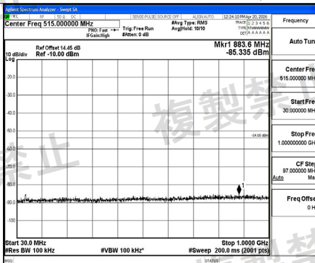
NTHV-11AC20MIMO-Ant2-5180-30~1000-PASS
