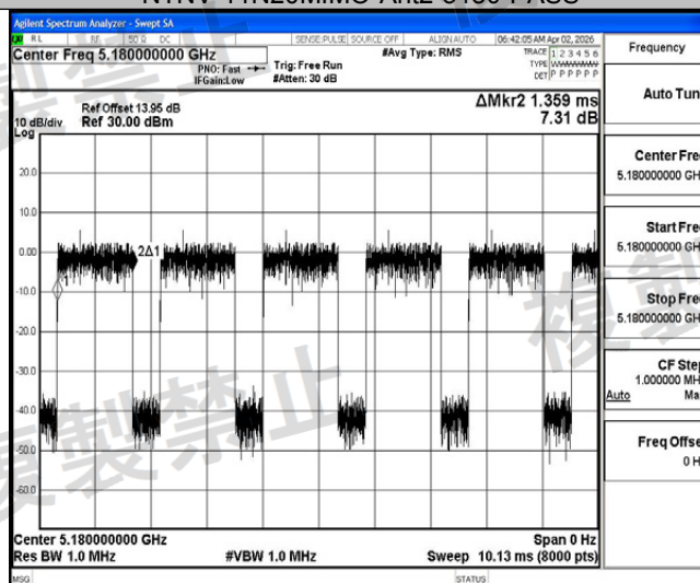
NTHV-11N20MIMO-Ant2-5180-PASS
