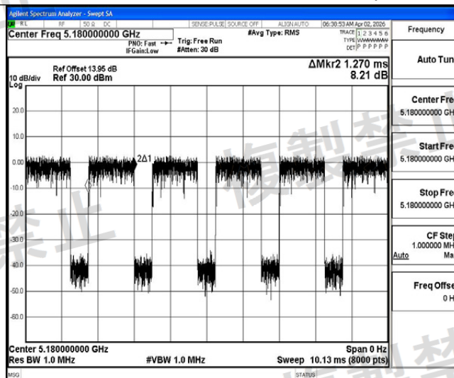
NTVN-11A-Ant2-5180-PASS
