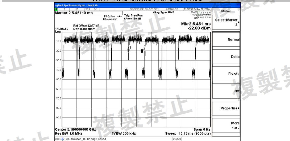
NTLV-11AC40MIMO-Ant2-5190-PASS
