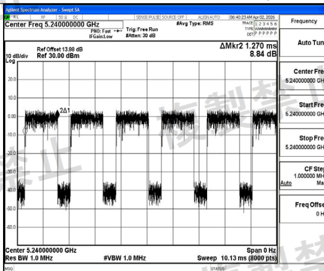
NTVN-11A-Ant2-5240-PASS
