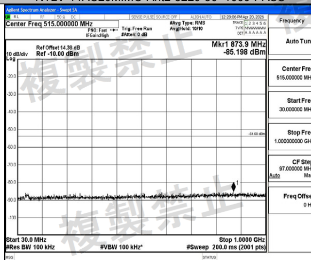
NTHV-11AC20MIMO-Ant2-5220-30~1000-PASS
