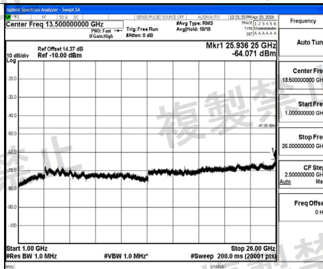
NTNV-11AC40MIMO-Ant1-5190-1000~26000-PASS
