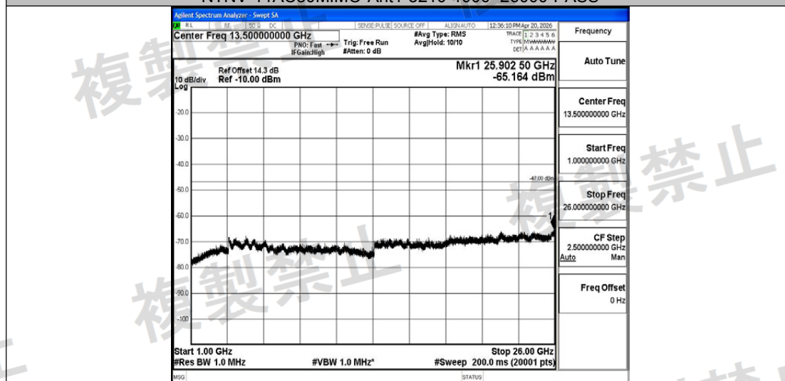
NTHV-11AC80MIMO-Ant1-5210-1000~26000-PASS
