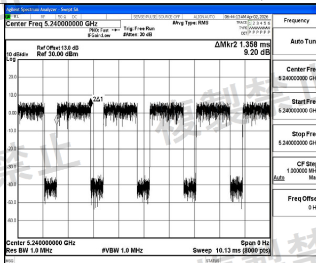
NTNV-11N20MIMO-Ant1-5240-PASS
