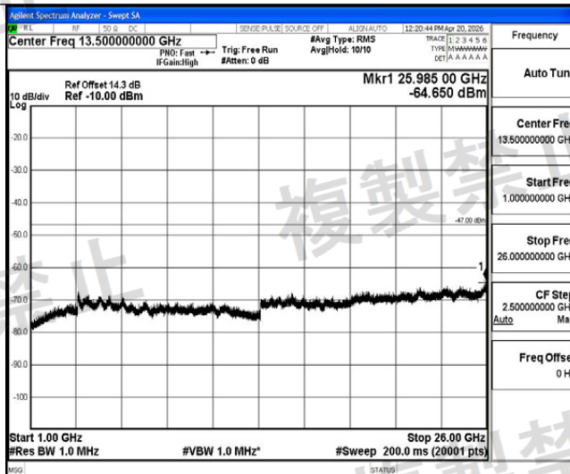
NTHV-11N40MIMO-Ant1-5230-1000~26000-PASS
