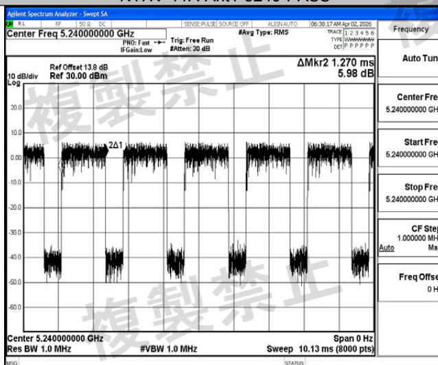
NTLV-11A-Ant2-5240-PASS
