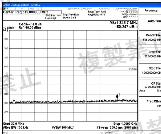
NTNV-11AC20MIMO-Ant1-5220-30~1000-PASS
