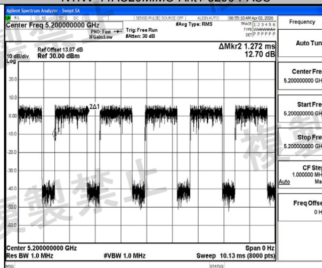
NTHV-11AC20MIMO-Ant1-5200-PASS
