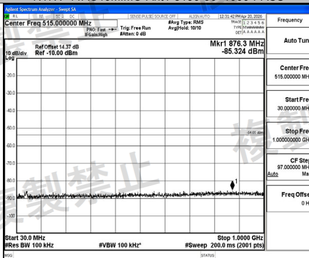
NTHV-11AC40MIMO-Ant1-5190-30~1000-PASS
