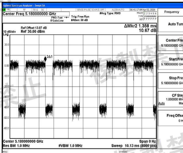
NTVN-11N20MIMO-Ant1-5180-PASS
