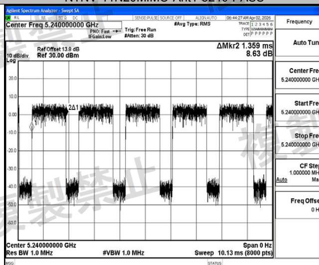
NTHV-11N20MIMO-Ant1-5240-PASS
