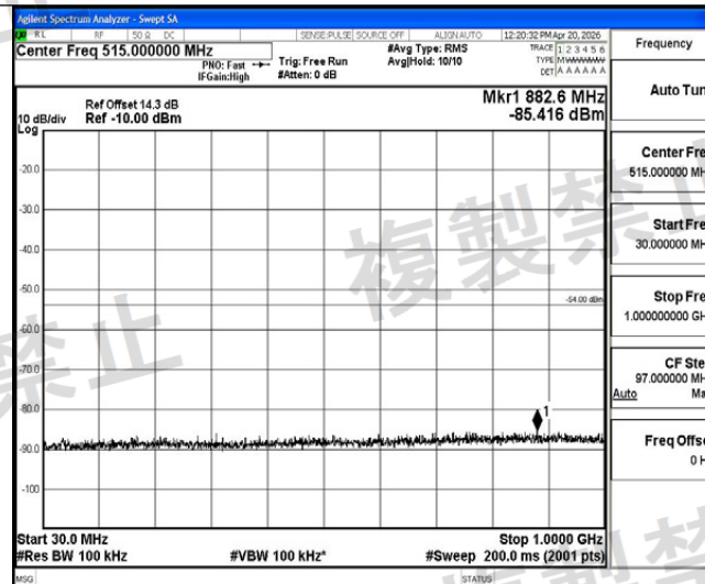
NTNV-11N40MIMO-Ant1-5230-30~1000-PASS
