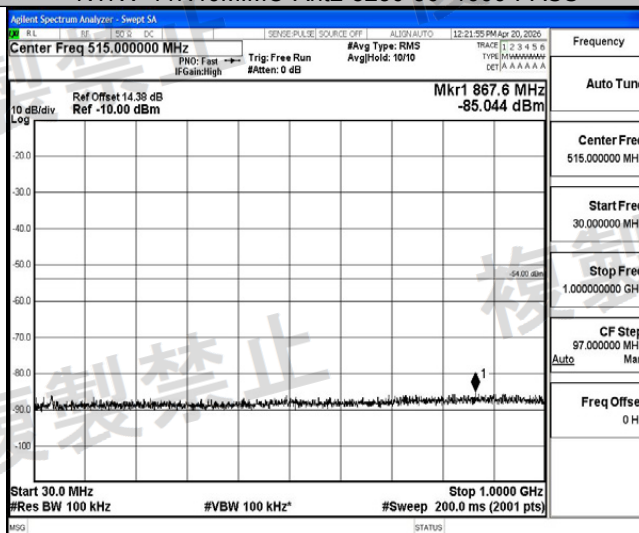
NTHV-11N40MIMO-Ant2-5230-30~1000-PASS
