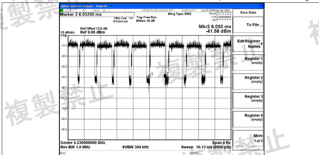
NTHV-11N40MIMO-Ant1-5230-PASS
