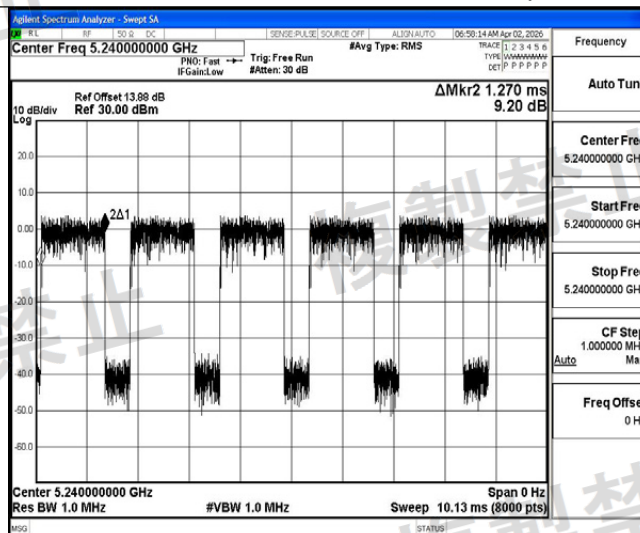
NTLV-11AC20MIMO-Ant1-5240-PASS
