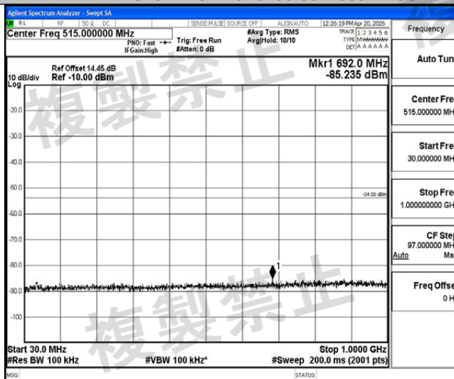
NTHV-11AC20MIMO-Ant2-5200-30~1000-PASS
