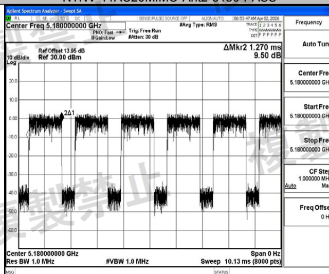
NTHV-11AC20MIMO-Ant2-5180-PASS
