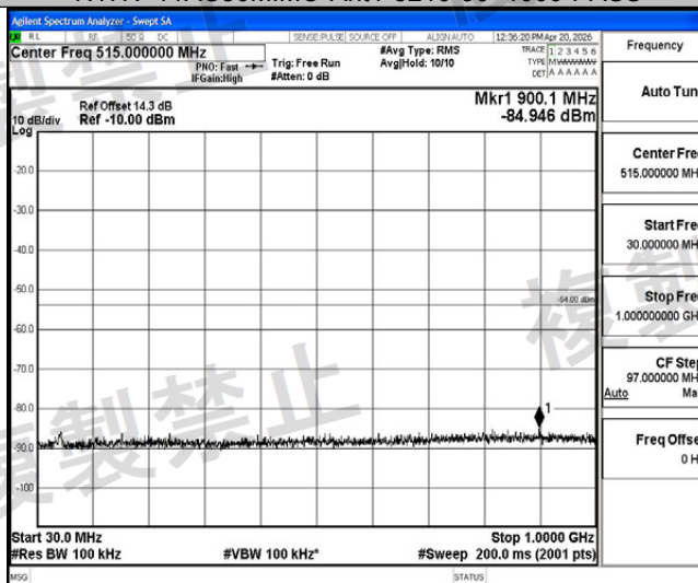
NTLV-11AC80MIMO-Ant2-5210-30~1000-PASS
