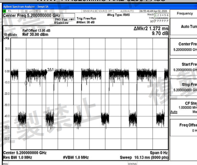
NTHV-11AC20MIMO-Ant2-5200-PASS
