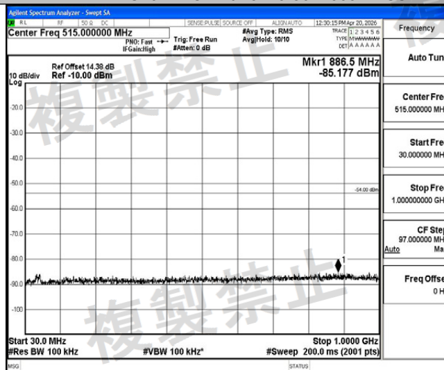
NTNV-11AC20MIMO-Ant2-5240-30~1000-PASS
