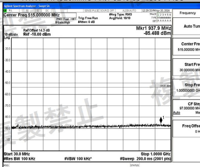
NTLV-11AC20MIMO-Ant2-5240-30~1000-PASS
