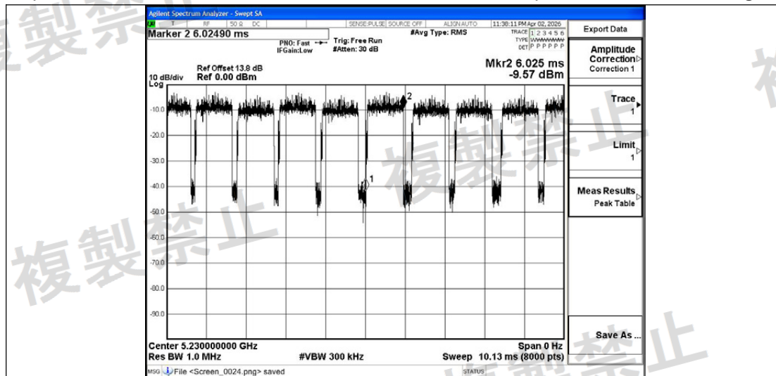
NTLV-11AC40MIMO-Ant2-5230-PASS
