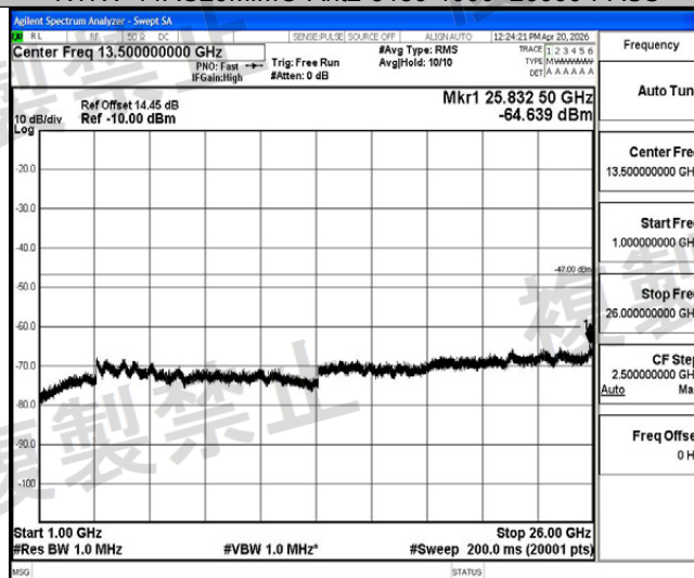
NTHV-11AC20MIMO-Ant2-5180-1000~26000-PASS
