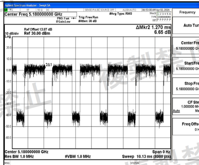
NTNV-11AC20MIMO-Ant1-5180-PASS
