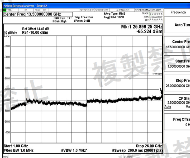
NTNV-11AC20MIMO-Ant2-5180-1000~26000-PASS
