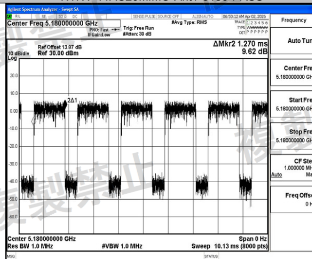
NTHV-11AC20MIMO-Ant1-5180-PASS
