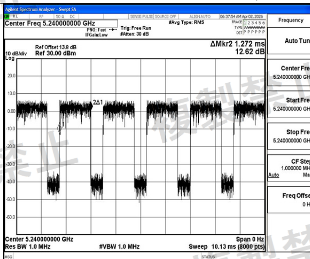
NTVN-11A-Ant1-5240-PASS
