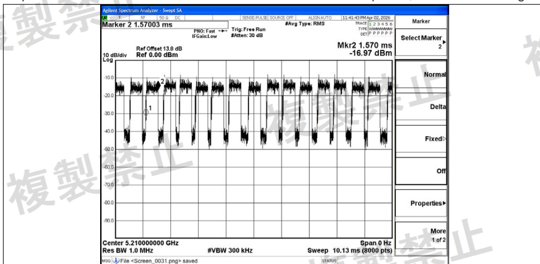
NTNV-11AC80MIMO-Ant2-5210-PASS
