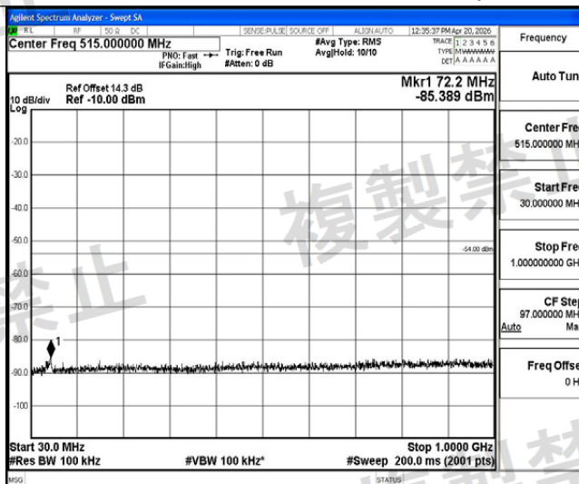
NTHV-11AC80MIMO-Ant1-5210-30~1000-PASS
