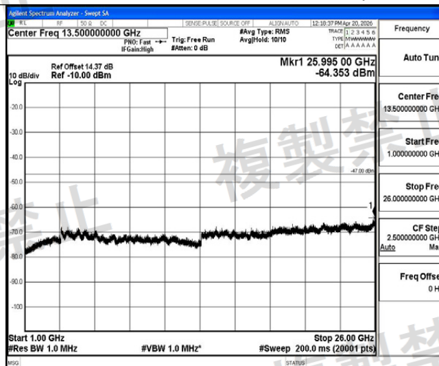
NTNV-11N40MIMO-Ant1-5190-1000~26000-PASS
