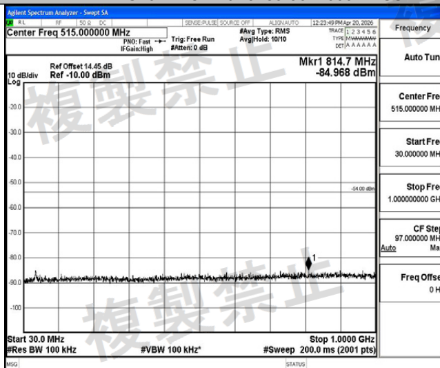
NTNV-11AC20MIMO-Ant2-5180-30~1000-PASS
