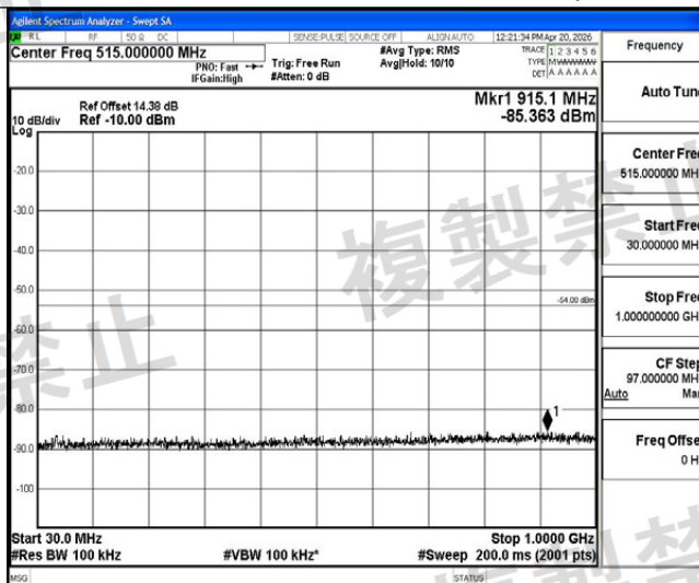
NTNV-11N40MIMO-Ant2-5230-30~1000-PASS
