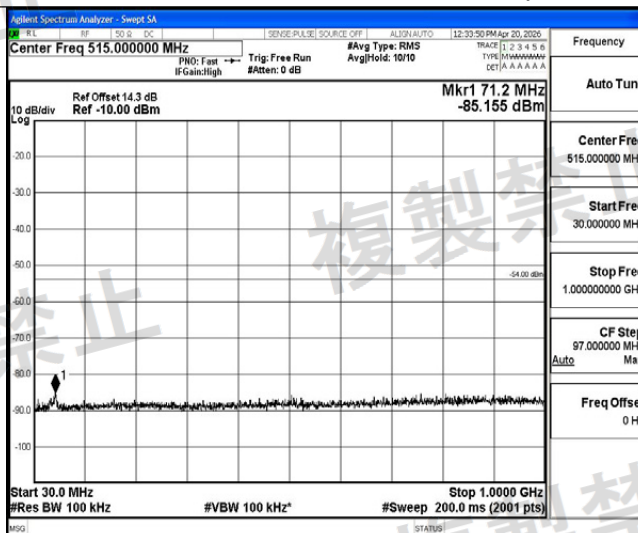
NTHV-11AC40MIMO-Ant1-5230-30~1000-PASS
