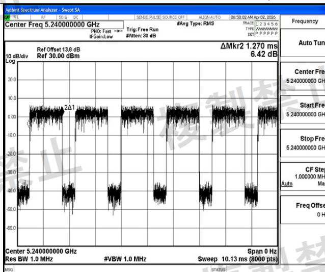
NTNV-11AC20MIMO-Ant2-5240-PASS
