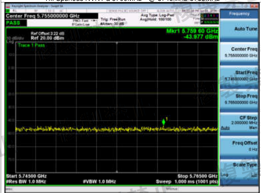
Tx. Spurious NVNT a 5700MHz @ 5745MHz-5765MHz
