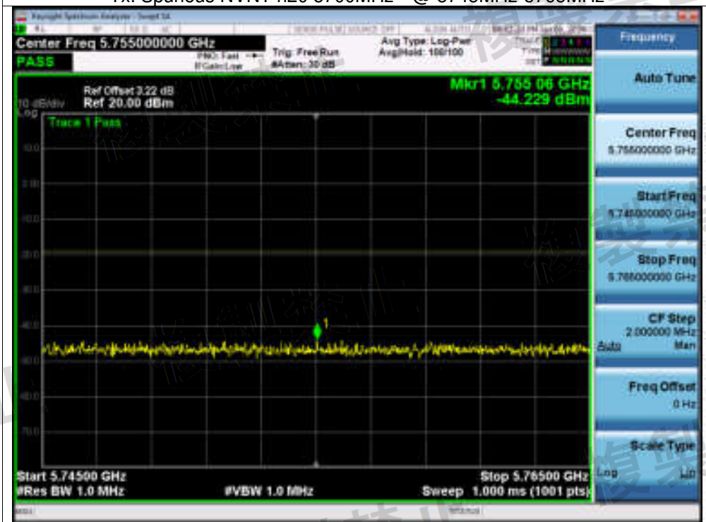
Tx. Spurious NVNT n20 5700MHz @ 5745MHz-5765MHz
