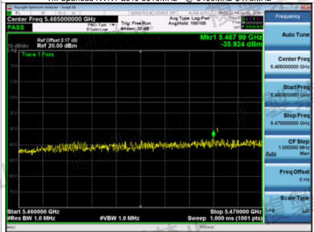
Tx. Spurious NVNT ac40 5510MHz @ 5460MHz-5470MHz
