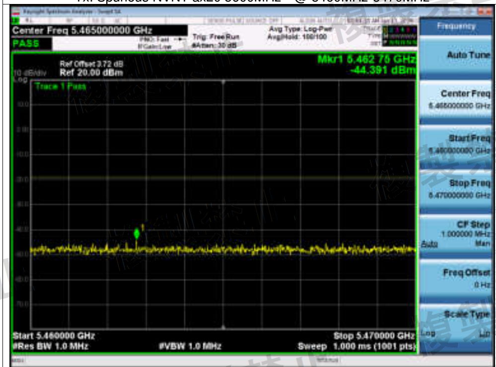
Tx. Spurious NVNT ax20 5600MHz @ 5460MHz-5470MHz
