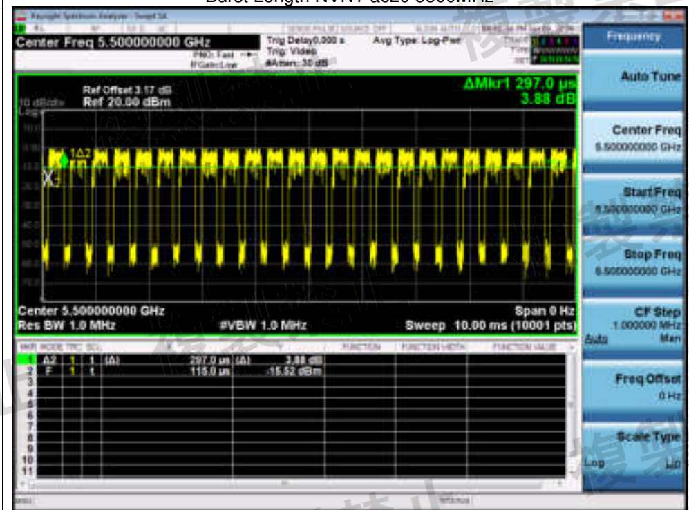
Burst Length NVNT ac20 5500MHz
