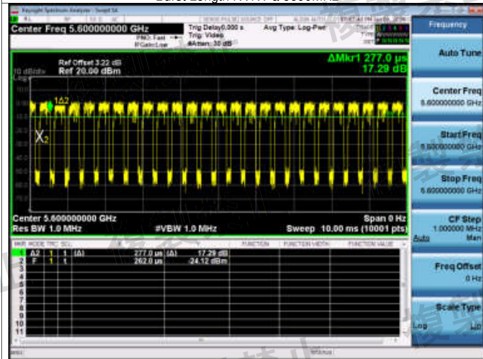
Burst Length NVNT a 5600MHz
