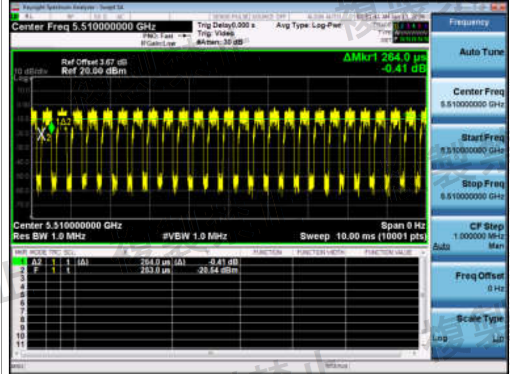
Burst Length NVNT ax40 5510MHz
