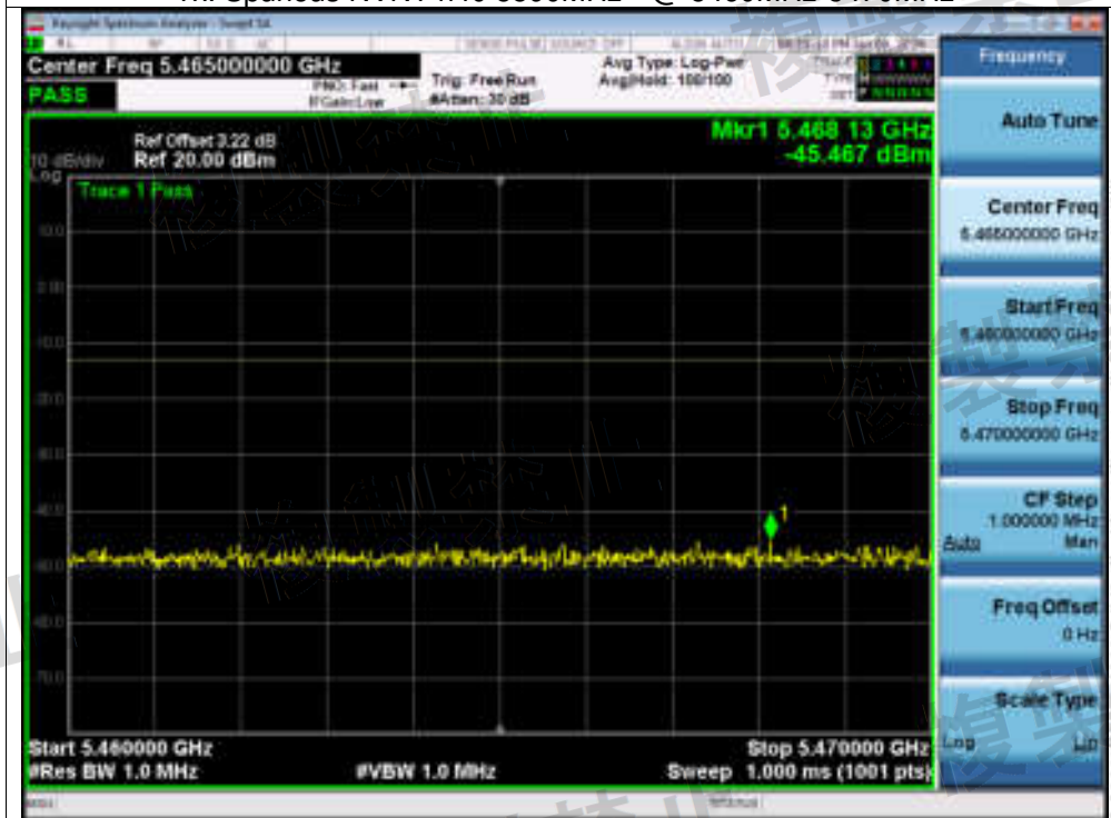
Tx. Spurious NVNT n40 5590MHz @ 5460MHz-5470MHz
