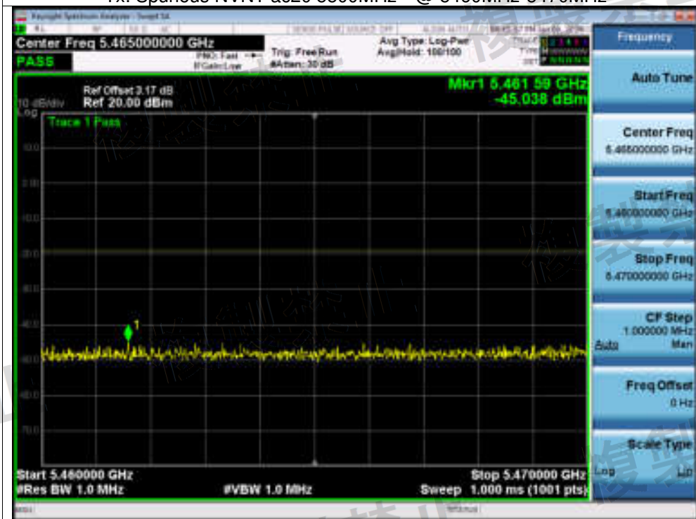
Tx. Spurious NVNT ac20 5500MHz @ 5460MHz-5470MHz
