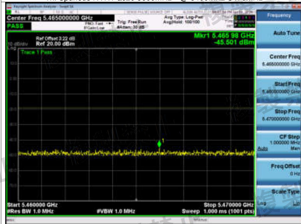
Tx. Spurious NVNT ac20 5600MHz @ 5460MHz-5470MHz
