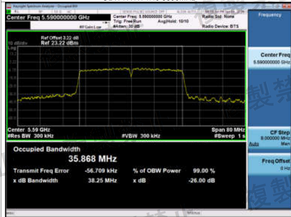
OBW NVNT n40 5590MHz
