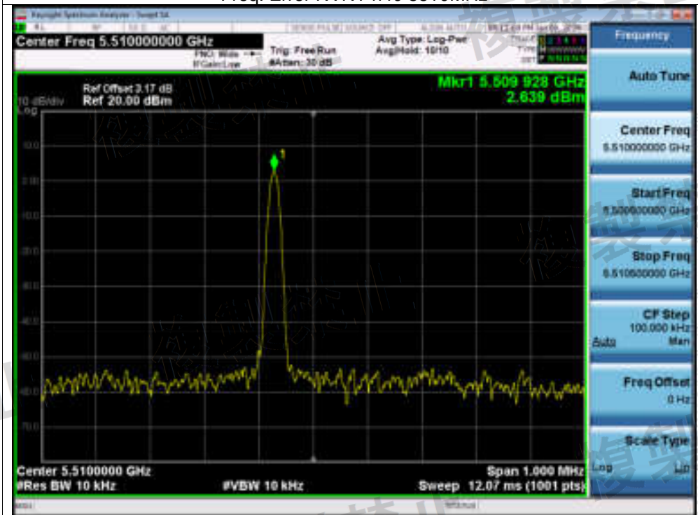
Freq. Error NVNT n40 5510MHz
