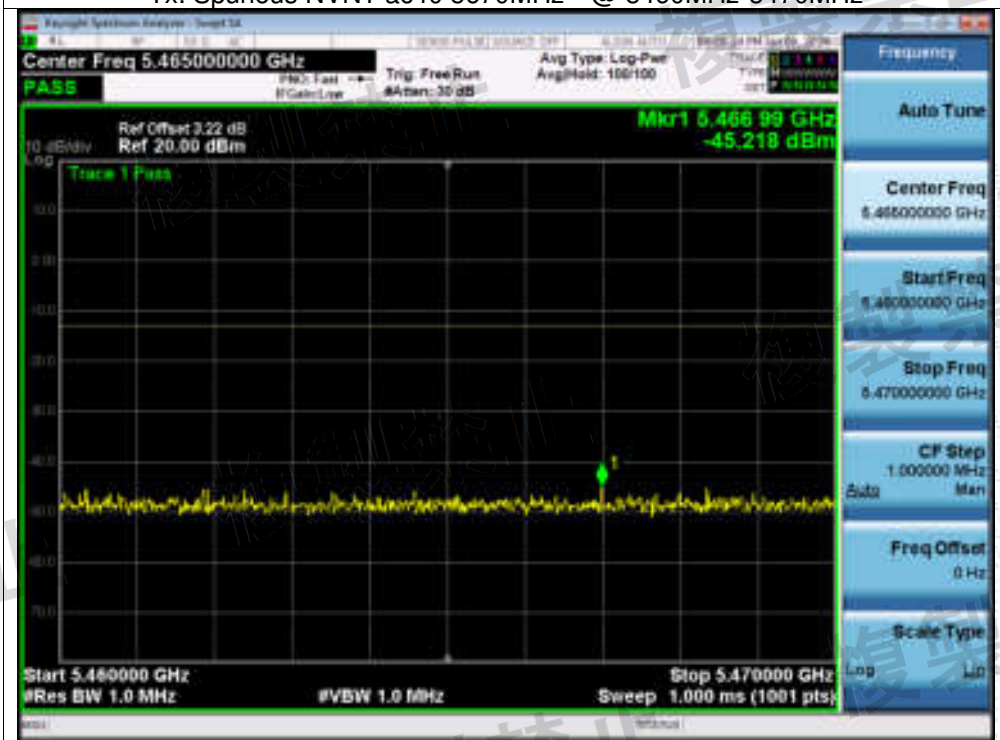
Tx. Spurious NVNT ac40 5670MHz @ 5460MHz-5470MHz
