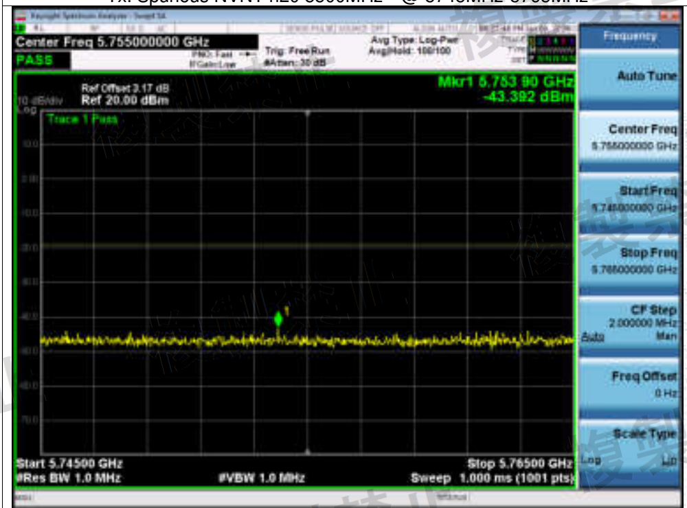
Tx. Spurious NVNT n20 5500MHz @ 5745MHz-5765MHz
