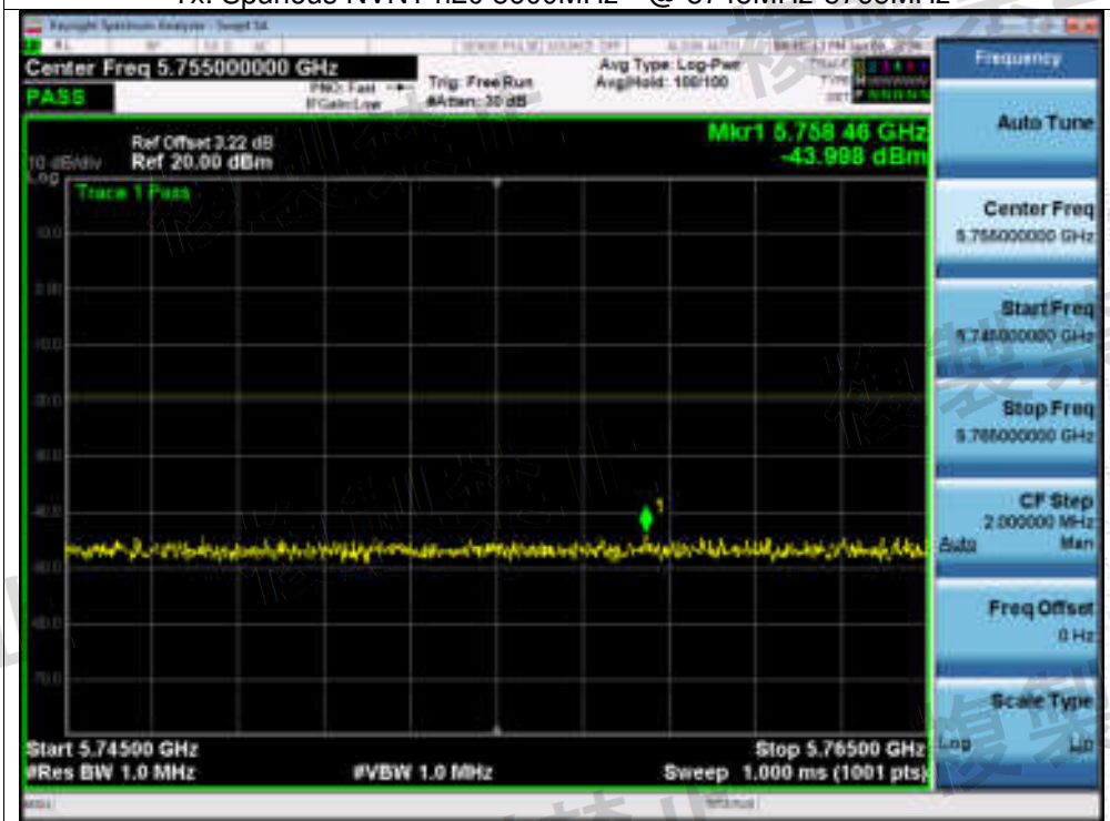
Tx. Spurious NVNT n20 5600MHz @ 5745MHz-5765MHz
