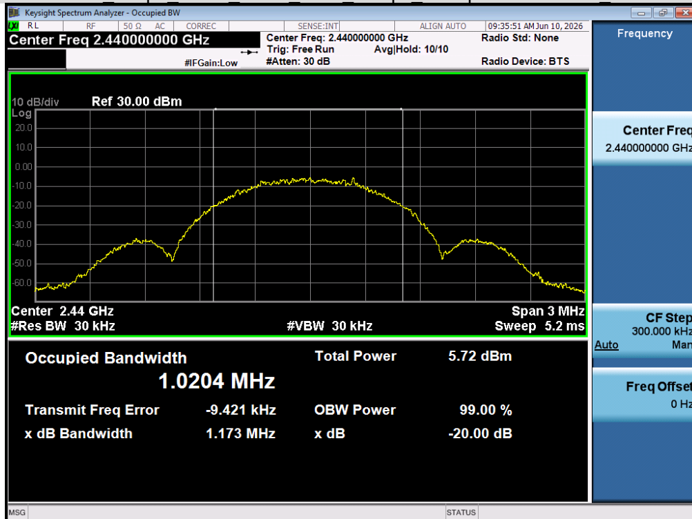
Test Graph LE1M ANT1 2440 1Mbps Occupied Bandwidth HV
