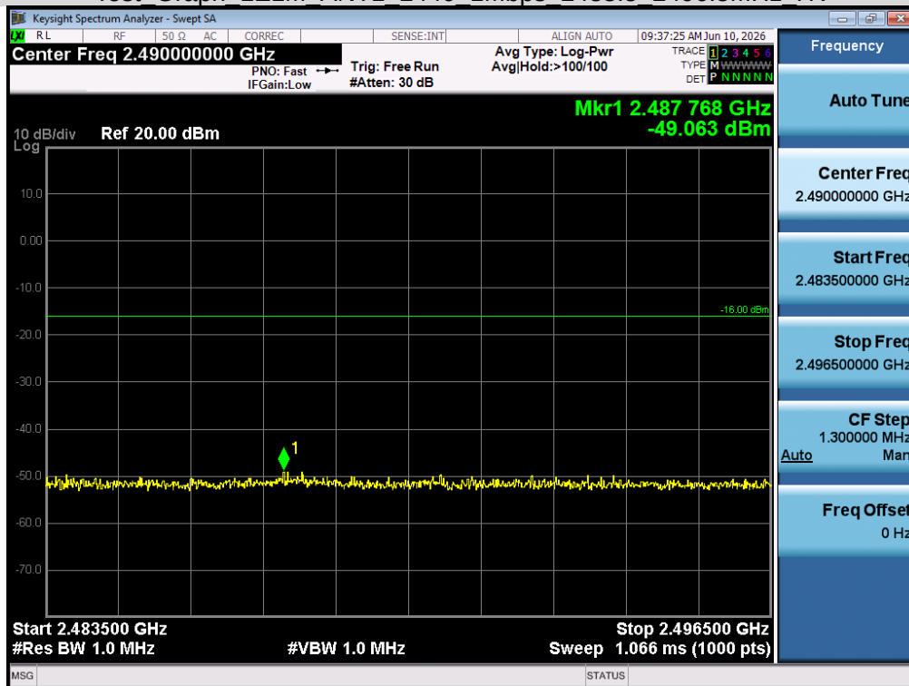
Test_Graph_LE1M_ANT1_2440_1Mbps_2483.5_2496.5MHz_LV
