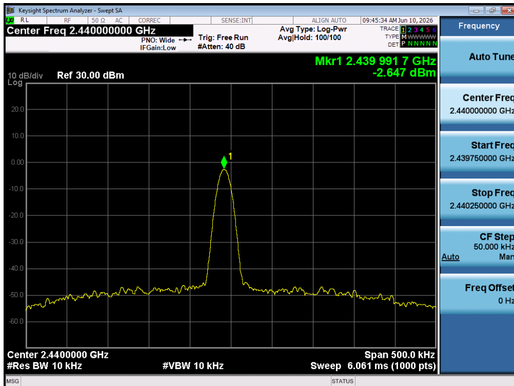
Test Graph Unmod ANT1 2440 NA Frequency Tolerance LV
