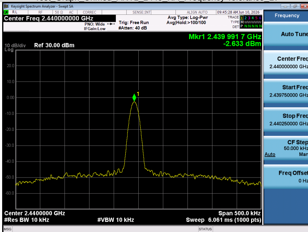
Test_Graph_Unmod_ANT1_2440_NA_Frequency Tolerance_NV
