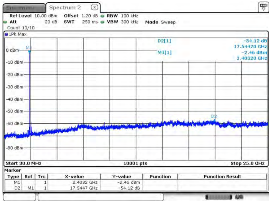
Channel 00 (30MHz-25GHz)-GFSK
