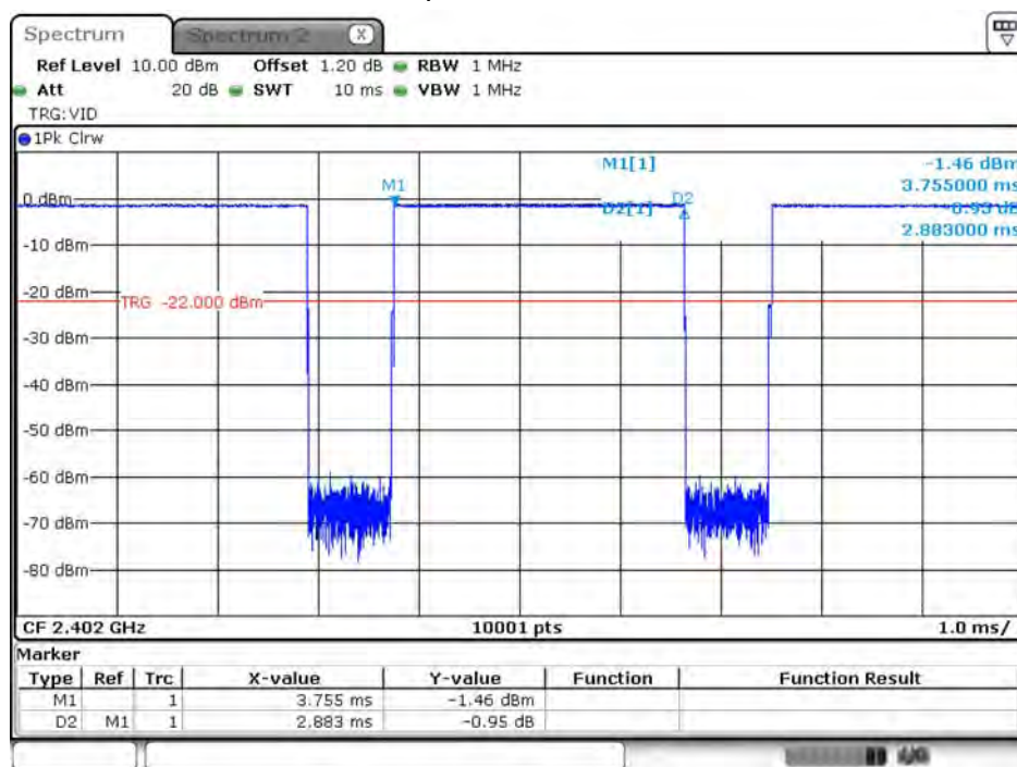
Hop rate-2402MHz
