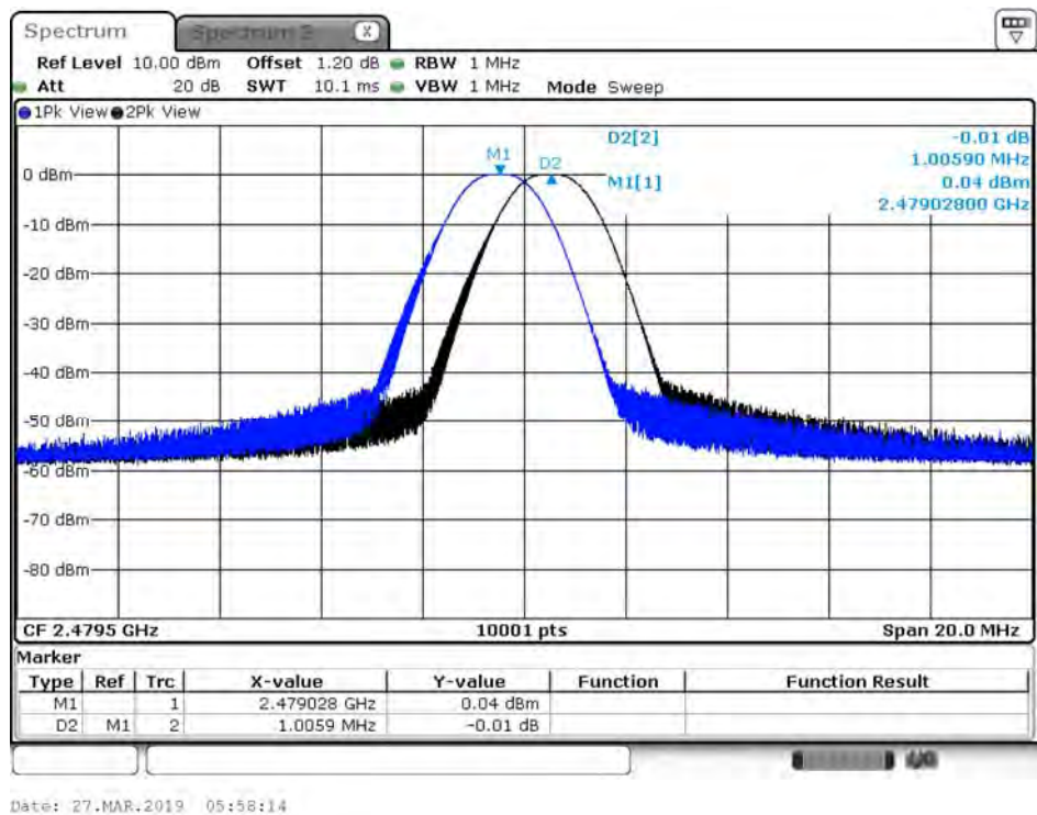
Channel 78
