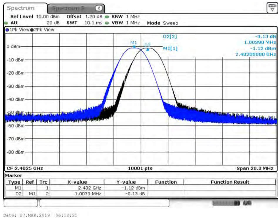
Channel 00
