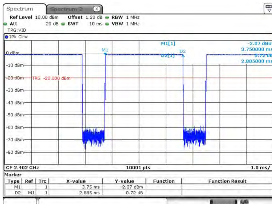
Hop rate-2402MHz
