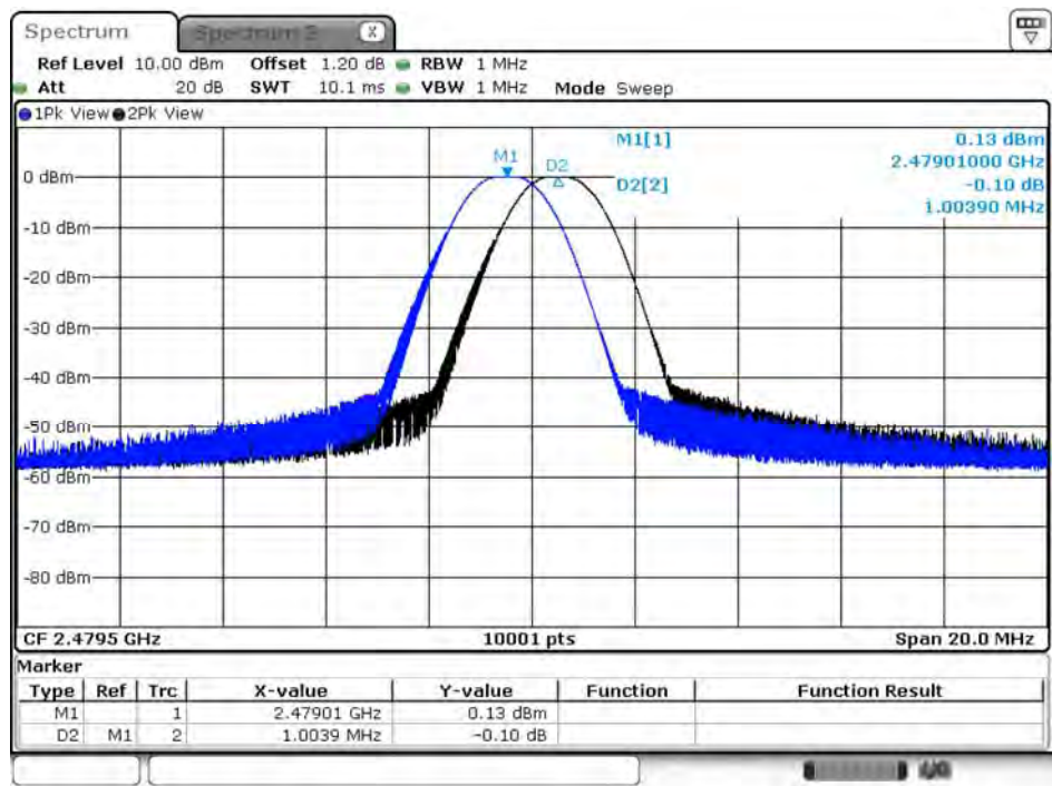
Channel 78
