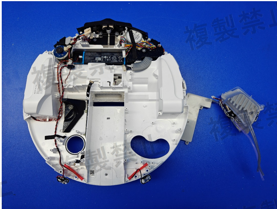
Figure 20. Internal view
