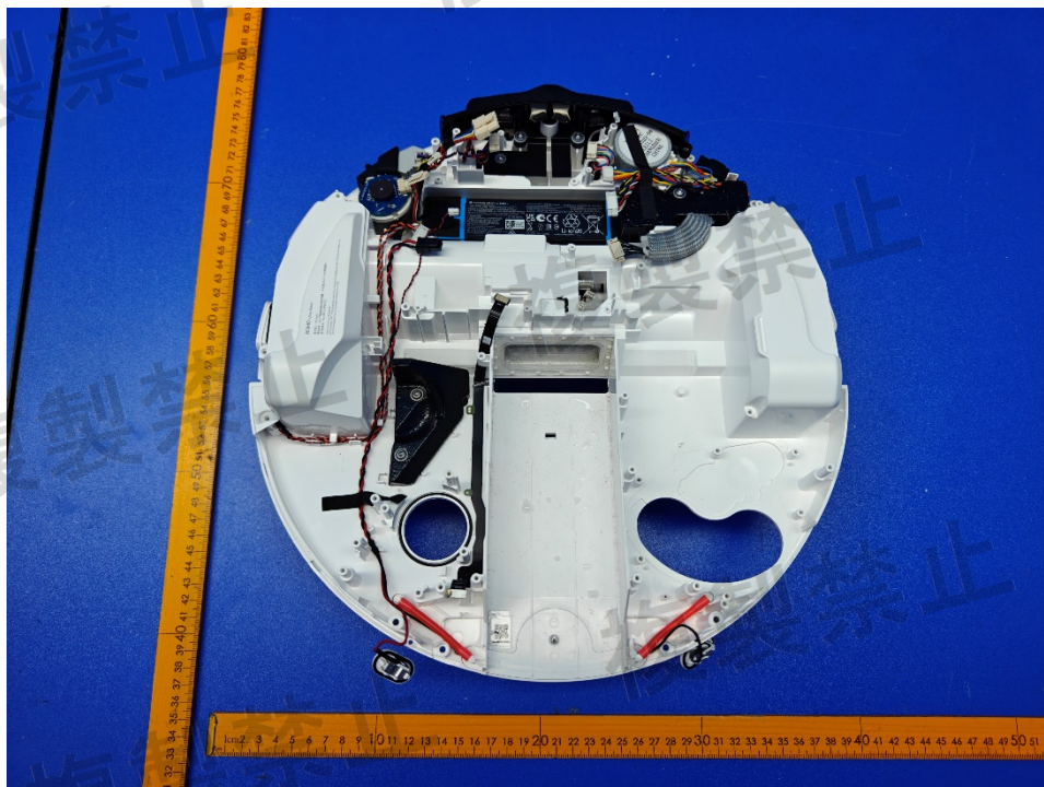
Figure 23. Internal view
