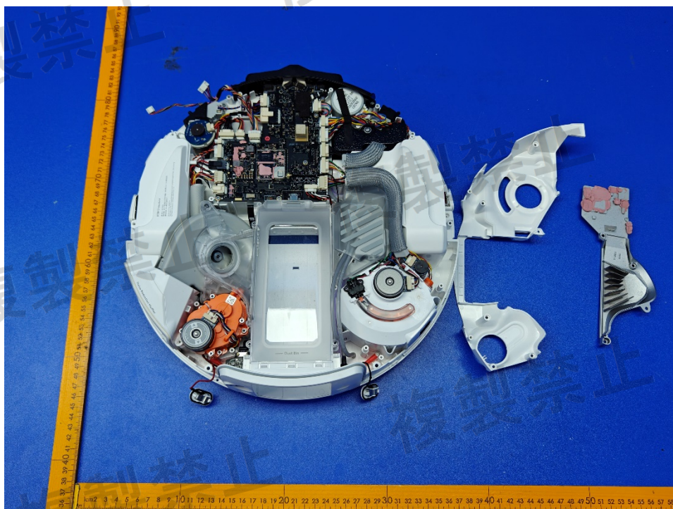
Figure 7. Internal view
