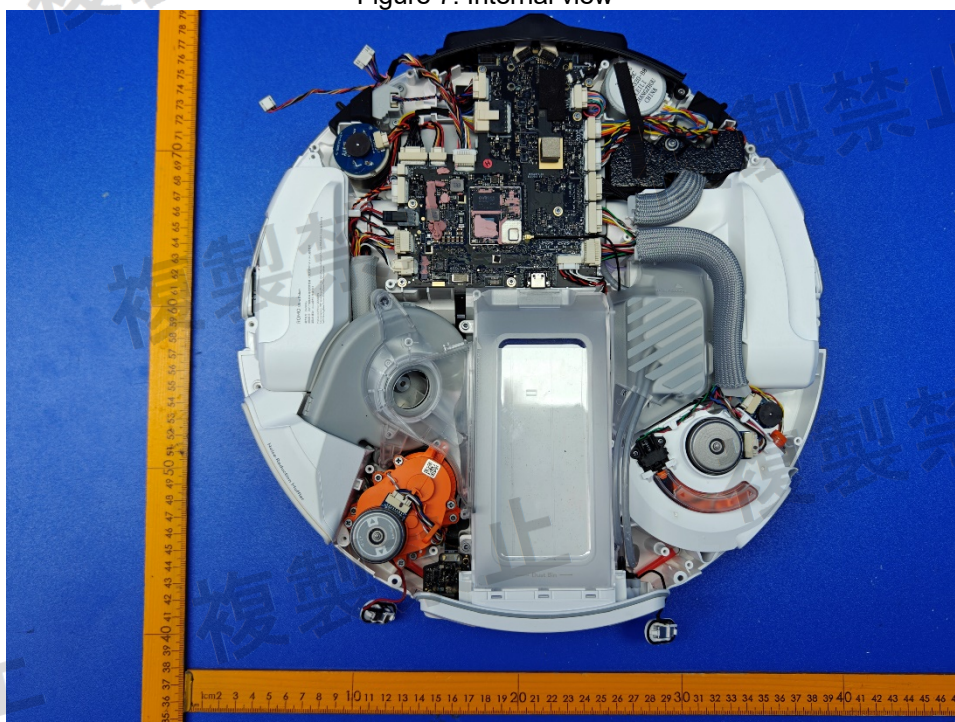
Figure 8. Internal view
