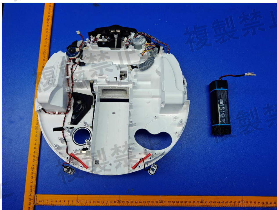
Figure 24. Battery pack view
