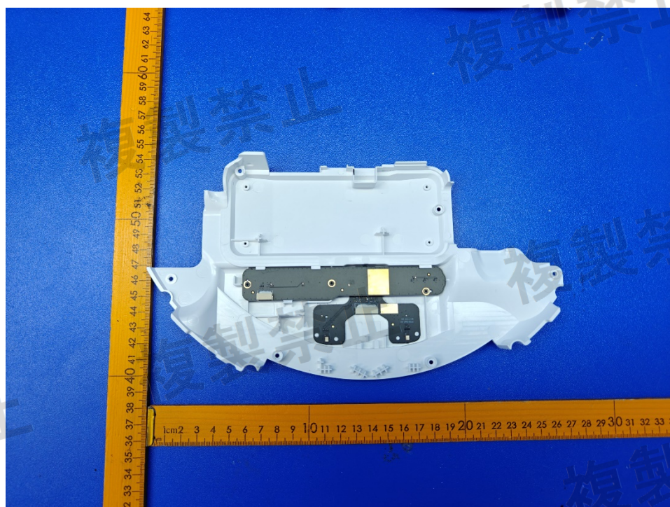
Figure 4. Control PCB cover
