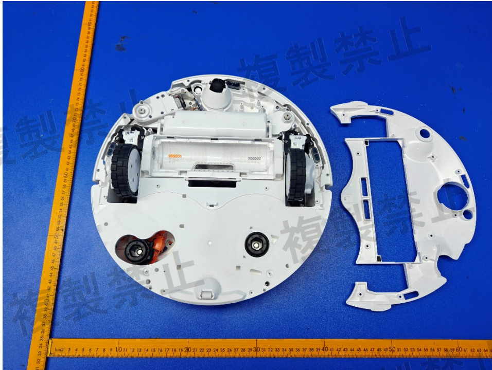
Figure 1. Internal view
