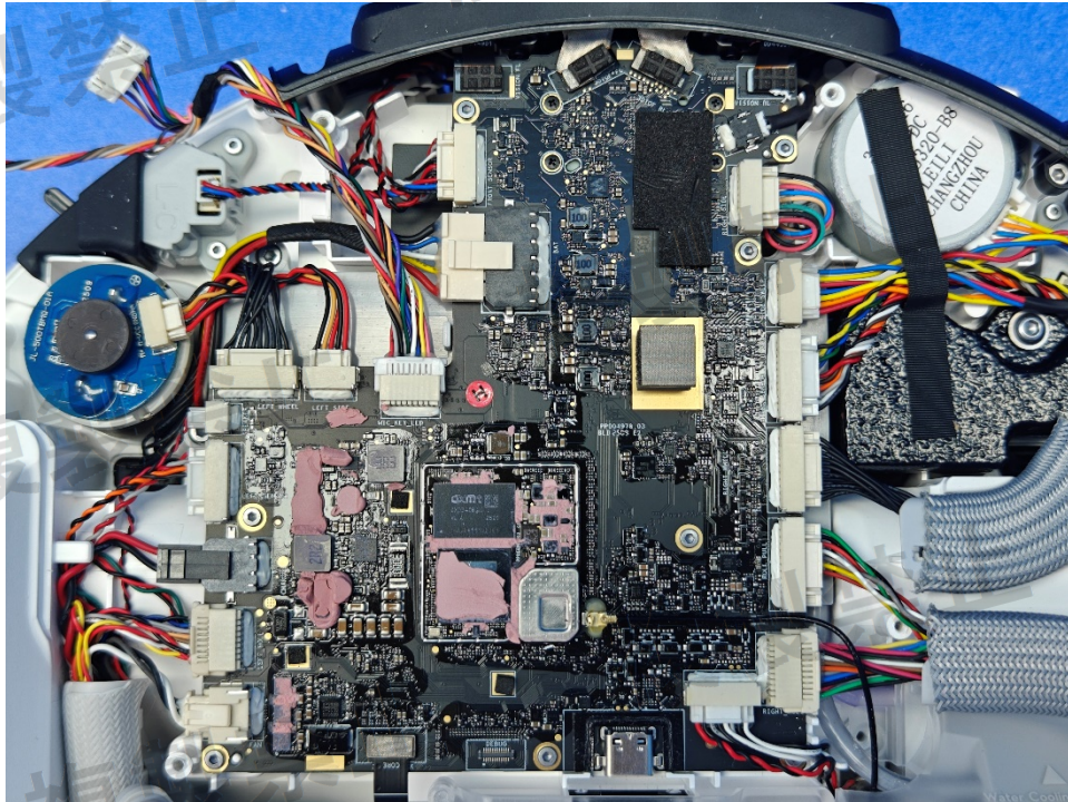
Figure 9. Internal view
