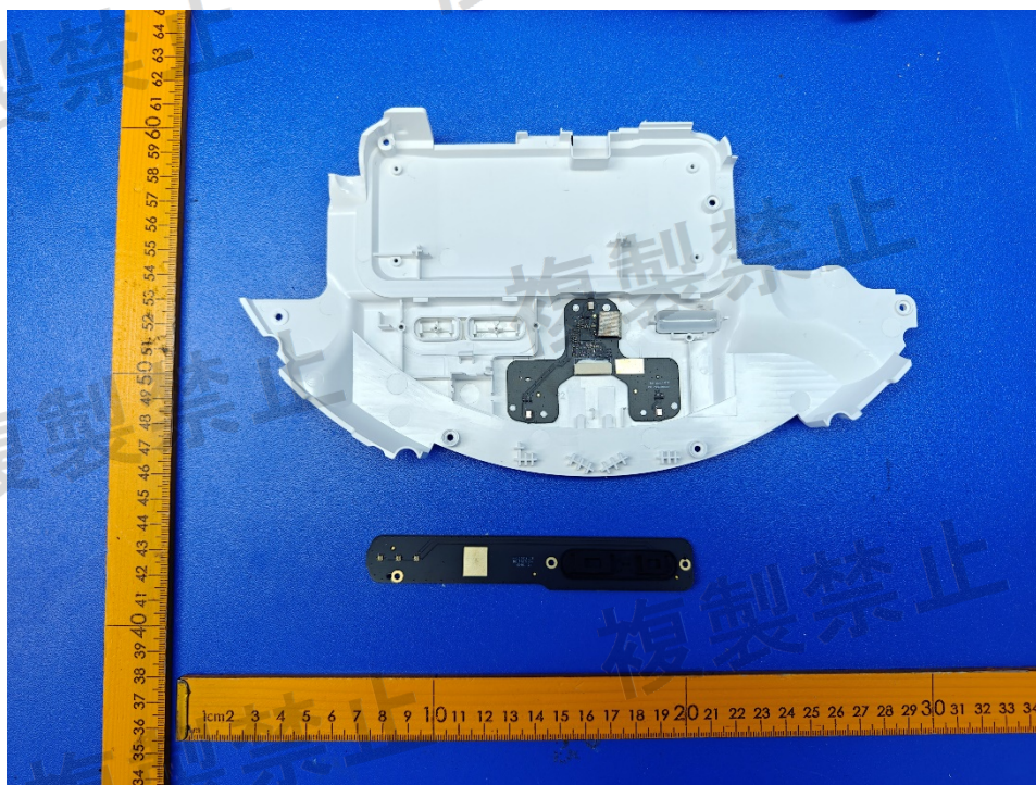
Figure 5. Control PCB
