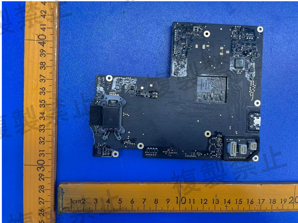
Figure 19. Main PCB
