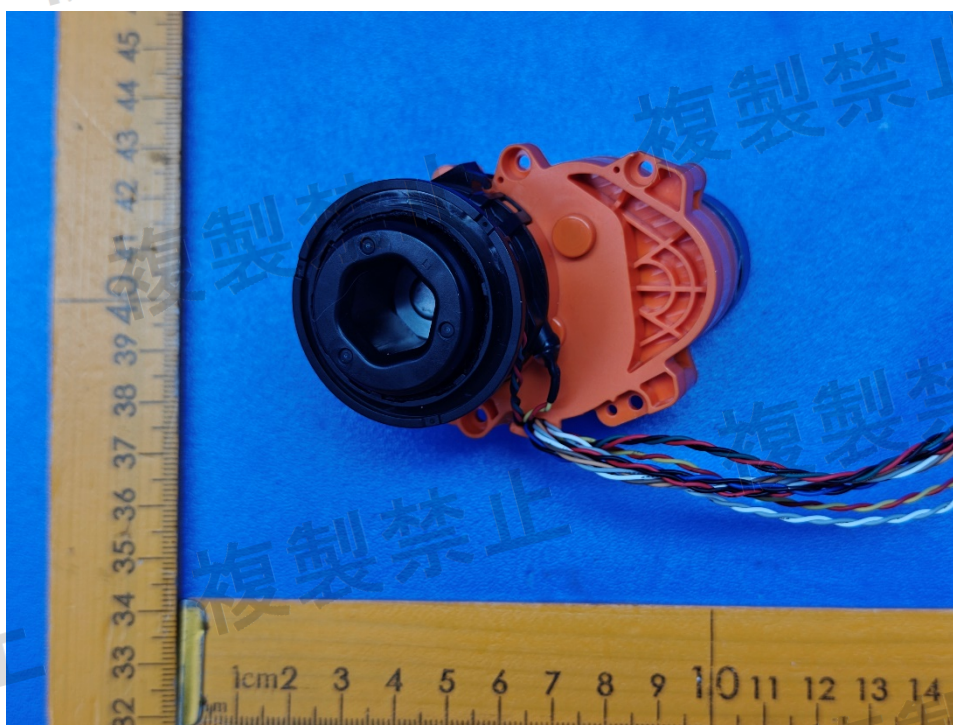
Figure 16. Mop motor
