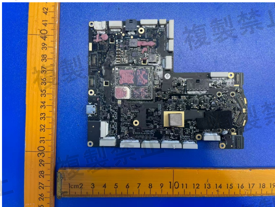
Figure 18. Main PCB
