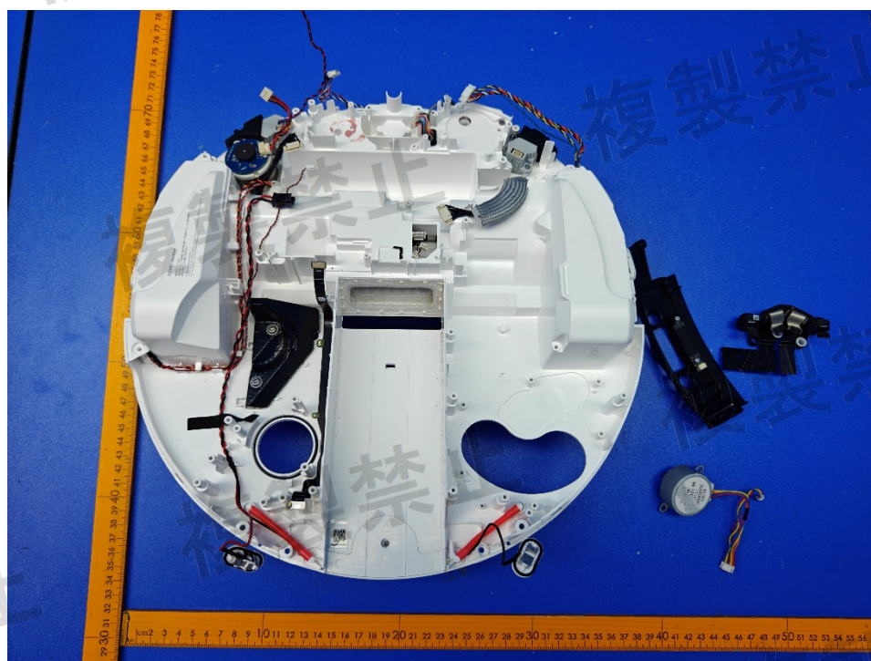
Figure 26. Internal view
