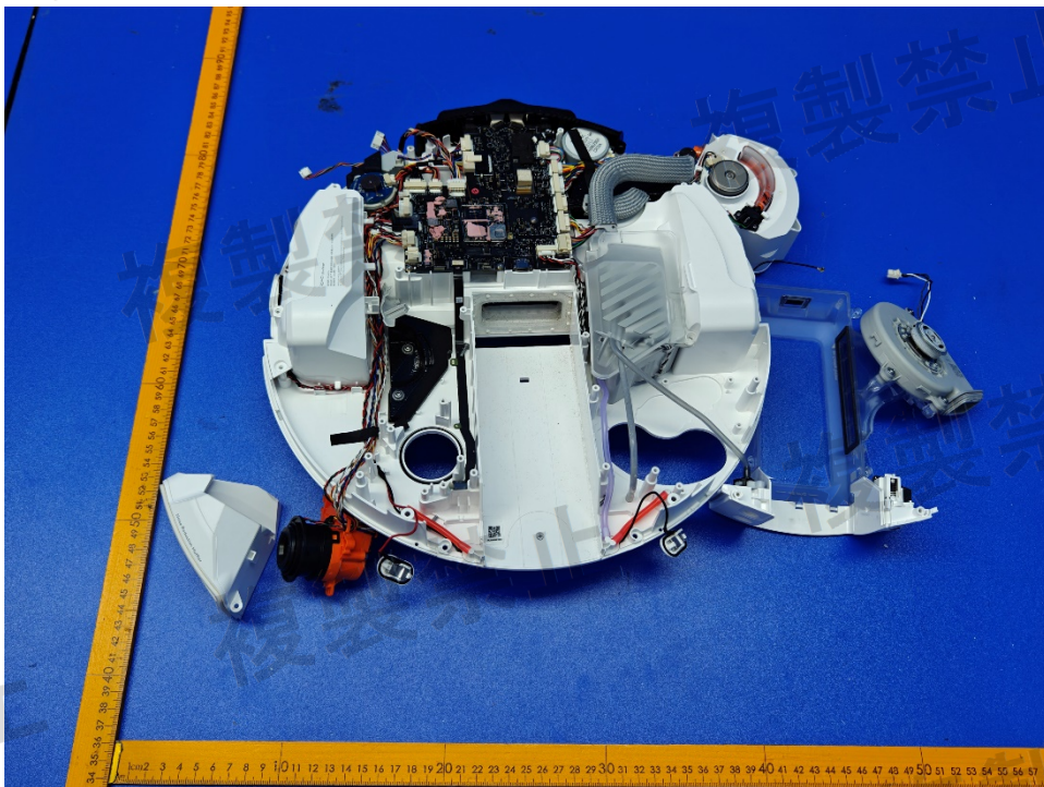
Figure 10. Internal view
